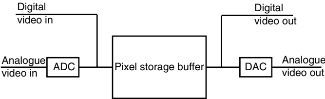
Figure 15-3 Dual-ported frame buffer.
