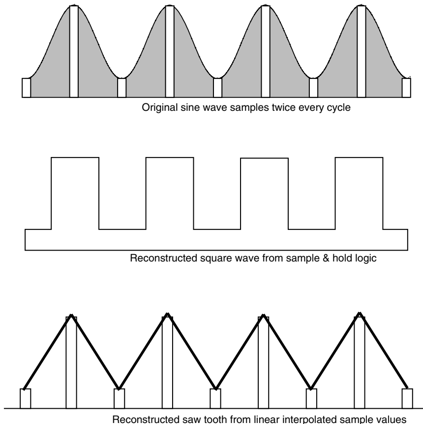
Figure 7-9 Waveform reconstruction from samples.
