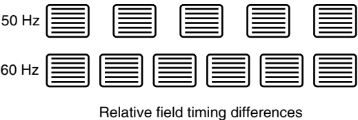
Figure 33-11 525i30 and 625i25 timing.
