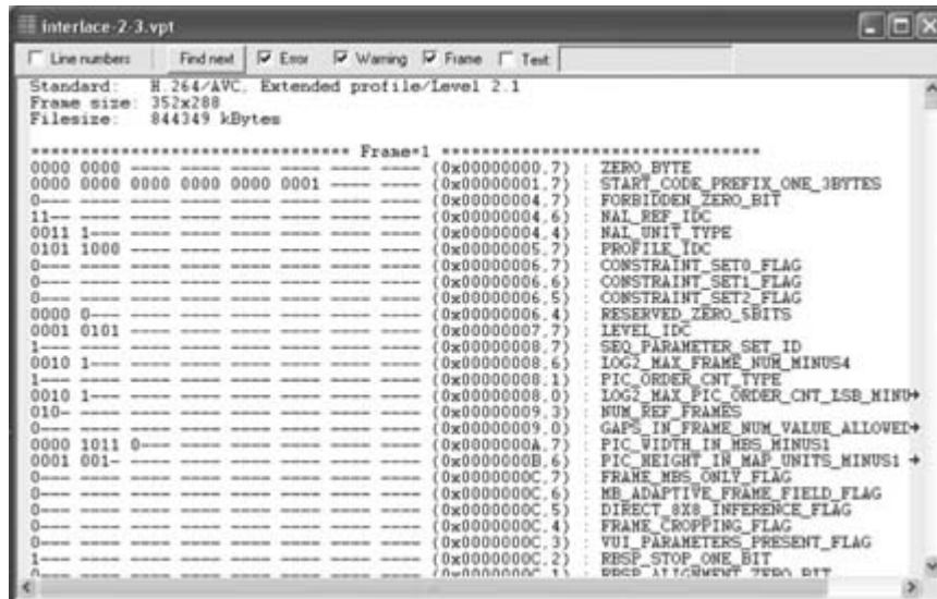
Figure 14-12 H.264 bit-stream output. Source: courtesy of Tektronix.
