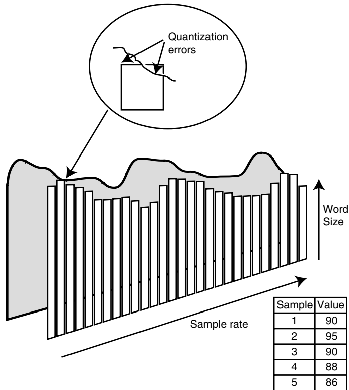
Figure 5-22 Digital waveform.
