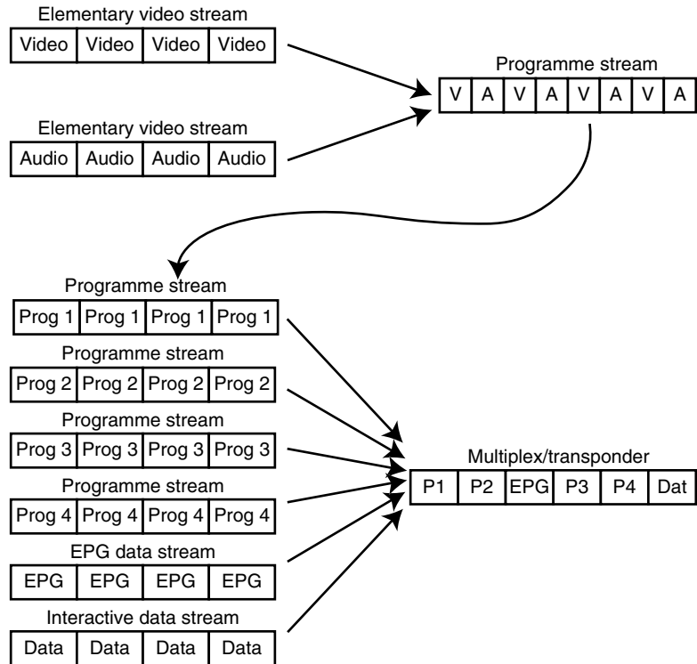
Figure 16-6 Stream structure.
