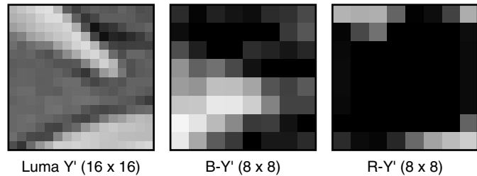
Figure 10-15 A picture of a macroblock.
