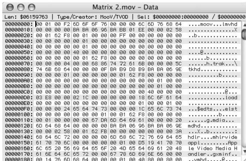
Figure 16-13 Screen shot from a hex dump application.
