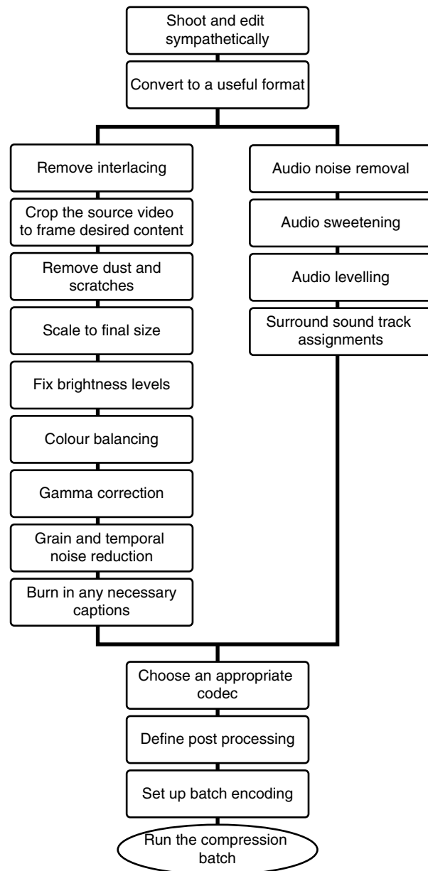
Figure 31-1 Compression workflow.
