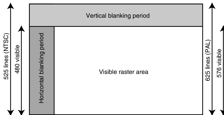
Figure 5-9 Physical and visible raster areas.
