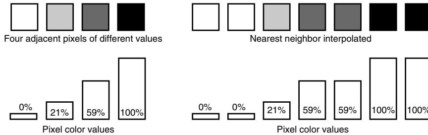
Figure 34-7 Nearest neighbor.
