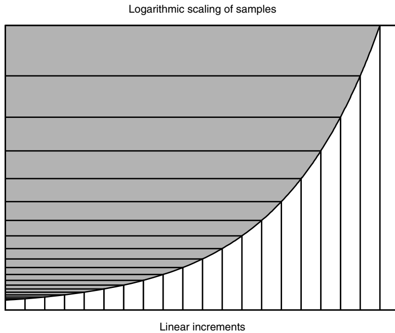
Figure 13-2 Logarithmic quantization.
