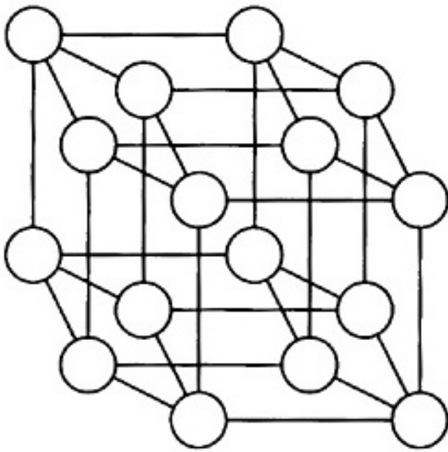
Figure 2.17 Hypercube Topology
