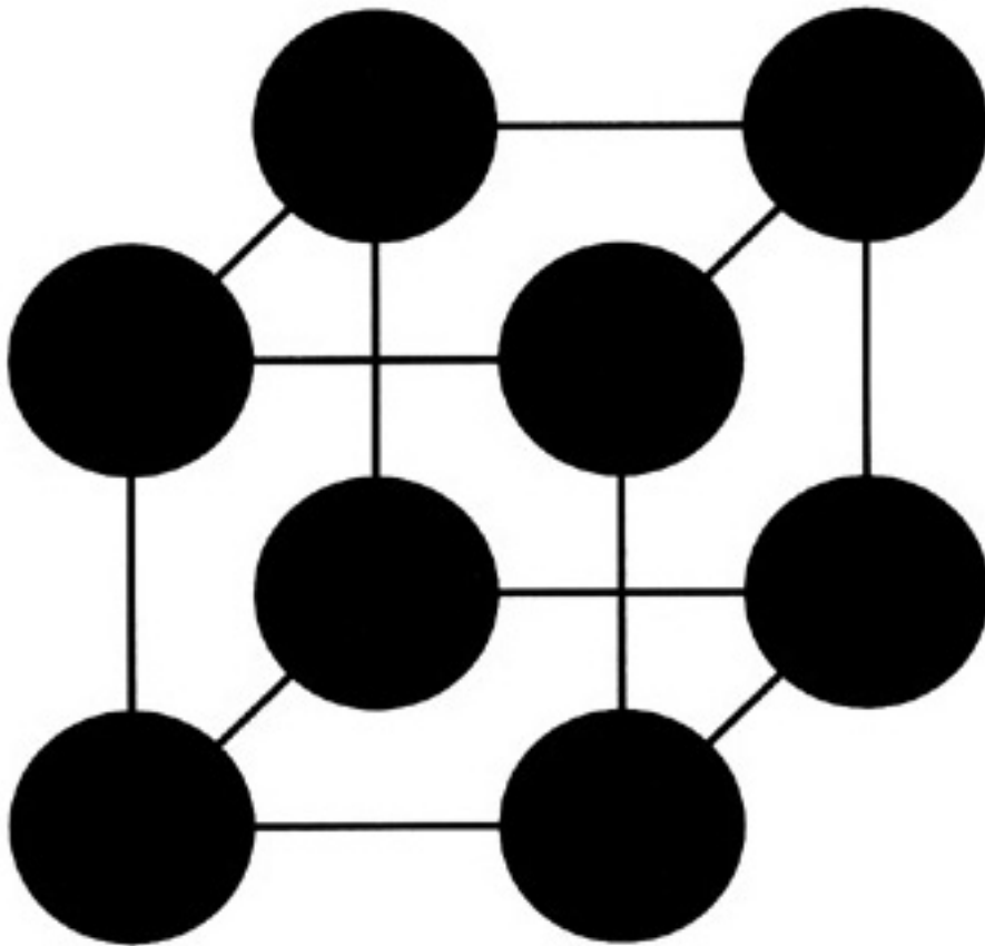
Figure 2.22 An 8-Node Hypercube
