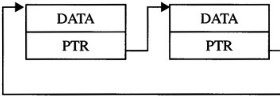
Figure 3.7 Circular List
