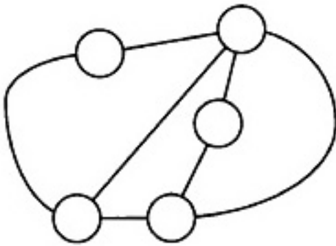
Figure 2.11 Planar Graph
