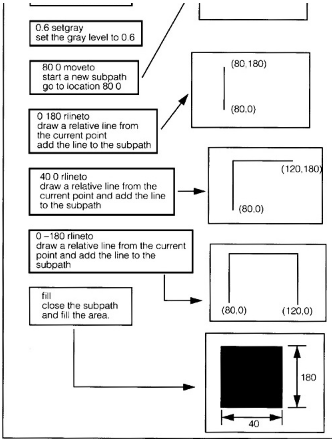
Figure 2.3 PostScript Rendering
