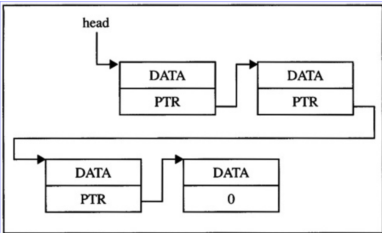
Figure 3.6 Linked List
