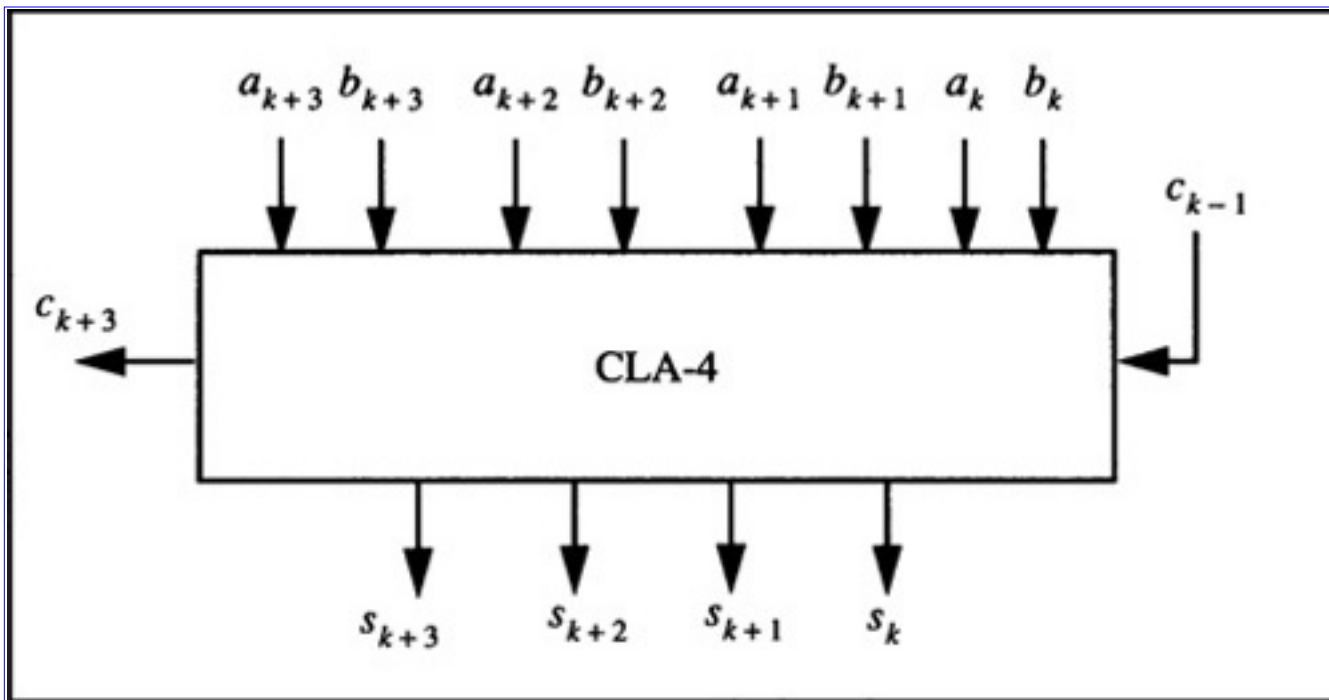
Figure 4.8 2's Complement 4-Bit Module Representation
