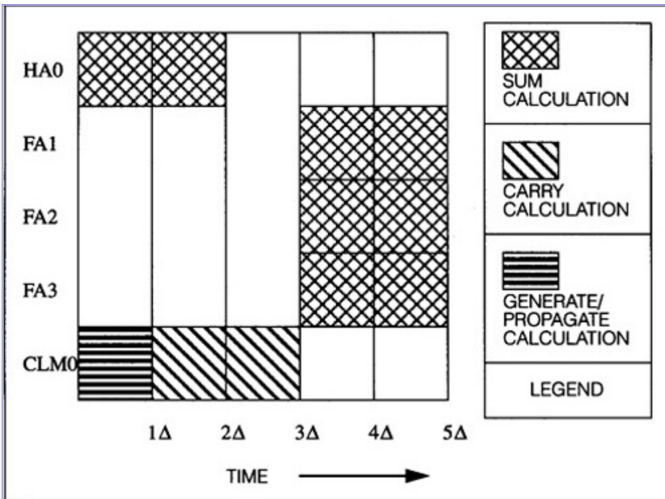
Figure 4.7 4-Bit CLA Adder Module Timing
