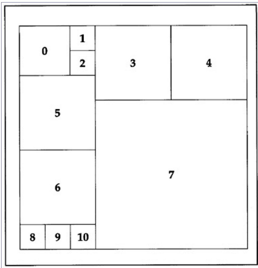
Figure 3.11 A Given Instance of the Square Packing Problem
