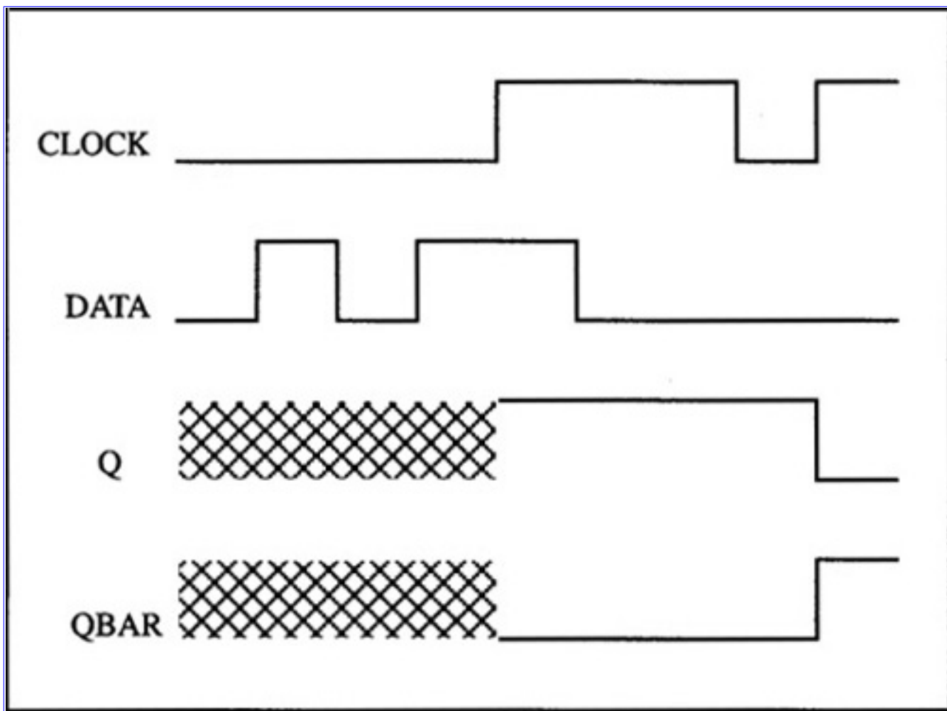
Figure 4.13 Timing Diagram for Simulation
