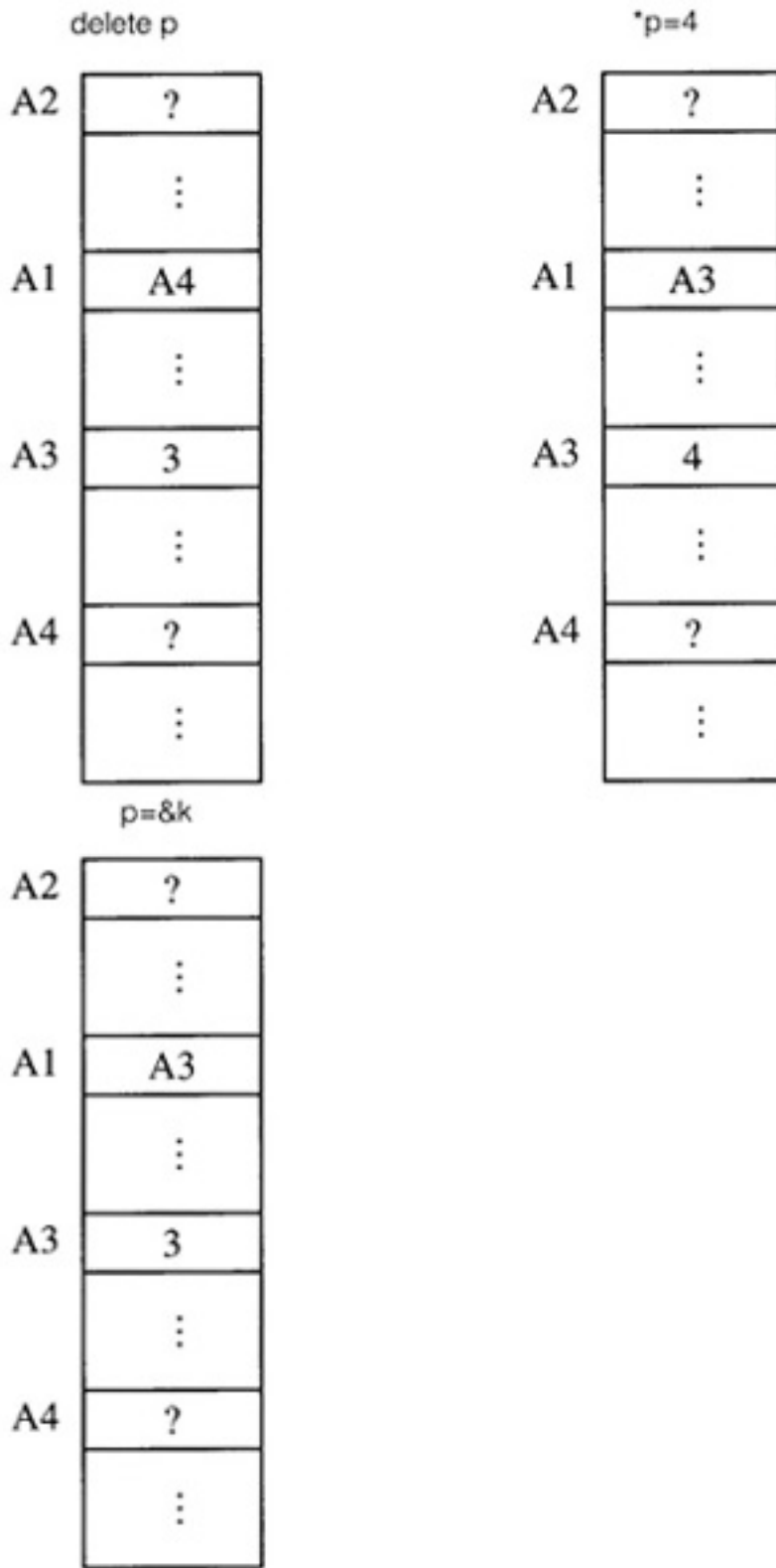
Figure 3.1 Memory Layout for C++ Program
