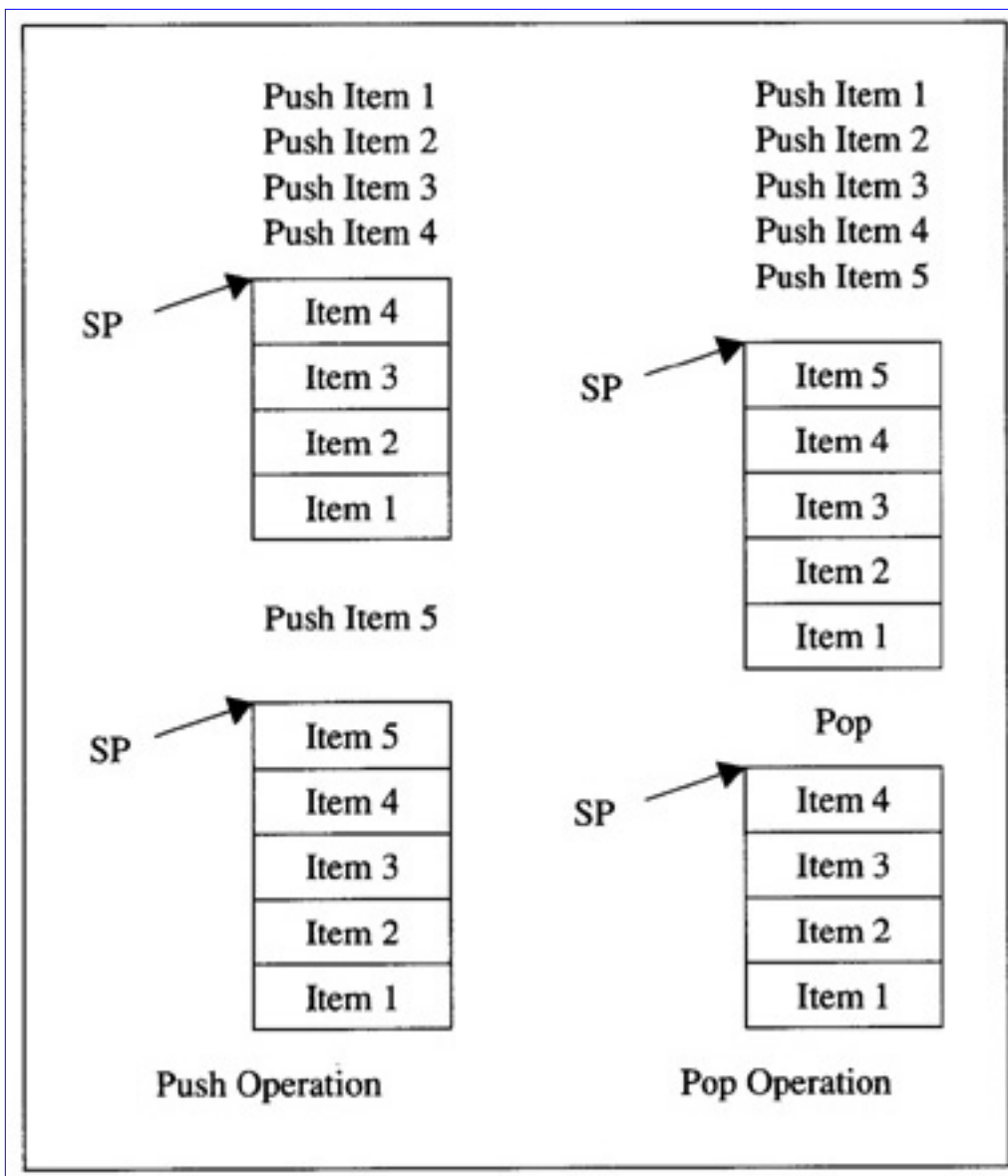
Figure 3.5 Push and Pop in a LIFO Stack
