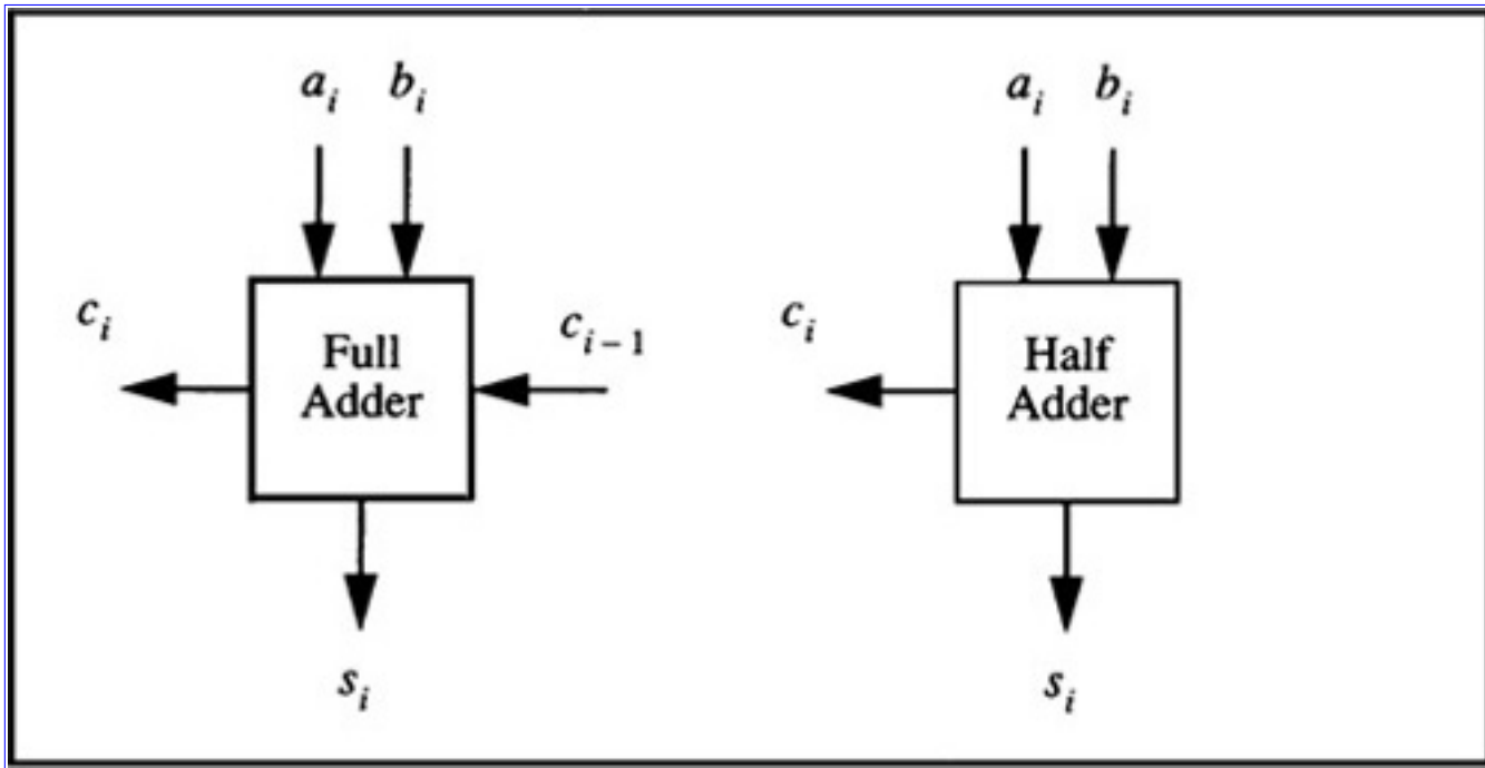
Figure 4.1 Full and Half Adder Modules
