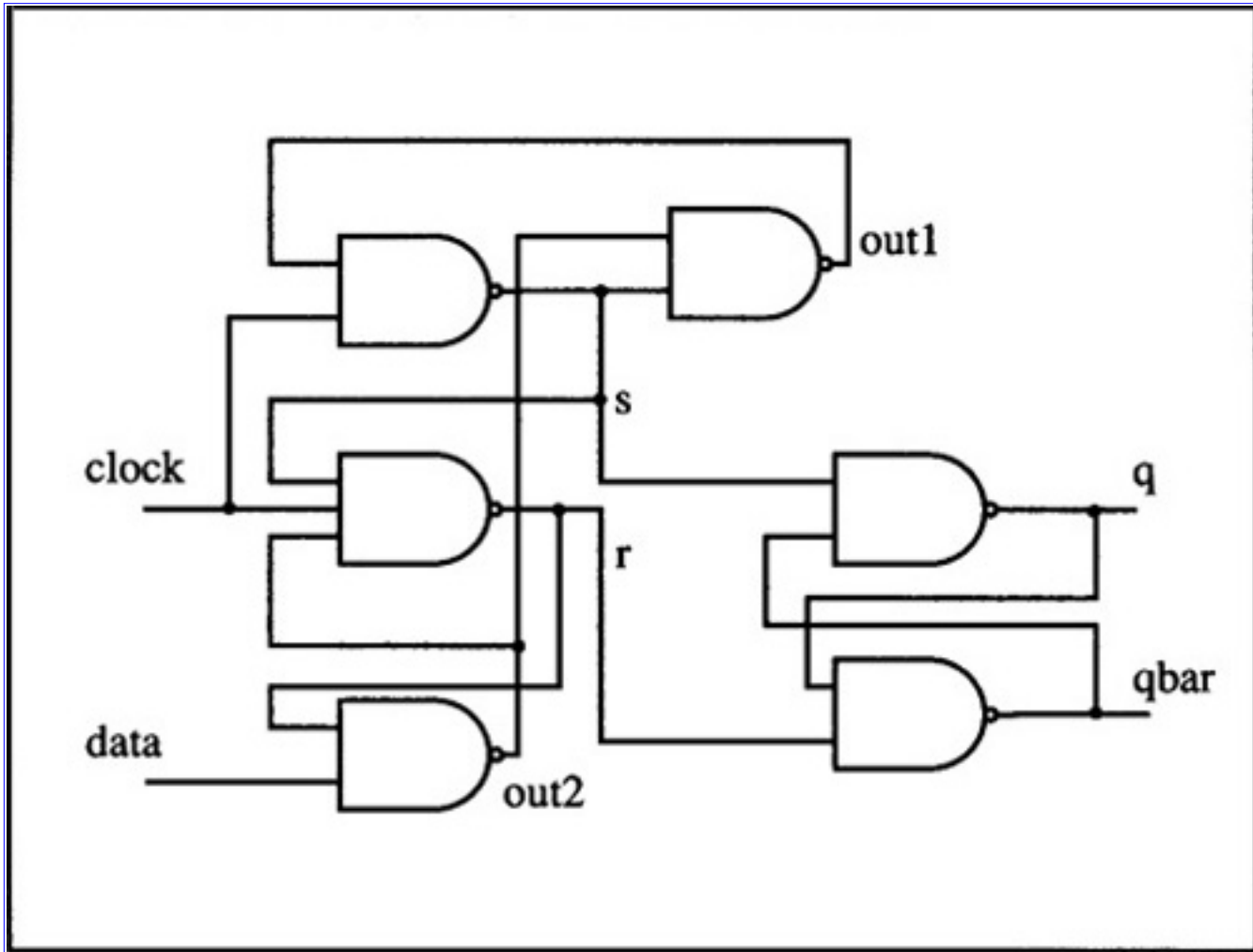
Figure 4.11 D Flip-Flop Circuit for Simulation
