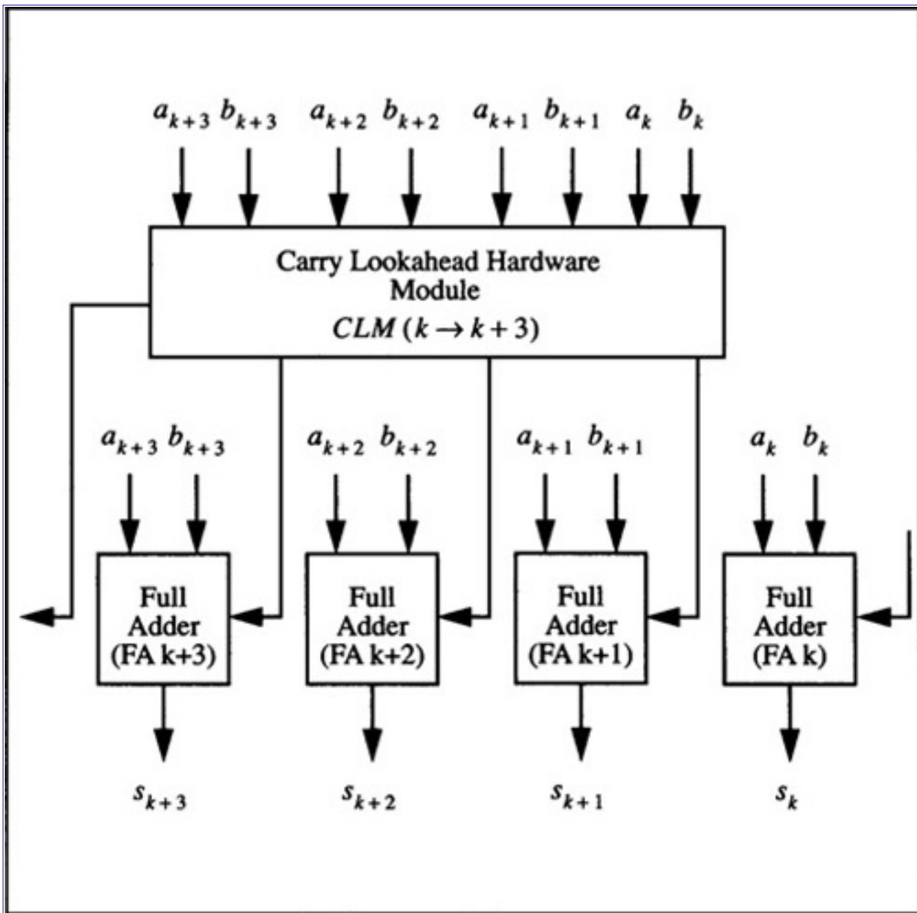
Figure 4.9 2's Complement 4-Bit CLA Adder Module
