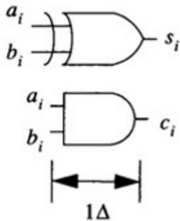
Figure 4.4 Output Delay Calculation for a Half Adder
