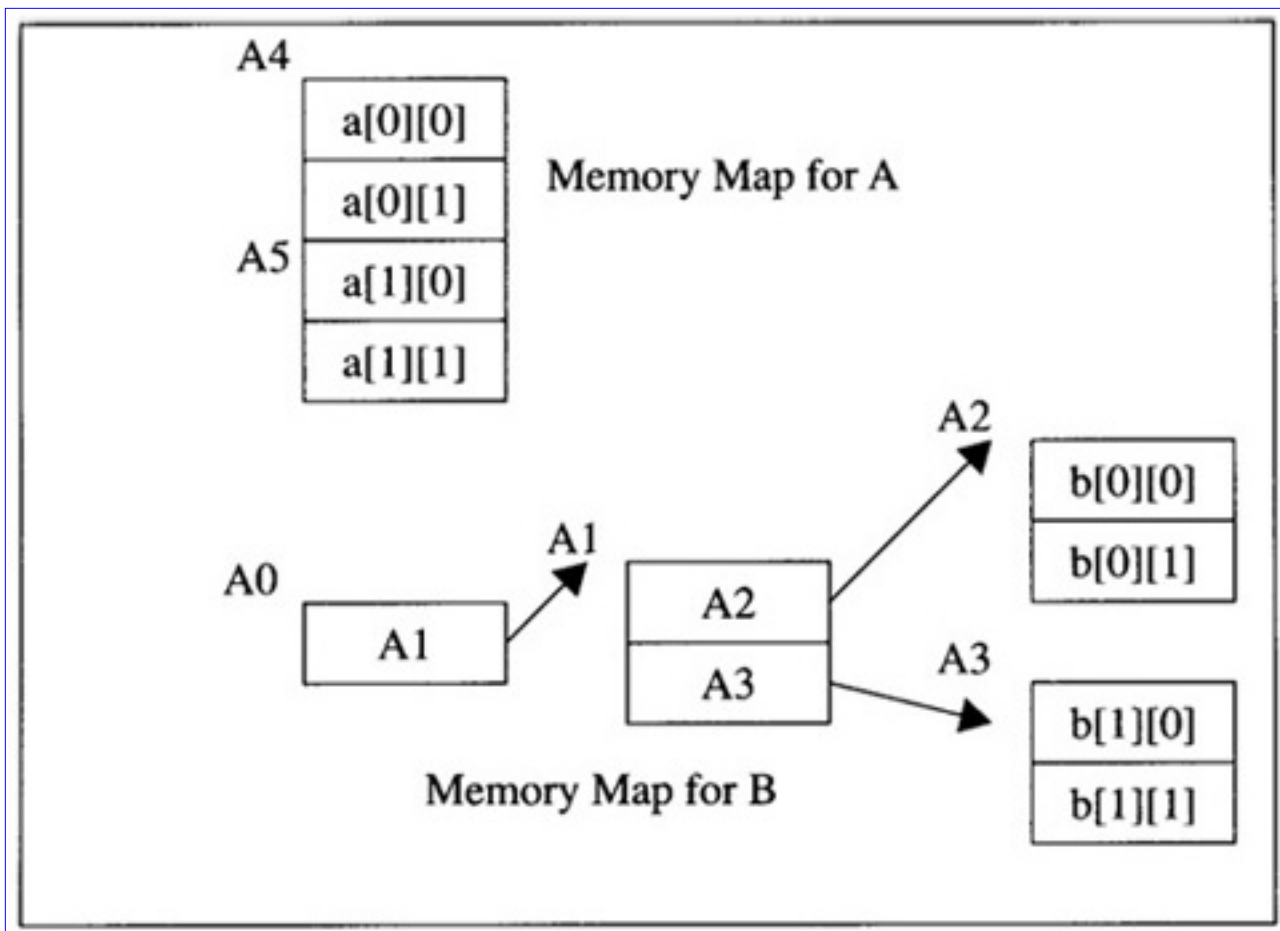
Figure 3.3 Memory Organization for Code List 3.8
