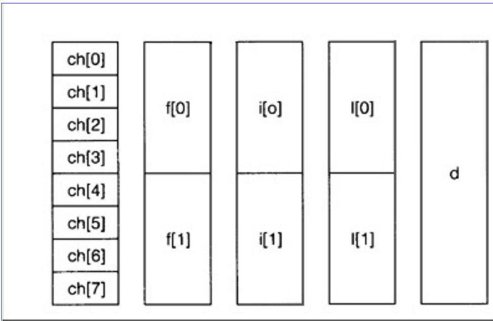
Figure 1.3 Mapping of each Union Entry
