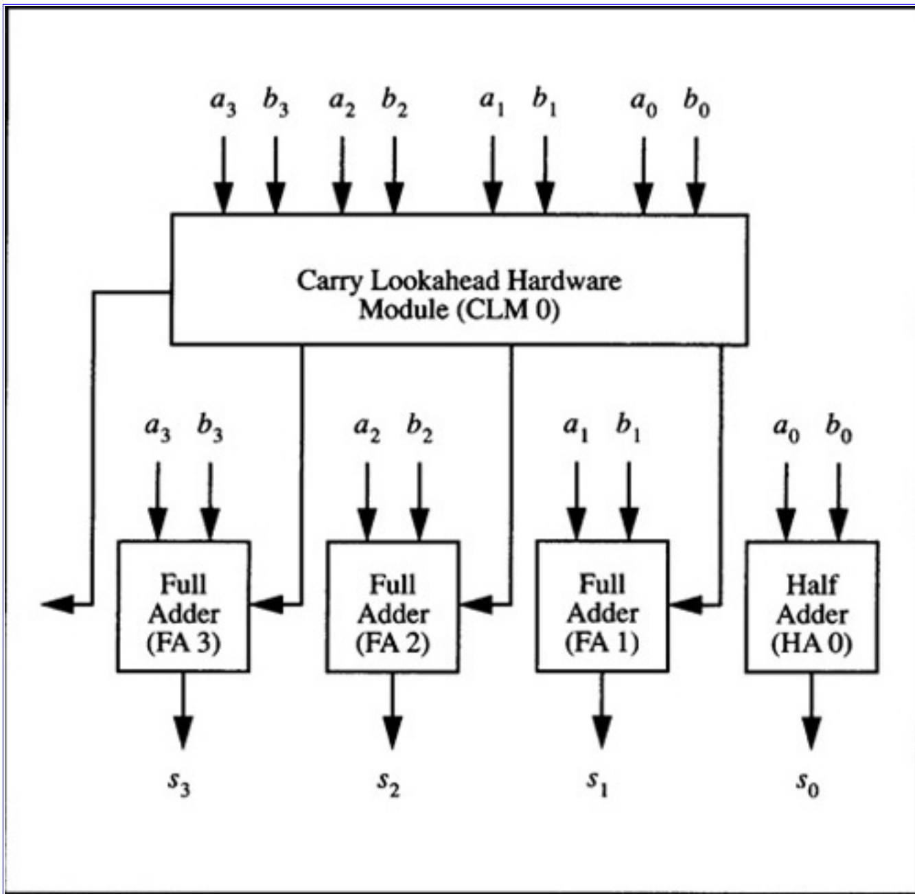
Figure 4.6 2's Complement 4-Bit CLA Adder Module
