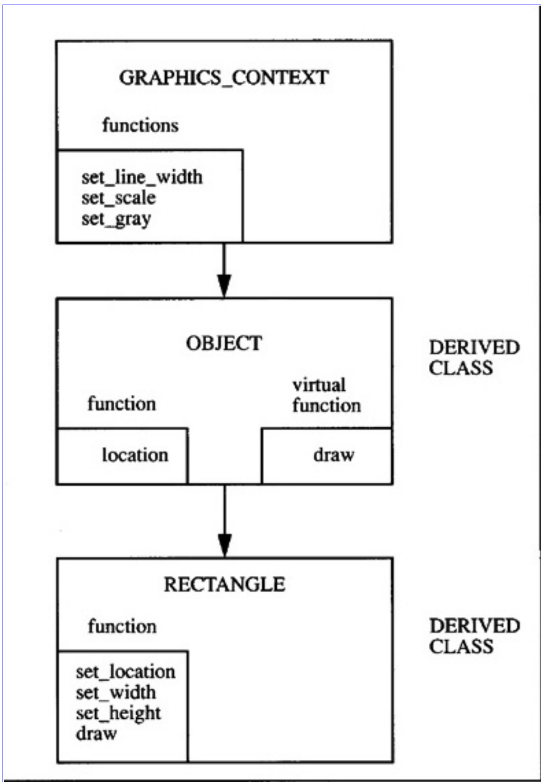
Figure 2.2 Class Structure
