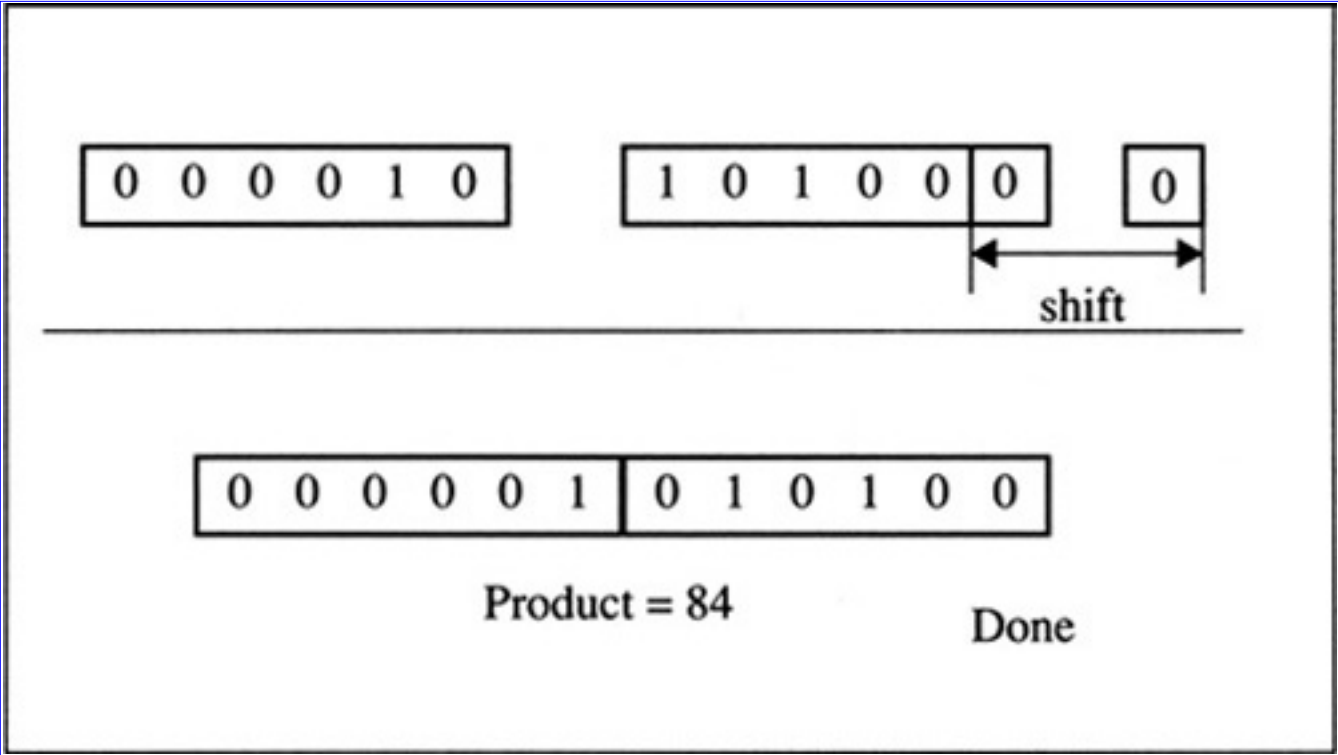
Figure 4.14 Booth Algorithm
