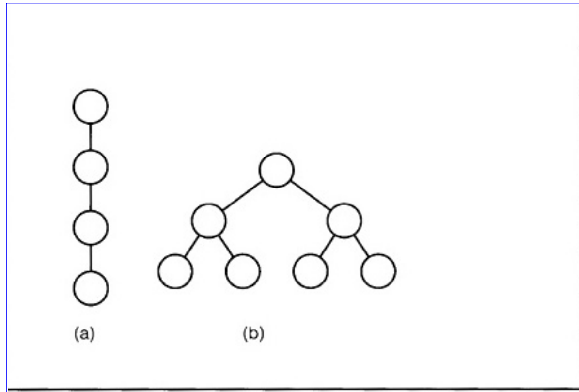
Figure 2.10 Trees
