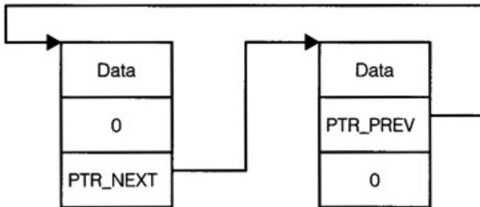
Figure 3.8 Doubly Linked List
