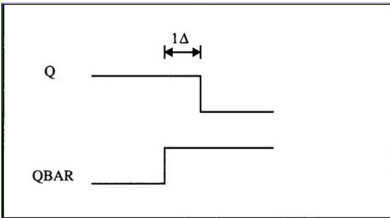
Figure 4.12 Transition Timing
