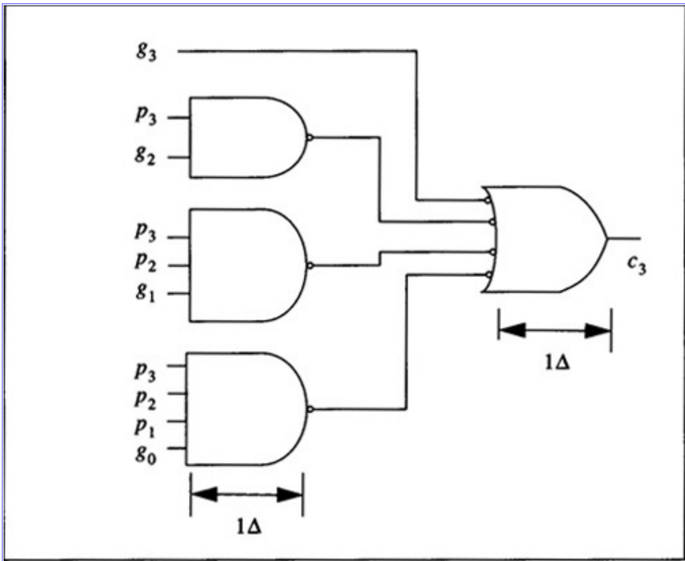
Figure 4.5 Delay Calculation
