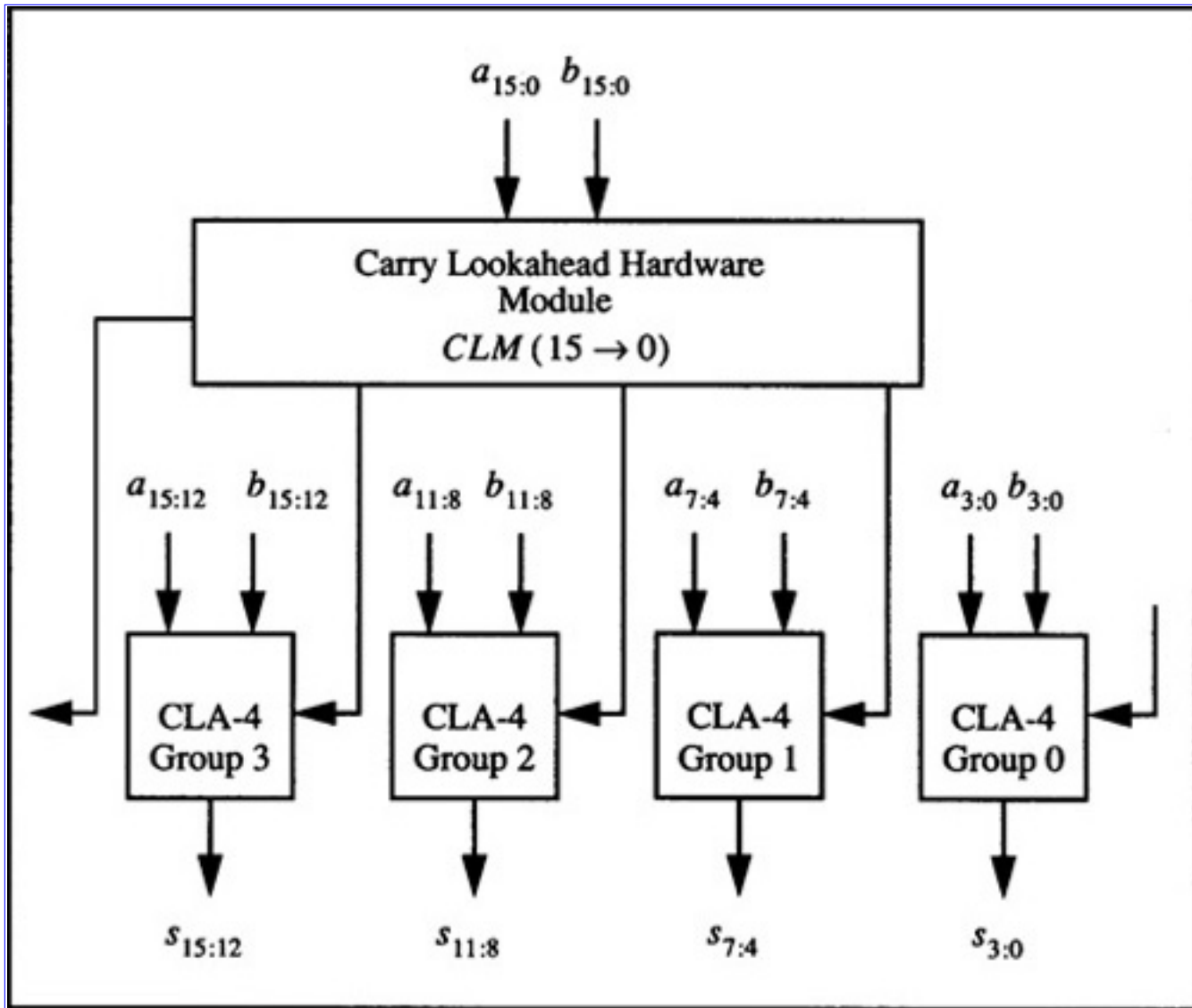
Figure 4.10 16-Bit CLA Adder with Group Lookahead
