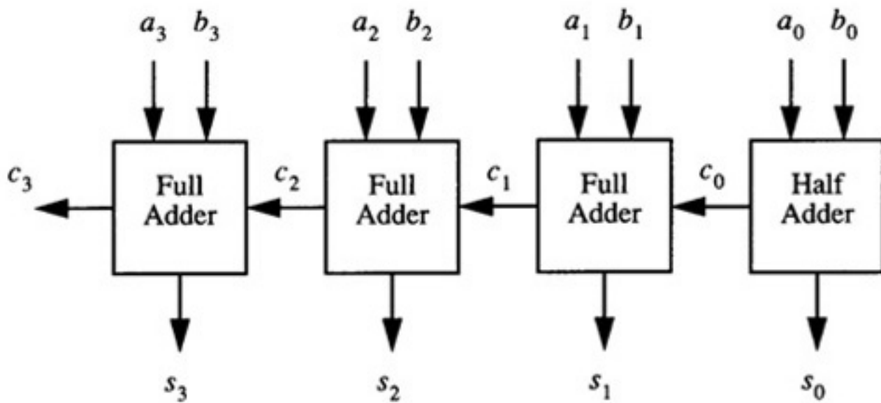
Figure 4.3 2's Complement 4-Bit Adder
