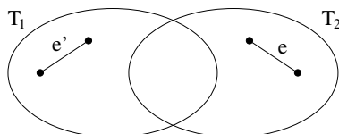
Fig. 2.1 Exchange lemma.
