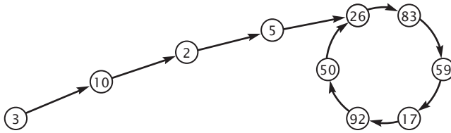
Figure 9.10 Tail and cycle iterating f(x) = x^2 + 1 \bmod 99 from x_0 = 3
