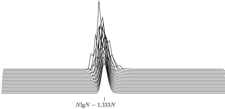
Figure 8.11 Distributions for path length in tries, even N from 10 to 50 (scaled and translated to center and separate curves)
