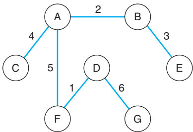
■ FIGURE 6.6G A minimum spanning tree
