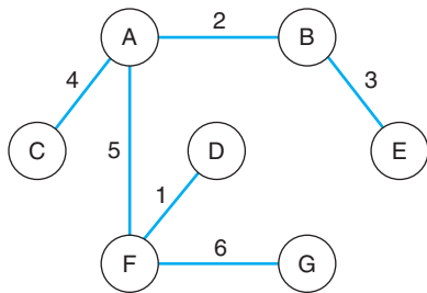
■ FIGURE 6.6H An alternative minimum spanning tree
