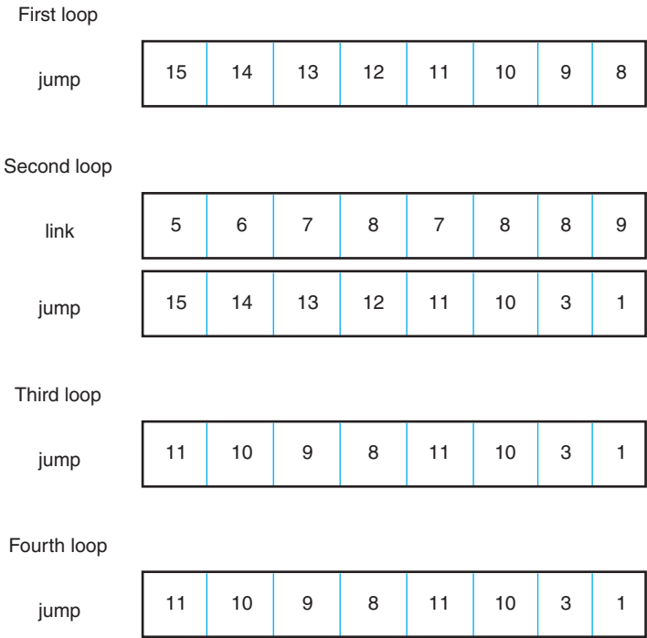
■ FIGURE 5.8 Calculation of the jump array for “datadata”
