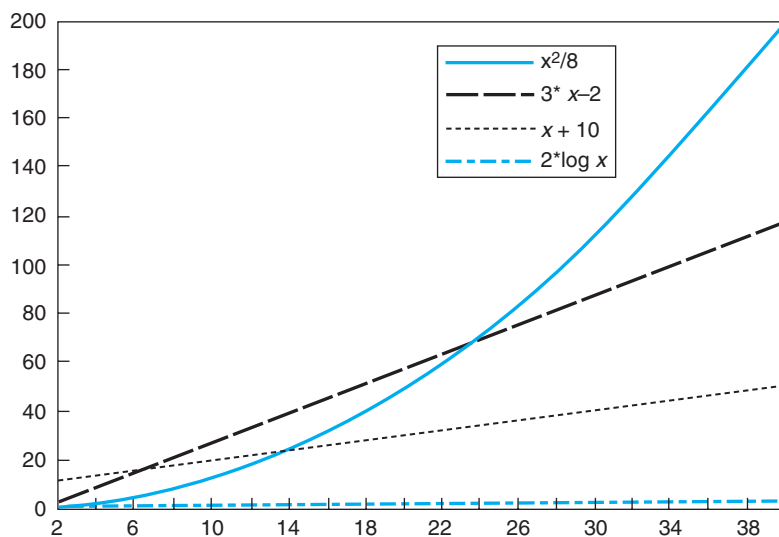
FIGURE 1.1 Graph of four functions
