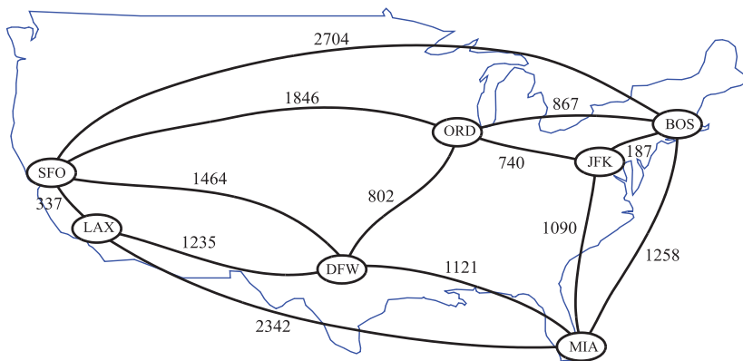
Figure 13.13: A weighted graph whose vertices represent major U.S. airports and whose edge weights represent distances in miles. This graph has a path from JFK to LAX of total weight 2,777 (going through ORD and DFW). This is the minimum weight path in the graph from JFK to LAX.
