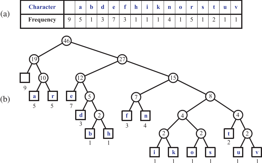
Figure 12.8: An example Huffman code for the input string X = \text{"a fast runner need never be afraid of the dark"} : (a) frequency of each character of X ; (b) Huffman tree T for string X . The code for a character c is obtained by tracing the path from the root of T to the external node where c is stored, and associating a left child with 0 and a right child with 1. For example, the code for “a” is 010, and the code for “f” is 1100.
