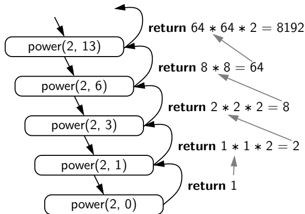
Figure 4.12: Recursion trace for an execution of \text{power}(2, 13) .
