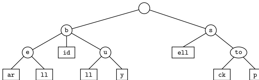
Figure 13.12: Compressed trie for the strings {bear, bell, bid, bull, buy, sell, stock, stop}. (Compare this with the standard trie shown in Figure 13.10.) In addition to compression at the leaves, notice the internal node with label to shared by words stock and stop .
