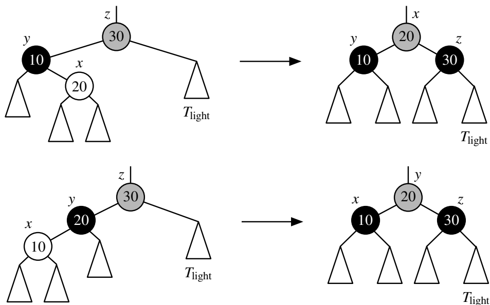
Figure 11.38: Resolving a black deficit in T_{\text{light}} by performing a trinode restructuring as \text{restructure}(x) . Two possible configurations are shown (two other configurations are symmetric). The gray color of z in the left figures denotes the fact that this node may be colored either red or black. The root of the restructured portion is given that same color, while the children of that node are both colored black in the result.
