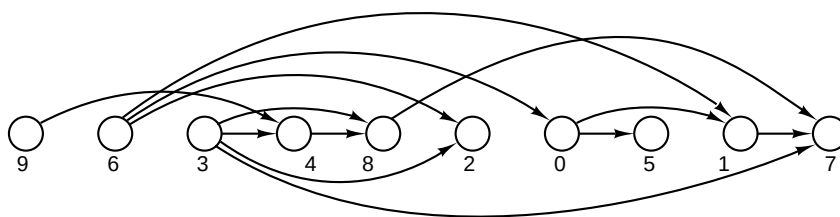
Depth-first ordering
