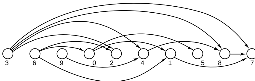
Breadth-first ordering
