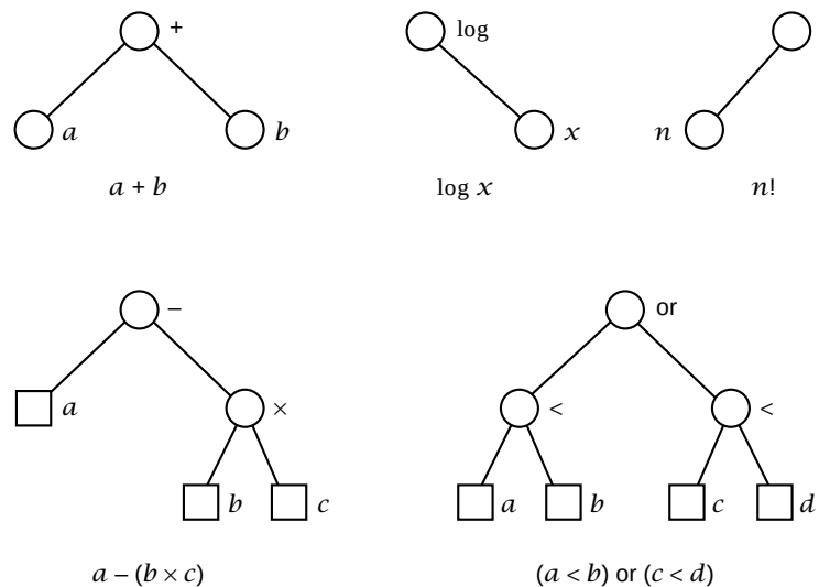
Figure 10.3. Expression trees
