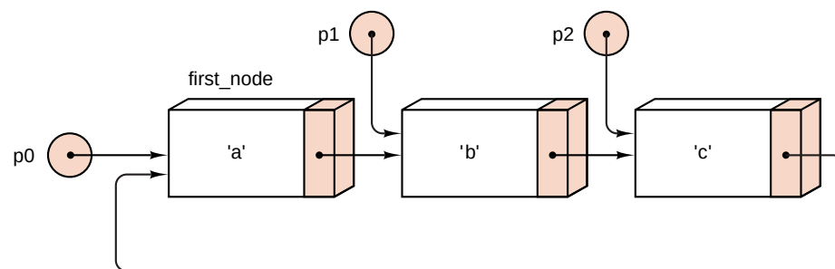
Figure 4.8. Linking nodes
