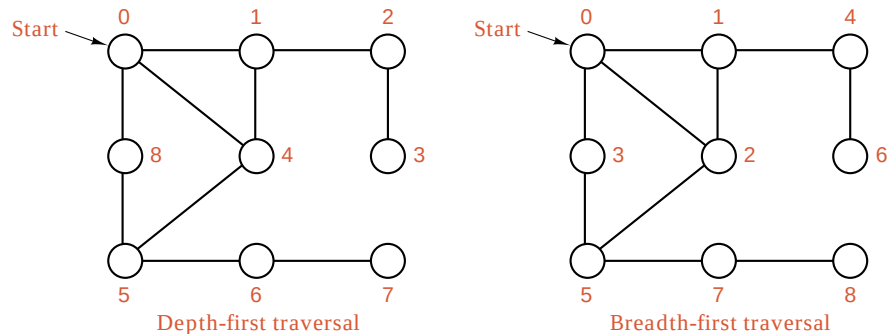
Figure 12.6. Graph traversal
