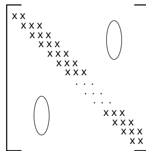
Tri-diagonal matrix
