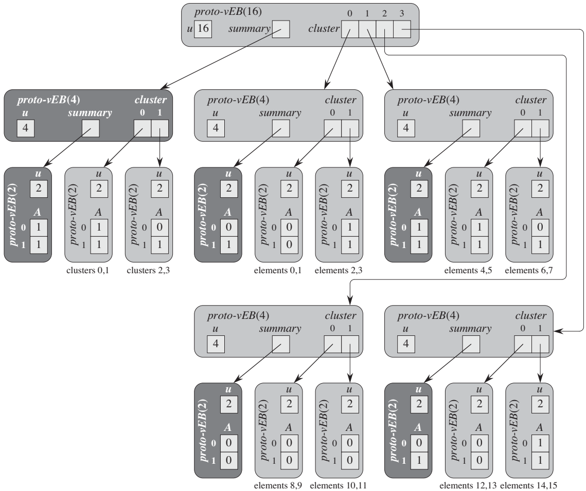
Figure 20.4 A proto-vEB(16) structure representing the set \{2, 3, 4, 5, 7, 14, 15\} . It points to four proto-vEB(4) structures in cluster [0..3] , and to a summary structure, which is also a proto-vEB(4) . Each proto-vEB(4) structure points to two proto-vEB(2) structures in cluster [0..1] , and to a proto-vEB(2) summary. Each proto-vEB(2) structure contains just an array A [0..1] of two bits. The proto-vEB(2) structures above “elements i, j ” store bits i and j of the actual dynamic set, and the proto-vEB(2) structures above “clusters i, j ” store the summary bits for clusters i and j in the top-level proto-vEB(16) structure. For clarity, heavy shading indicates the top level of a proto-vEB structure that stores summary information for its parent structure; such a proto-vEB structure is otherwise identical to any other proto-vEB structure with the same universe size.
