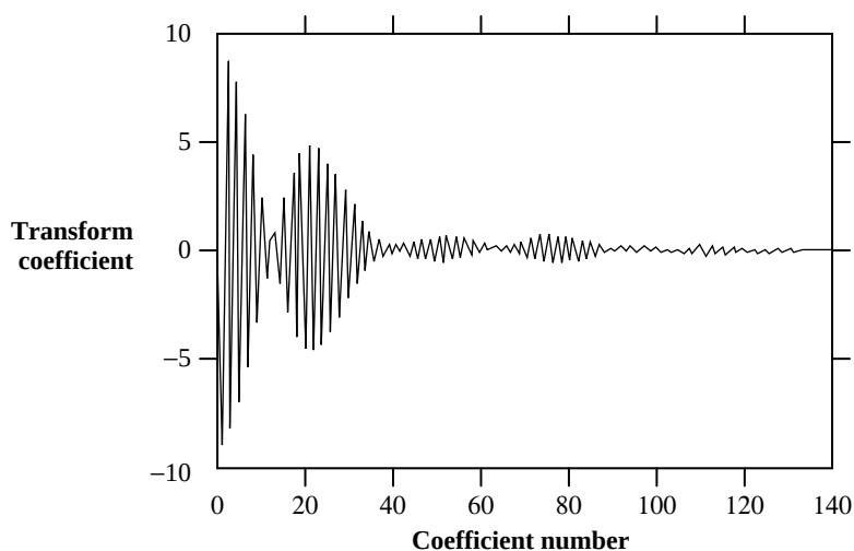
FIGURE 16.8 Transformed sequence.
