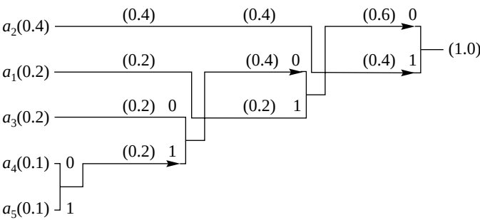
FIGURE 3. 2 Building the binary Huffman tree.
