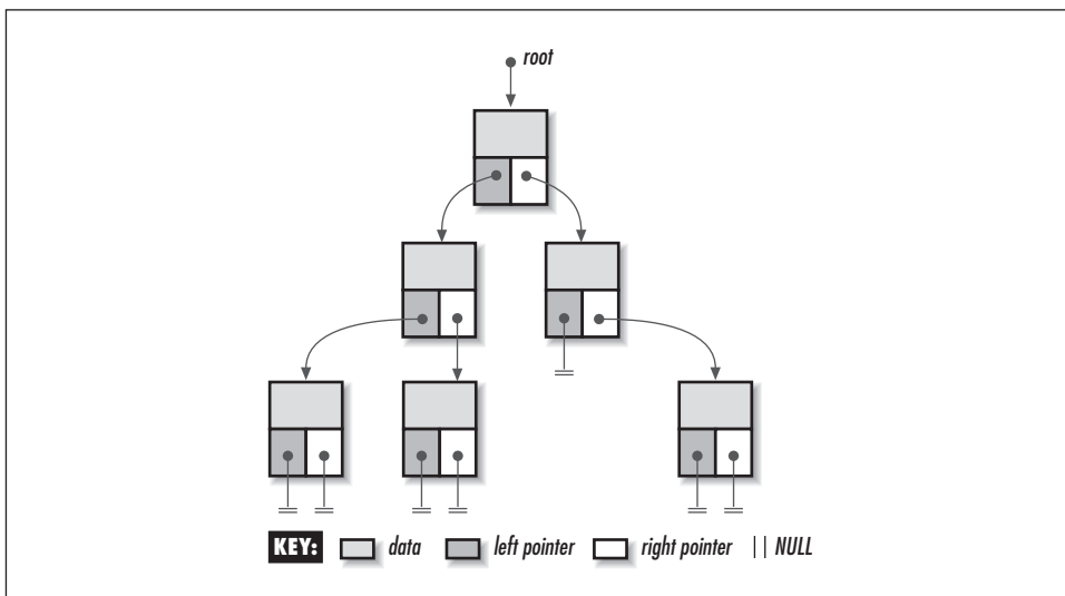
Figure 9-2. Nodes linked together form a binary tree
