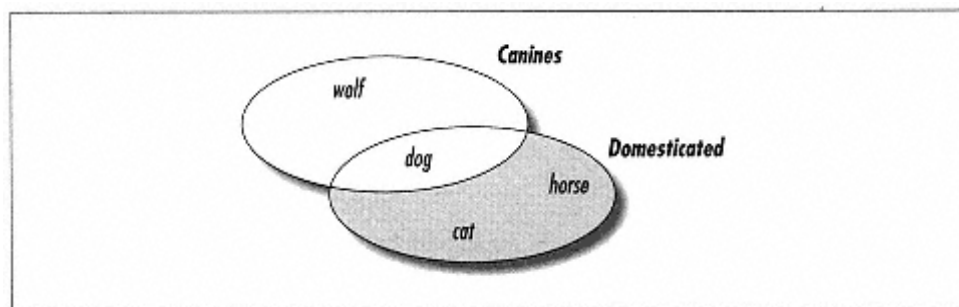
Figure 6-9. Set difference: "domesticated but not canine"
