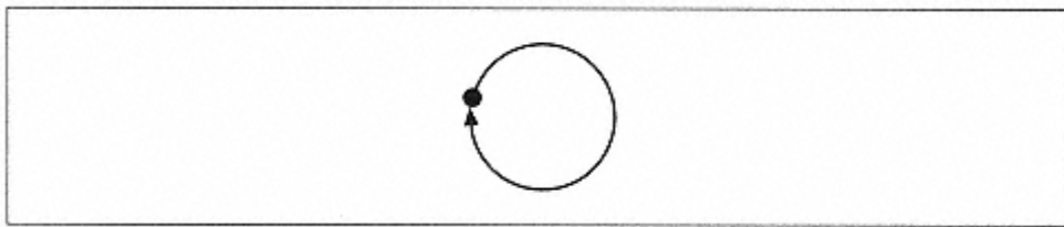
Figure 8-13. A self-looping vertex
