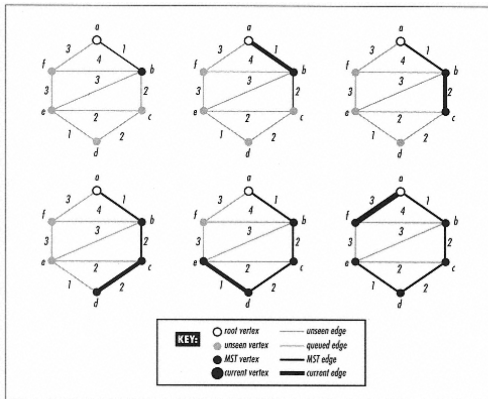
Figure 8-46. A graph and the growing of one of its Prim MSTs
