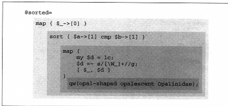
Figure 4-2. The Schwartzian Transform for our example
