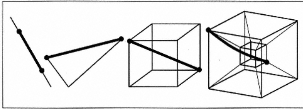
Figure 10-1. Euclidean distance in 1, 2, 3, and 4 dimensions
