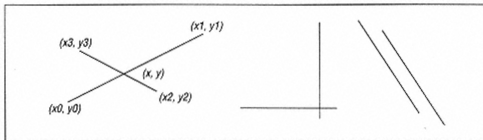
Figure 10-7. Line intersection: general case, horizontal and vertical cases, parallel case
