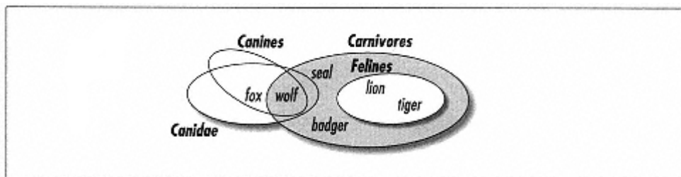
Figure 6-13. Set relations
