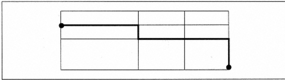
Figure 10-2. Manhattan distance
