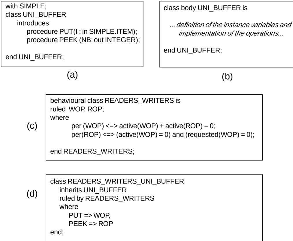
Figure 2.6 Constraint definition in DRAGOON.
