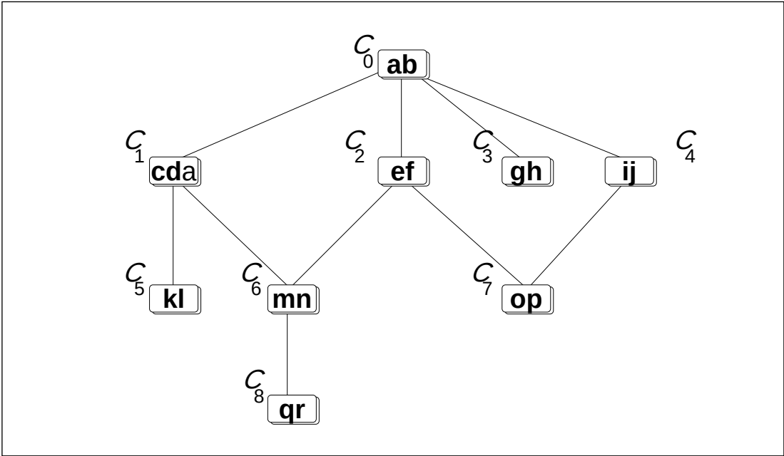
Figure 9.3 Inheritance structure of a set of classes.
