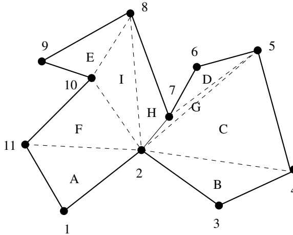
Figure 14.2. Triangulating a polygon via the van Gogh (ear-cutting) algorithm, with triangles labeled in order of insertion ( A - I ).
