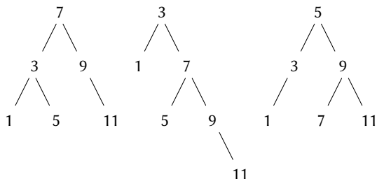
Figure 2.16: Various binary trees that represent the set \{1, 3, 5, 7, 9, 11\} .
