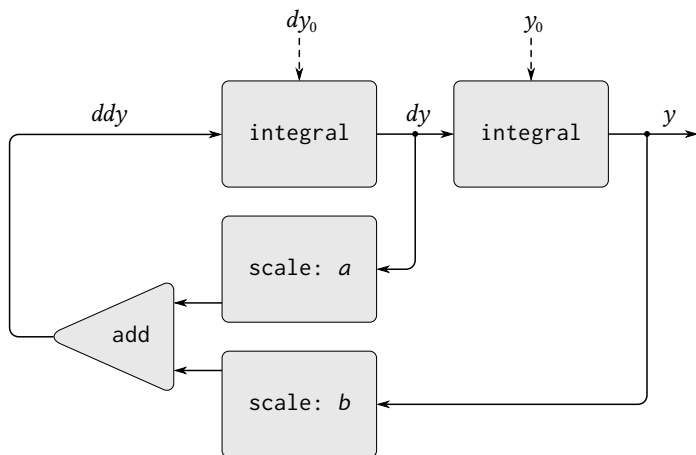
Figure 3.35: Signal-flow diagram for the solution to a second-order linear differential equation.
