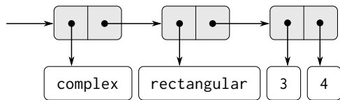
Figure 2.24: Representation of 3 + 4i in rectangular form.
