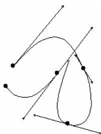
Figure 25.7 - Courbe de Bézier
