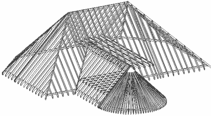
Figure 38.52 - La charpente RoofMaker en volume
