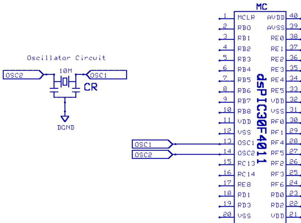
Fig H5 Ceramic Resonator circuit
