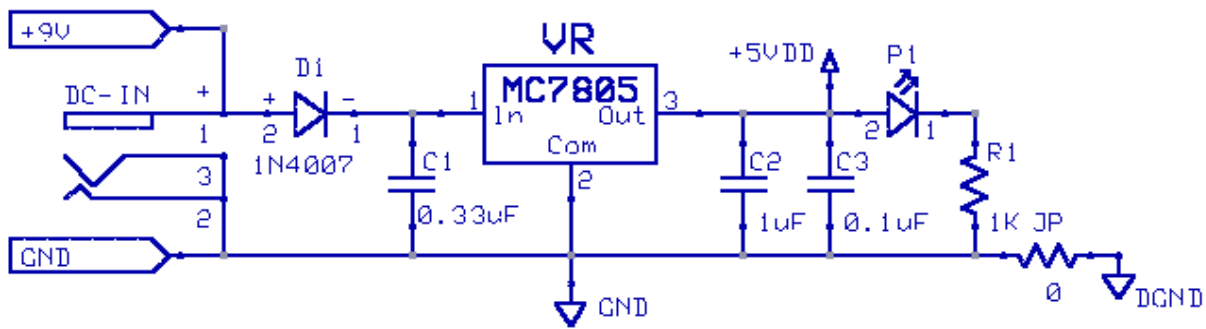
Fig H6 Power supply module
