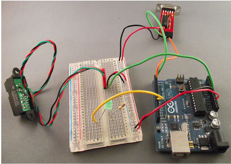
Figure 10.23 GP2D12 infrared sensor added to circuit
