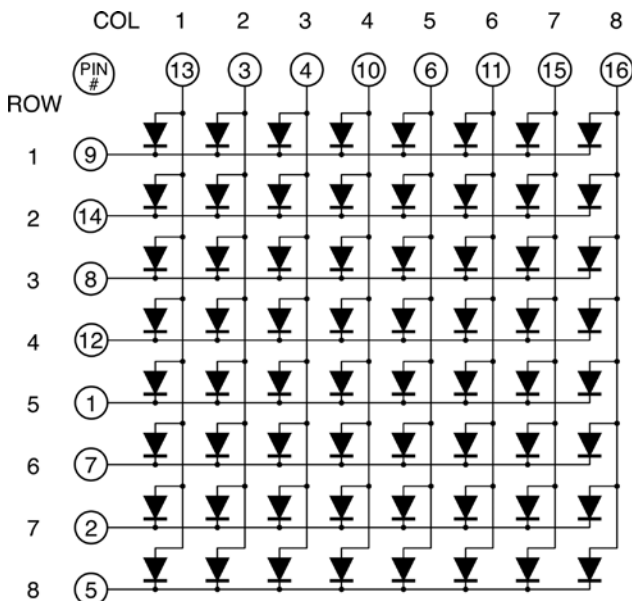
Figure 7-2. A typical schematic for an 8×8 LED dot matrix display
