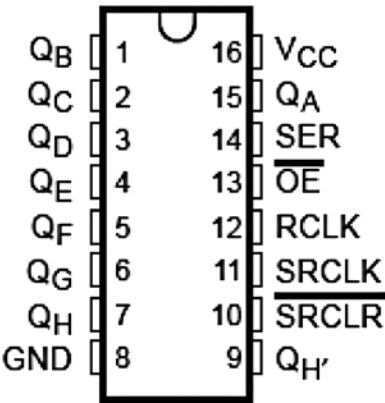
Figure 6-2. Pin diagram of a 595 chip
