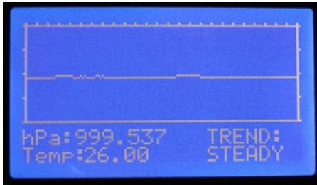
Figure 11-8. The display for Project 32 – Digital Barograph
