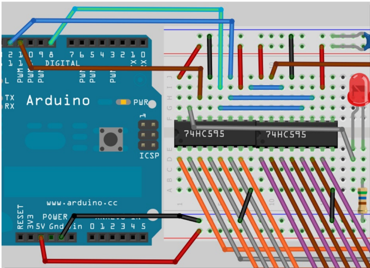
Figure 6-5. The circuit for Project 18. Close up of the wiring of the ICs
