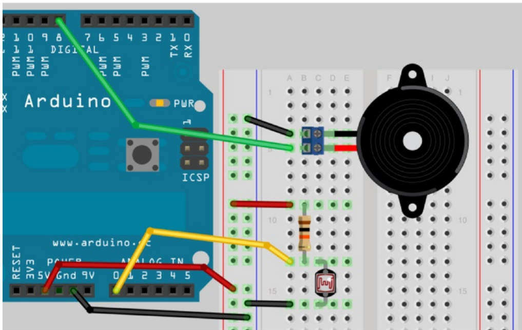
Figure 4-4. The circuit for Project 14 – Light Sensor
