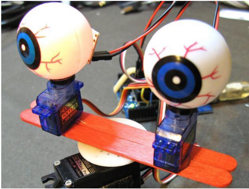
Figure 9-2. Three servos controlling a head and eyeballs for a robot (image by Tod E. Kurt)
