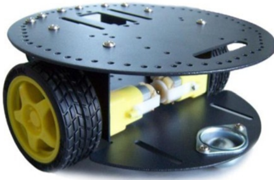
Figure 10-7. A two-wheeled robot base (image courtesy of DFRobot)
