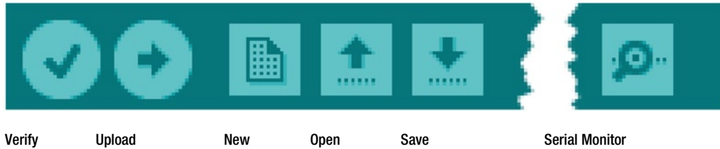
Figure 1-16. The Toolbar
