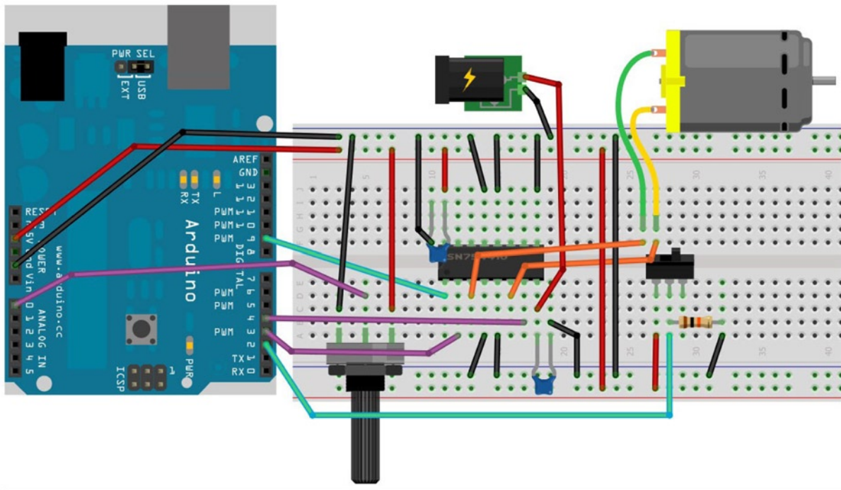
Figure 5-3. The circuit for Project 16
