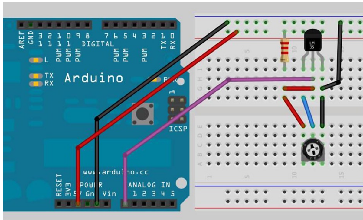
Figure 13-1. The circuit for Project 36 – Serial Temperature Sensor
