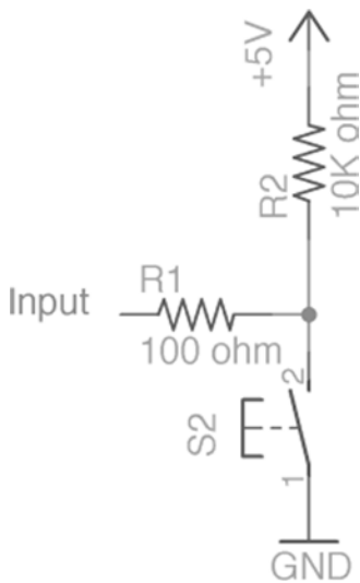
Figure 2-11. A pull-up resistor circuit
