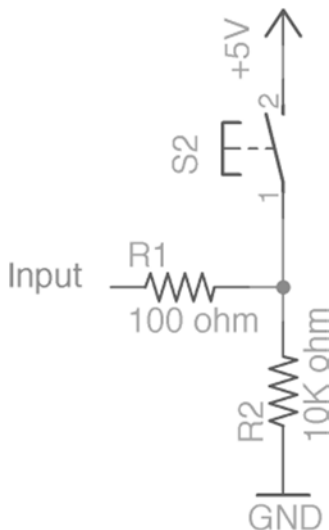
Figure 2-10. A pull-down resistor circuit
