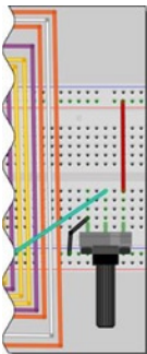
Figure 7-8. Add a potentiometer to the Project 21 circuit. The middle pin of the potentiometer goes to Analog Pin 5
