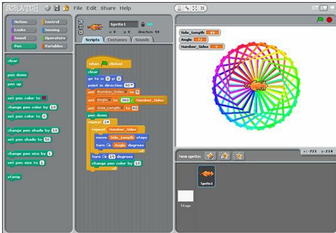
Figure 4-7 The results of adding the change pen shade by 10 block
