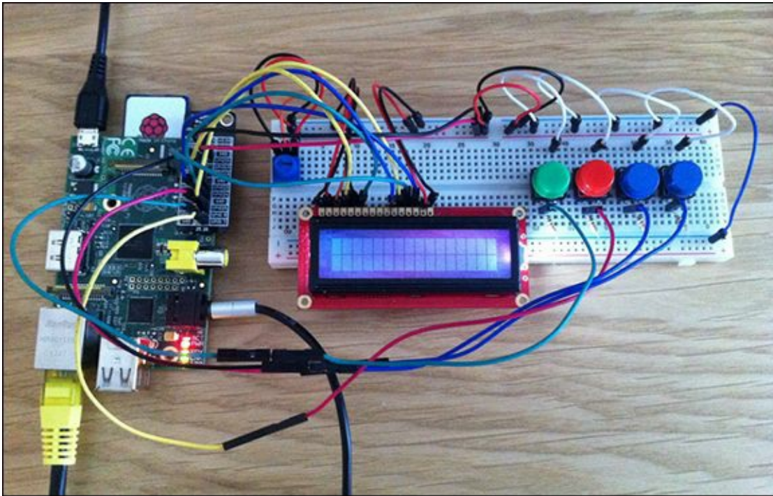
Figure 9-9 Completed wiring of Pi jukebox with buttons
