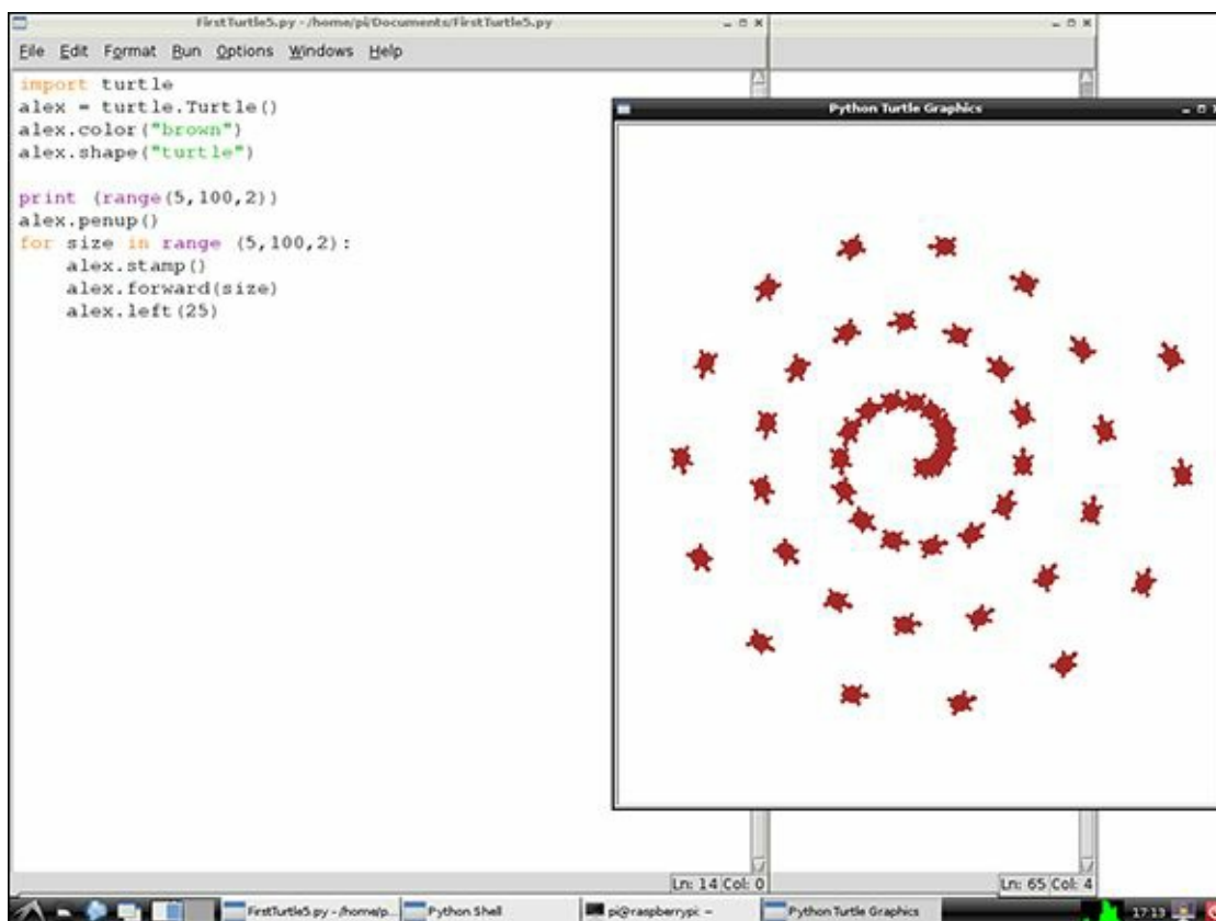
Figure 4-15 Using penup and stamp to create spiralTurtle2.py
