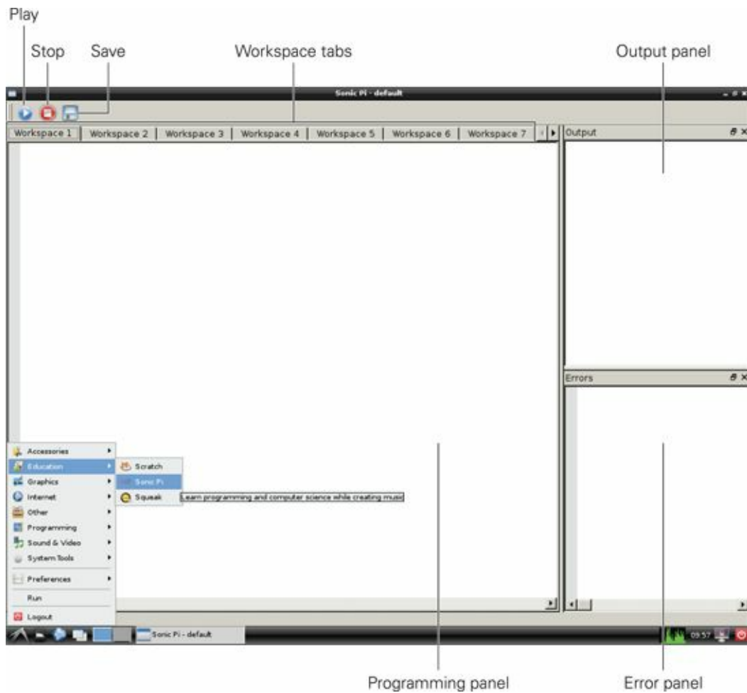
Figure 7-3 The Sonic Pi interface
