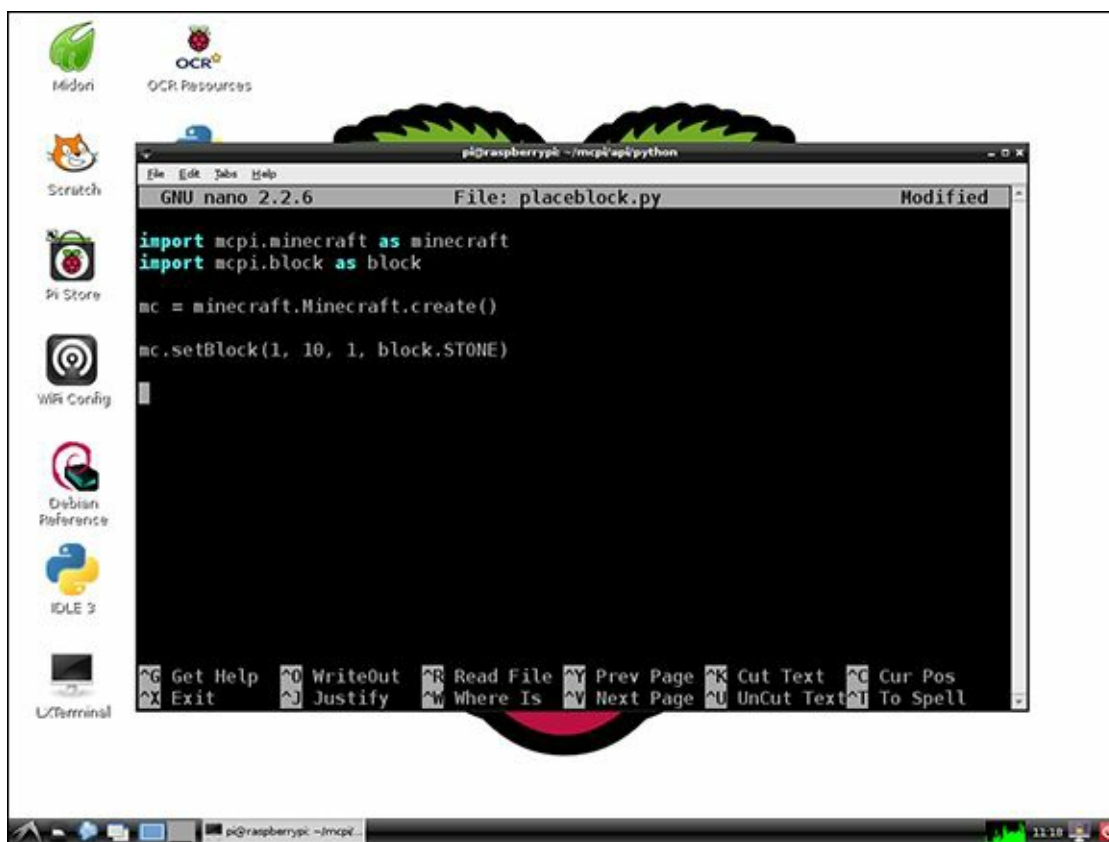
Figure 6-6 Using setBlock in Minecraft Pi
