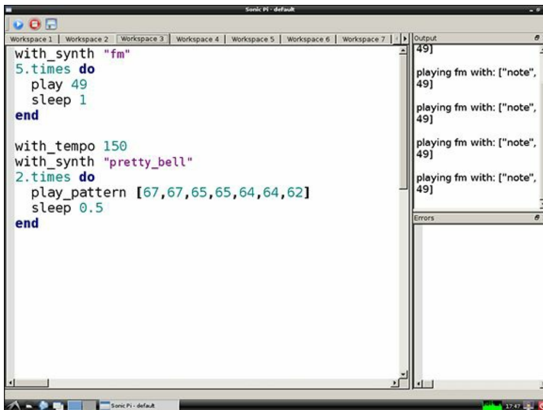
Figure 7-9 Using different synthesizer sounds in Sonic Pi
