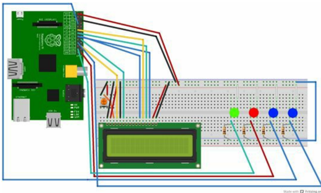
Figure 9-8 Wiring diagram for the four jukebox buttons
