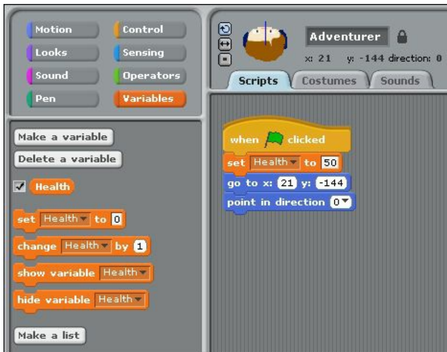
Figure 3-16 The Adventurer sprite start script so far
