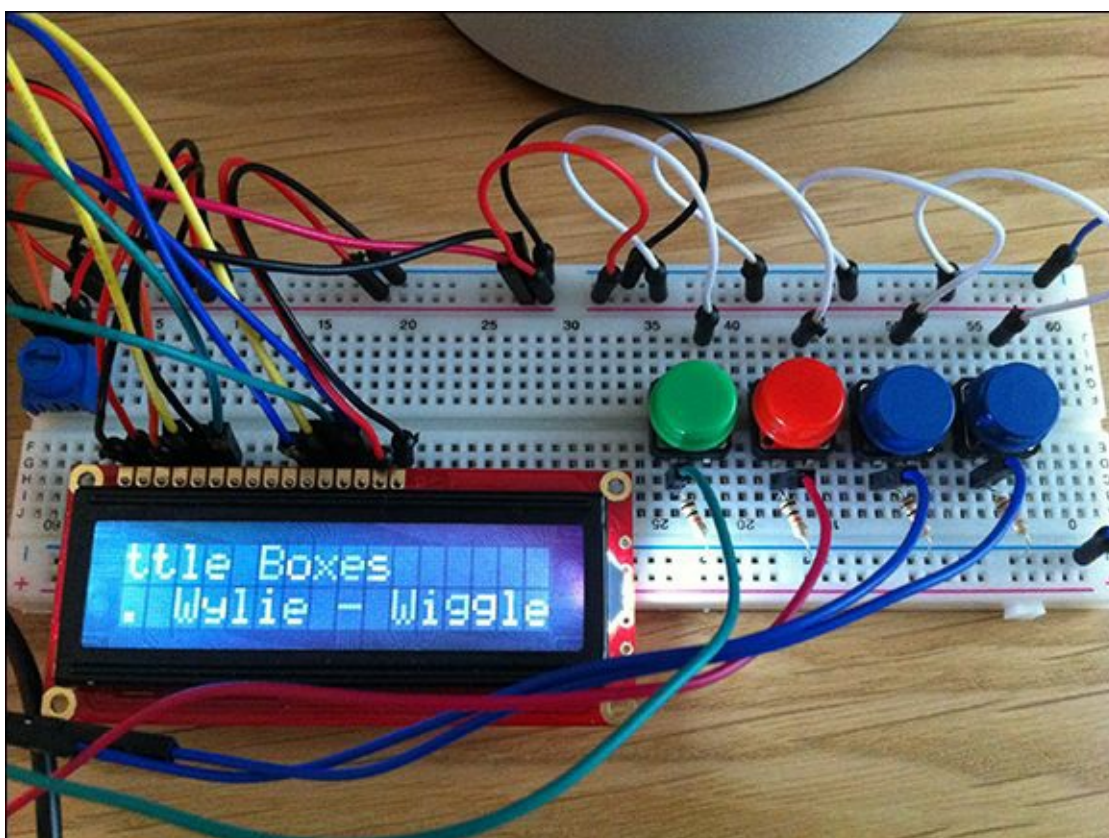
Figure 9-10 Jukebox LCD in action displaying MP3 metadata
