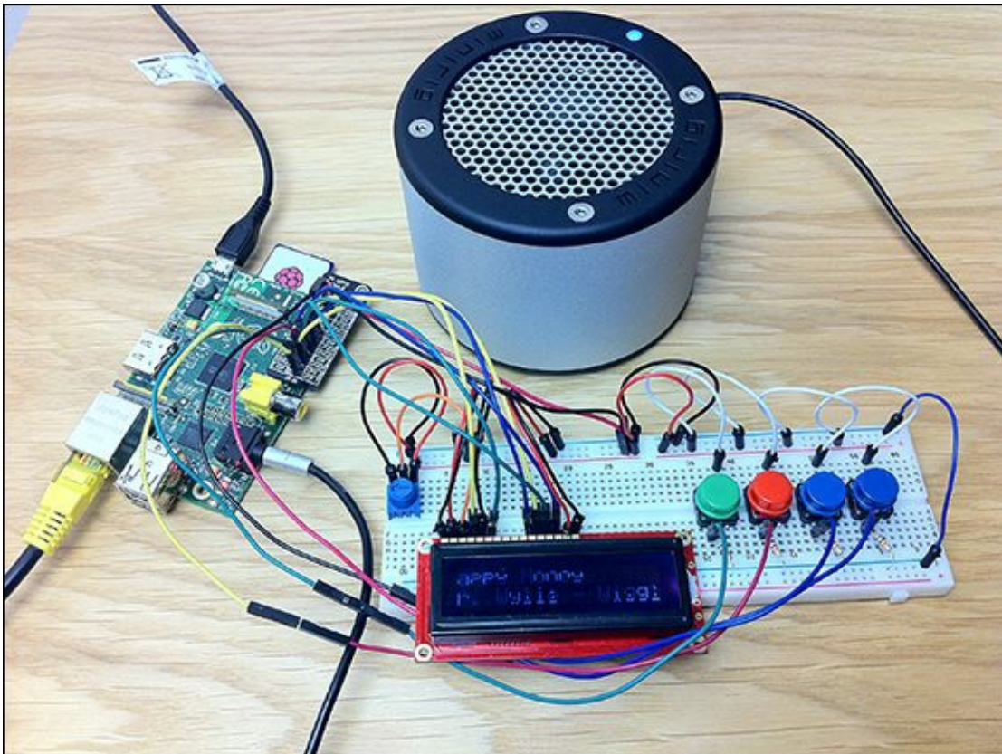
Figure 9-1 The completed Adventures in Raspberry Pi Big Jukebox Project !
