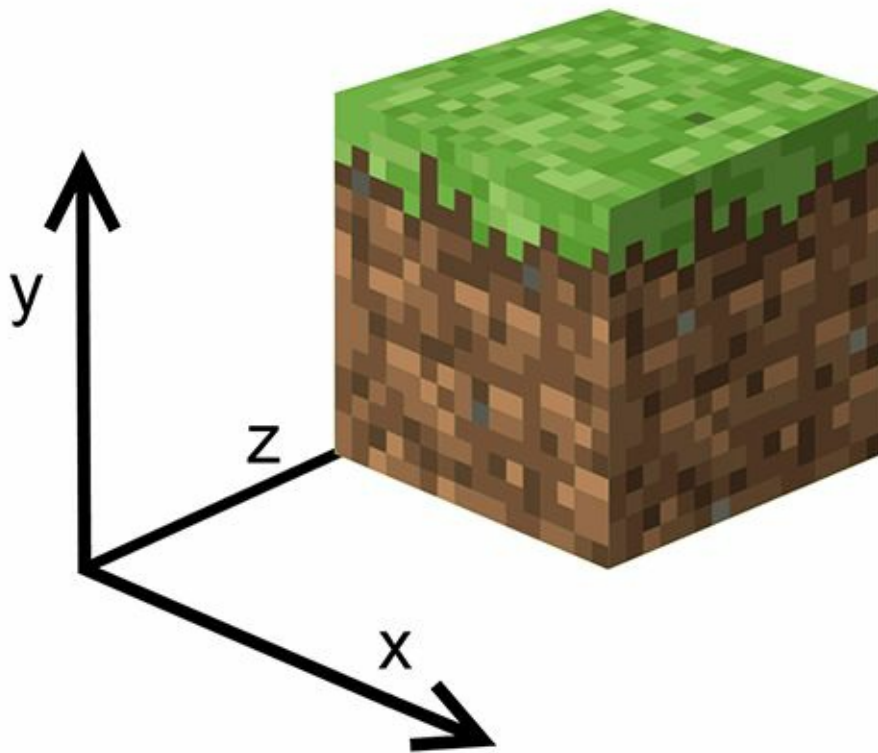
Figure 6-4 x, y and z coordinates
