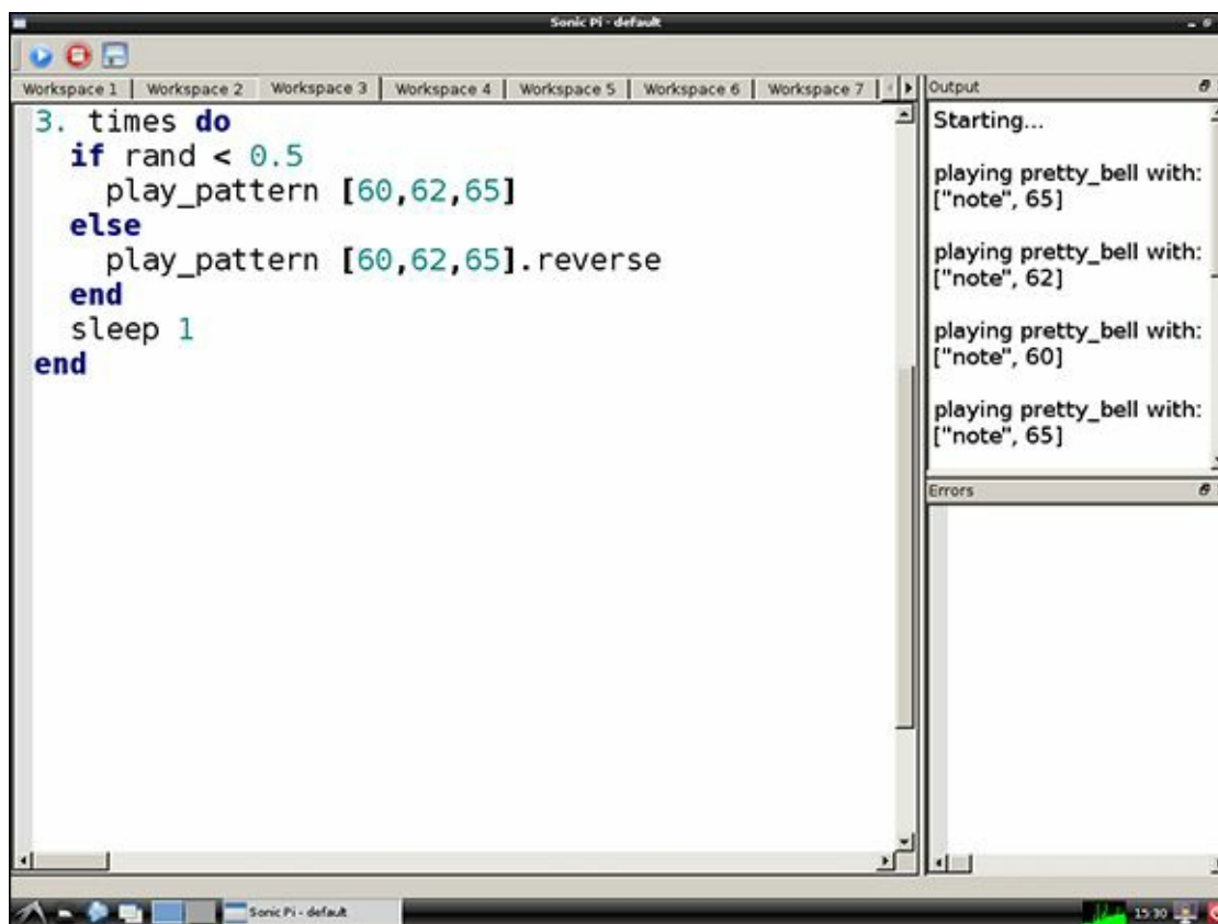
Figure 7-11 Using algorithms to change the order of notes in lists
