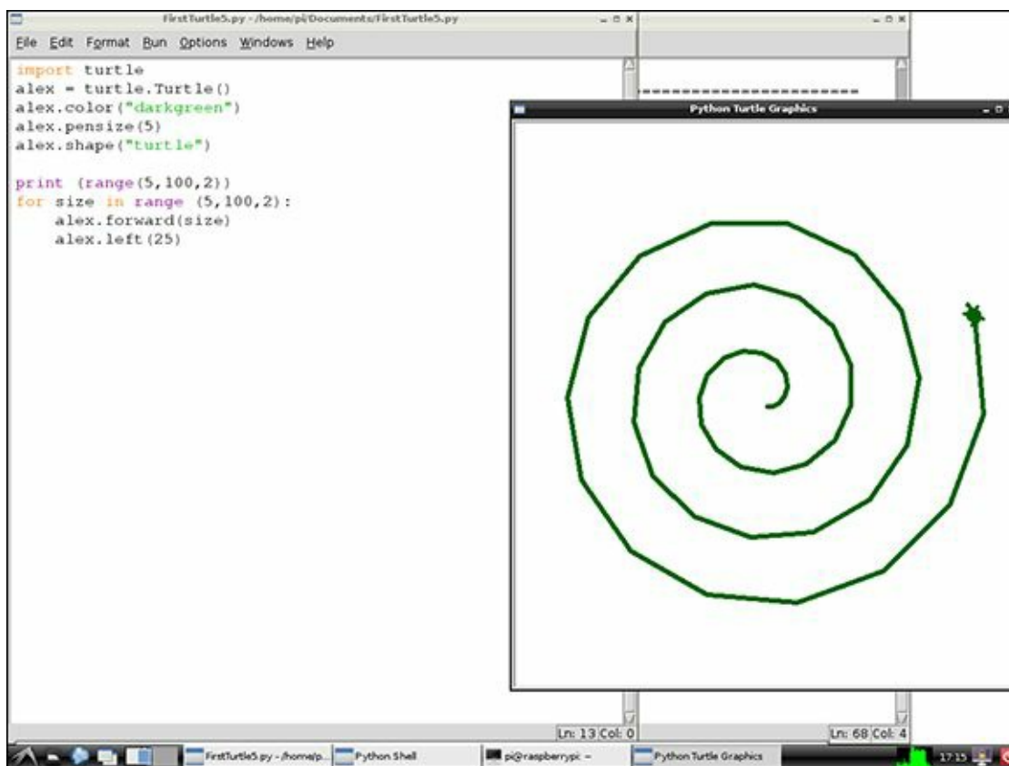
Figure 4-14 Using pensize and color to create spiralTurtle1.py
