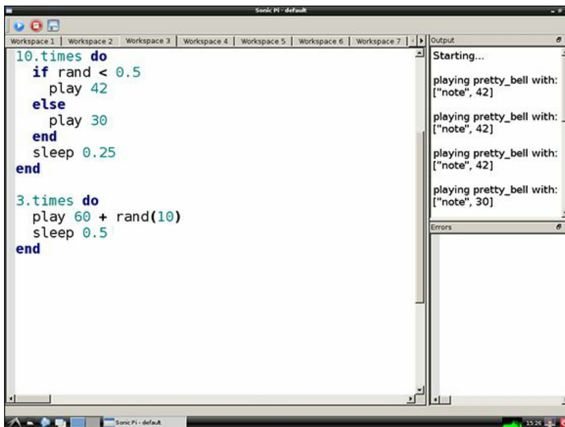
Figure 7-10 Using conditionals and random in Sonic Pi
