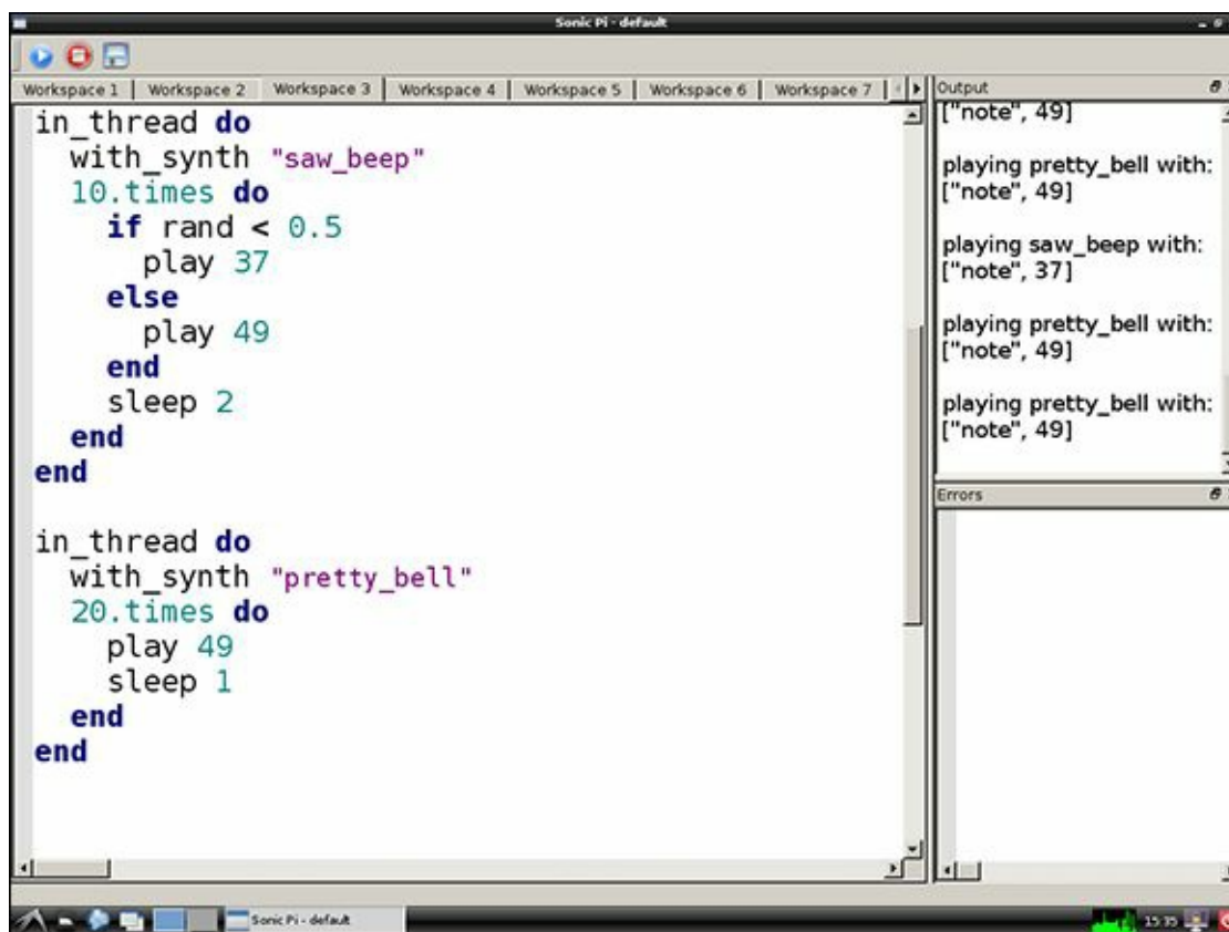
Figure 7-12 Playing multiple tunes at the same time using threads
