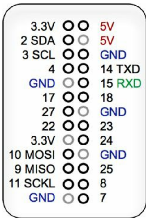
Figure 8-3 The Raspberry Leaf for the Rev 2 board
