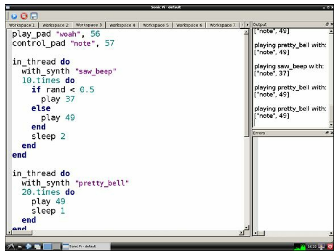
Figure 7-13 Adding pads in Sonic Pi
