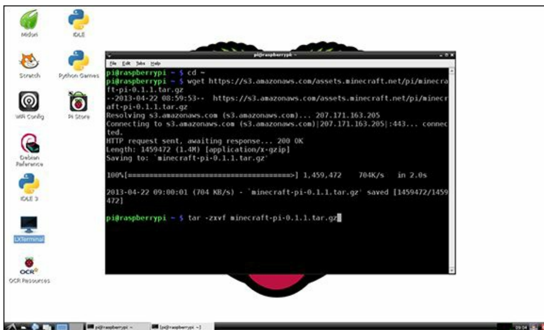
Figure 6-2 Minecraft Pi downloading and extraction commands via the LXTerminal on Raspberry Pi
