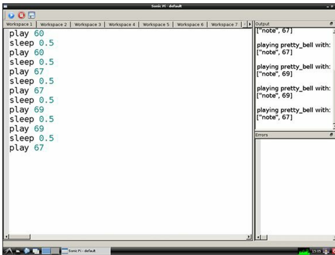
Figure 7-6 Using play and sleep to play Twinkle Twinkle Little Star in Sonic Pi
