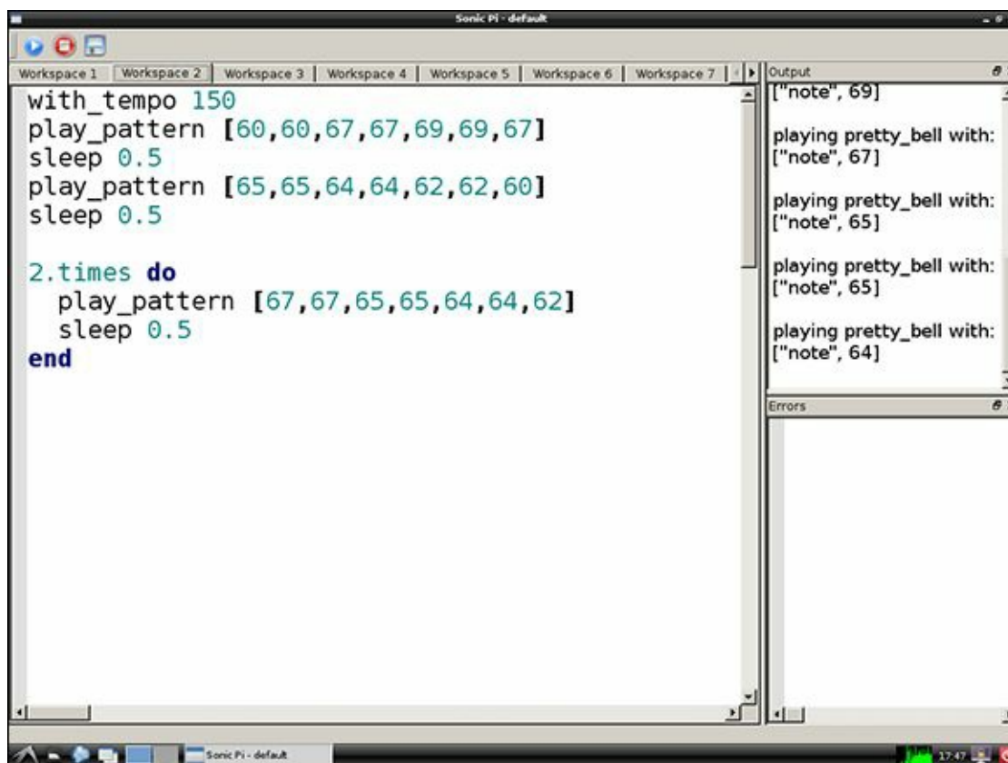
Figure 7-8 Using repeating loops in Sonic Pi
