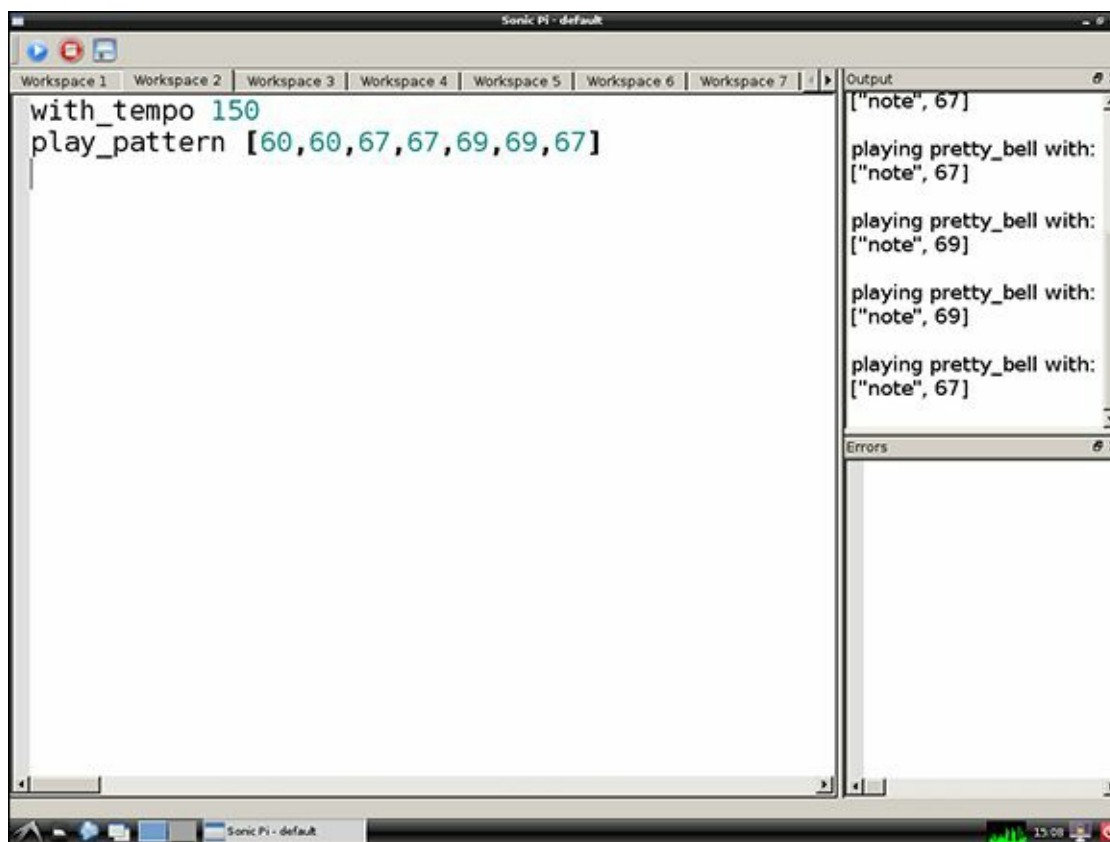
Figure 7-7 Using a list in Sonic Pi to play notes
