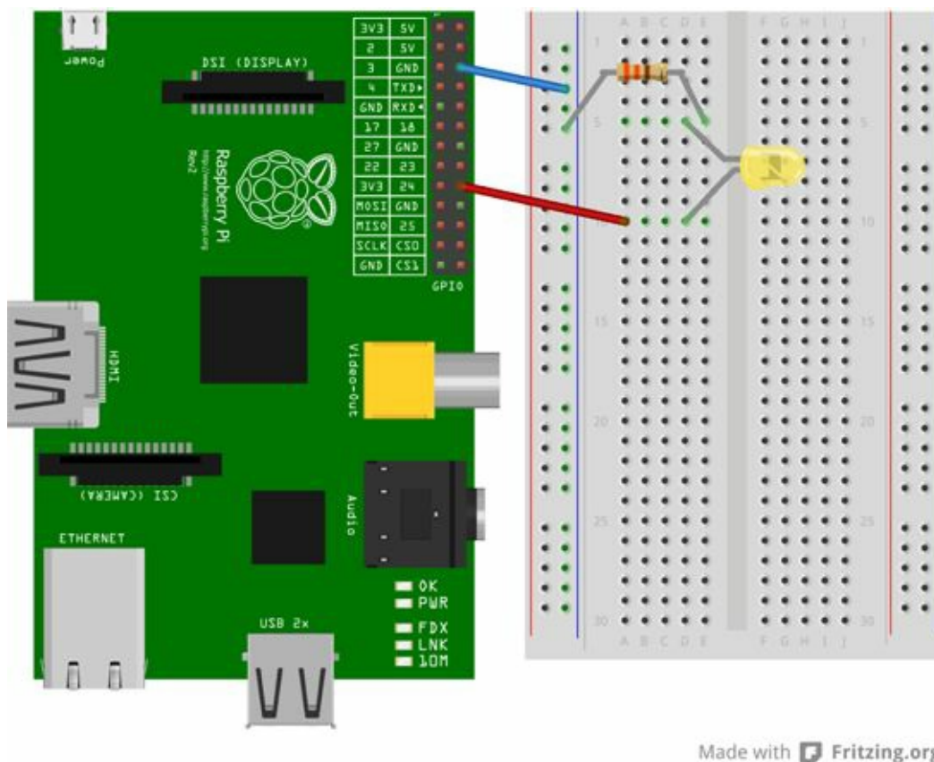
Figure 8-8 Circuit diagram to connect components to Raspberry Pi for a blinking LED
