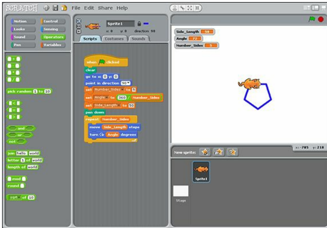
Figure 4-4 Using variables instead of values in Scratch
