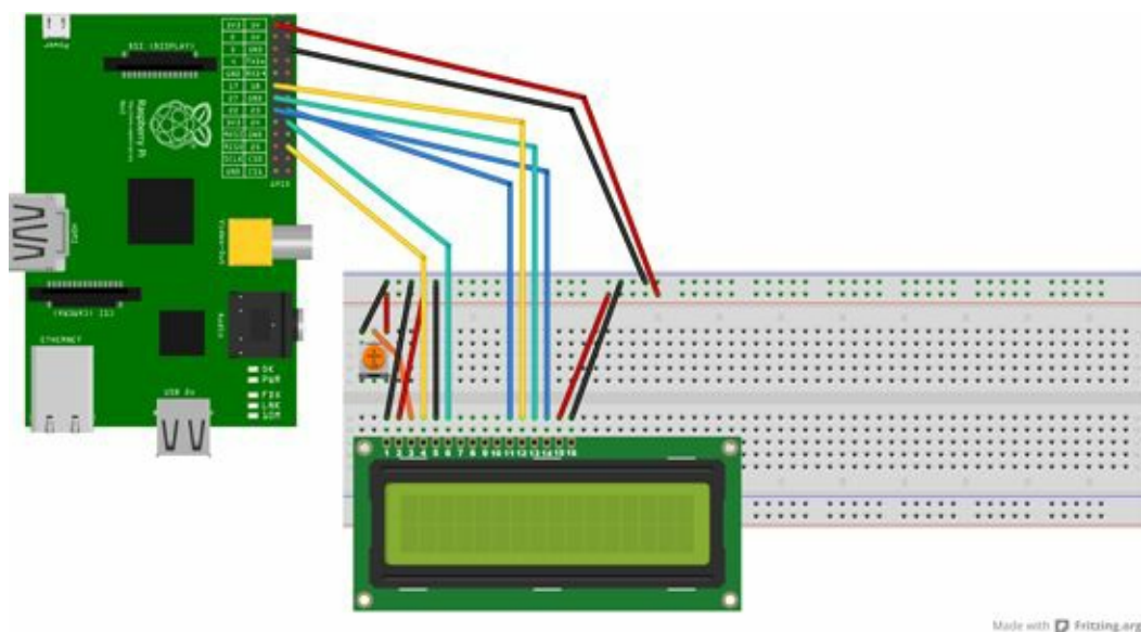
Figure 9-2 Circuit diagram for wiring the LCD screen and potentiometer
