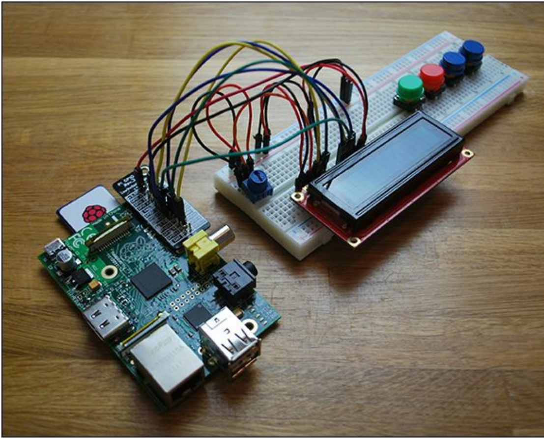
Figure 9-3 Mounted LCD screen and potentiometer
