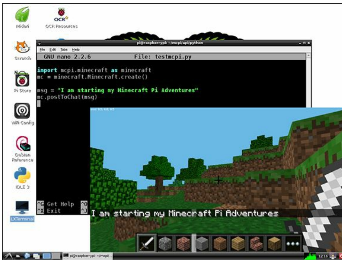
Figure 6-3 Your first Minecraft Pi Python program
