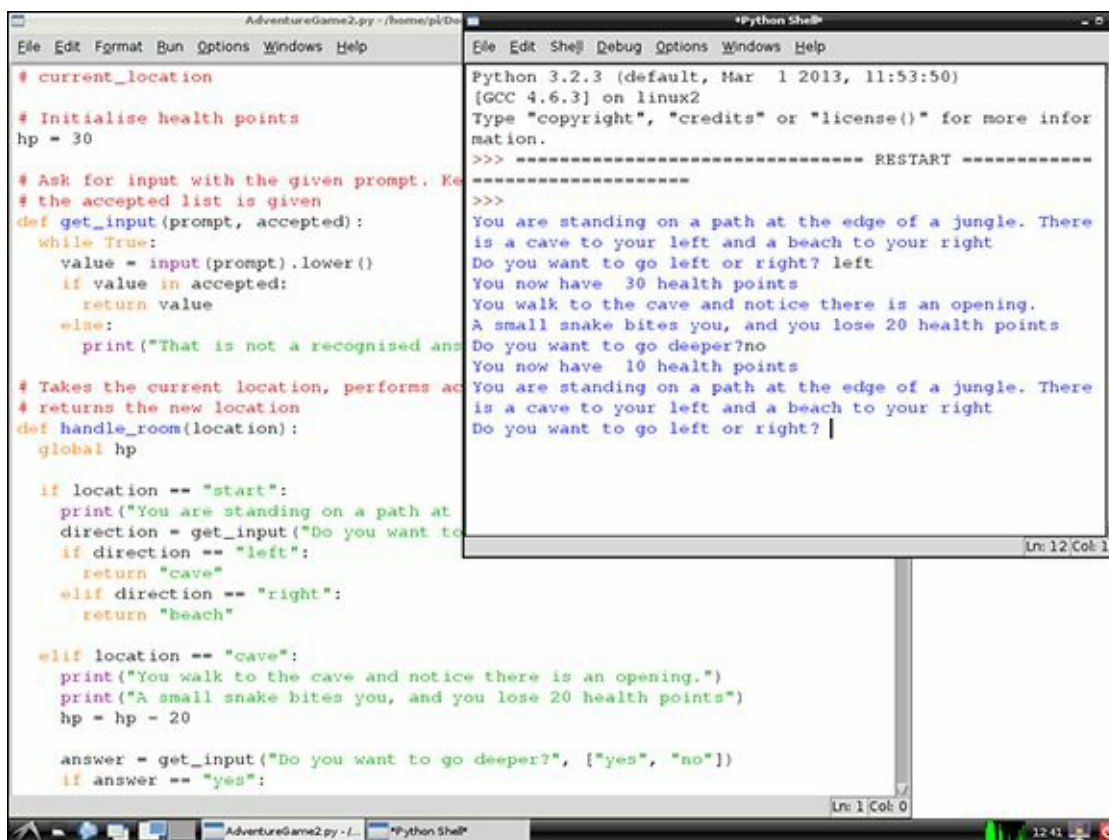
Figure 5-13 The Python Adventure Game in action, using the newly defined functions
