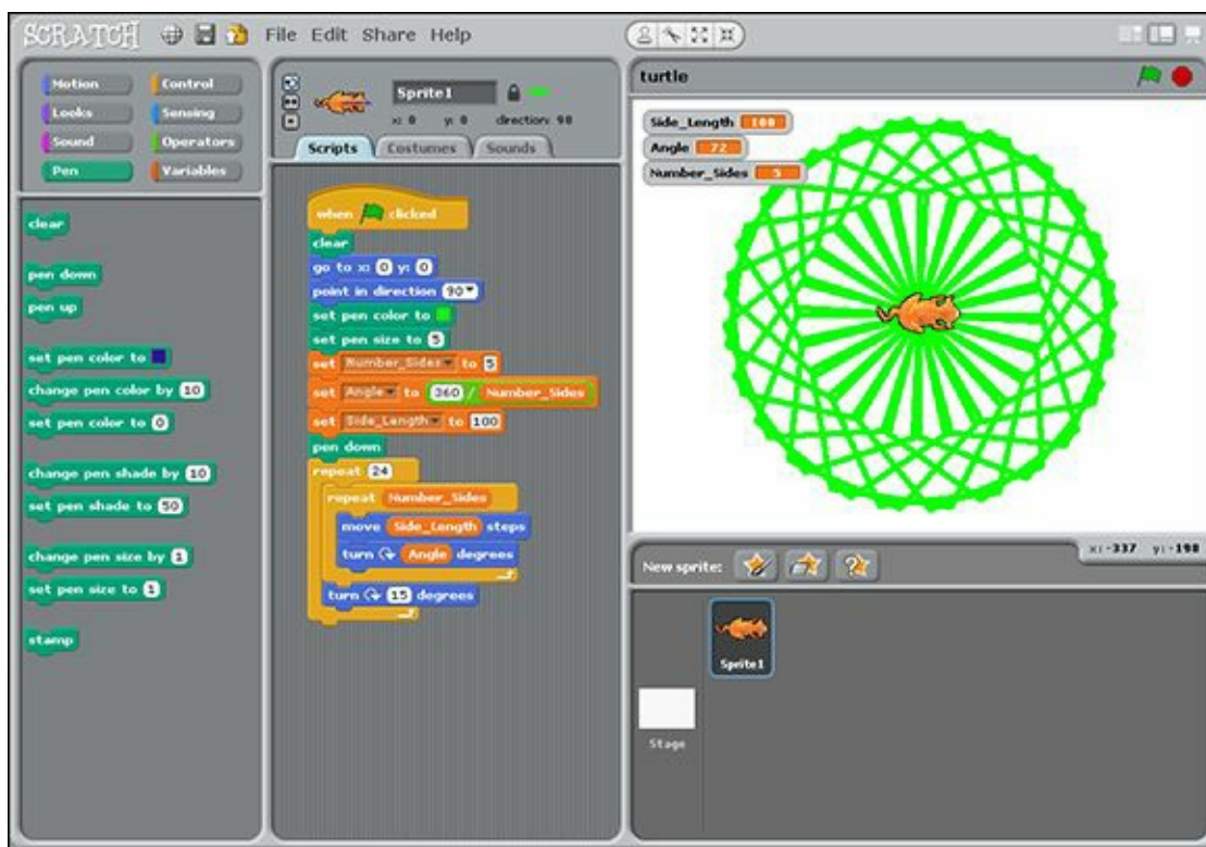
Figure 4-6 Creating repeating pentagon spirals
