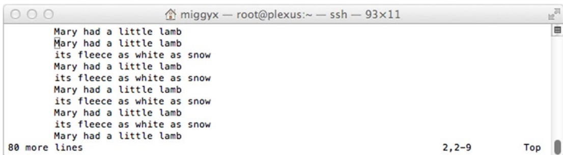
Figure 6-25. Mass pasting
