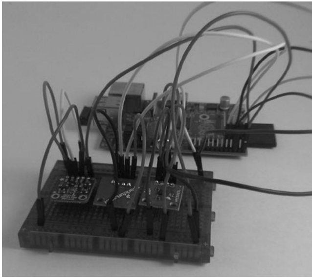
Figure 6-12. Breadboarded chips
