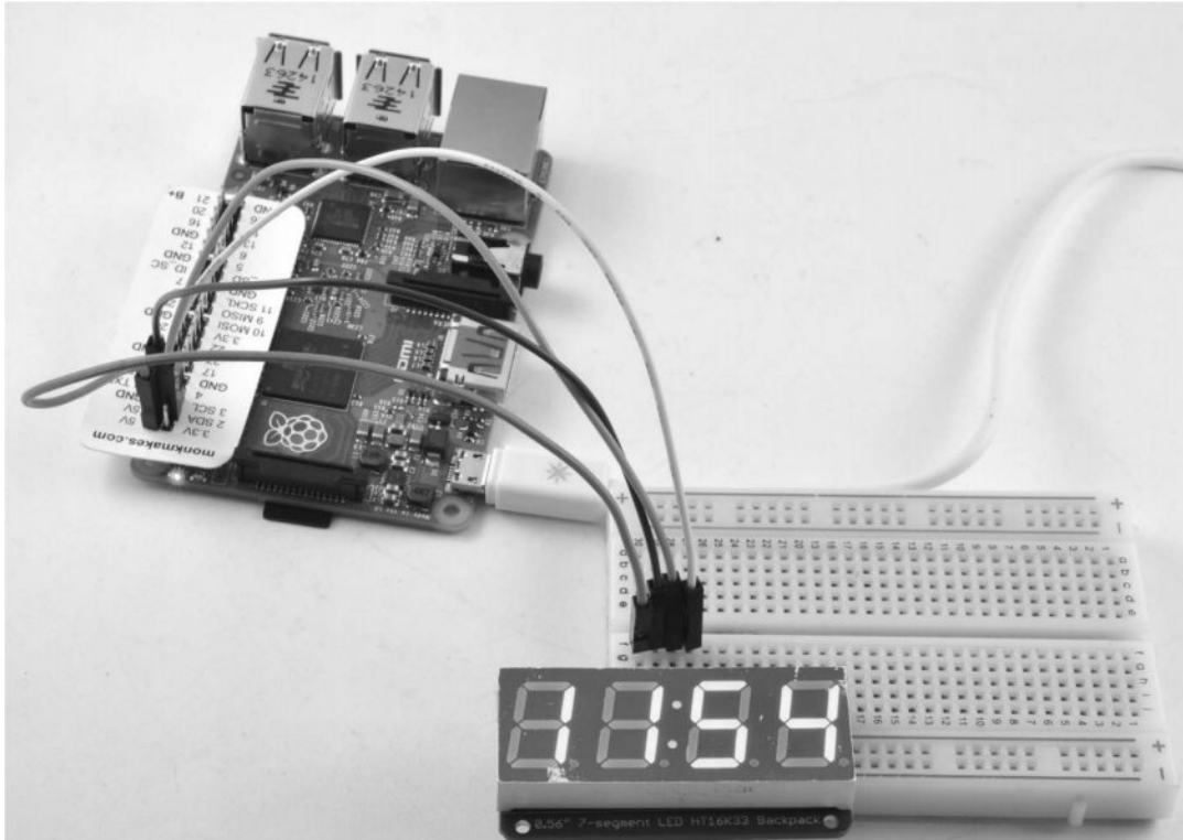
Figure 11-1 LED clock using the Raspberry Pi.
