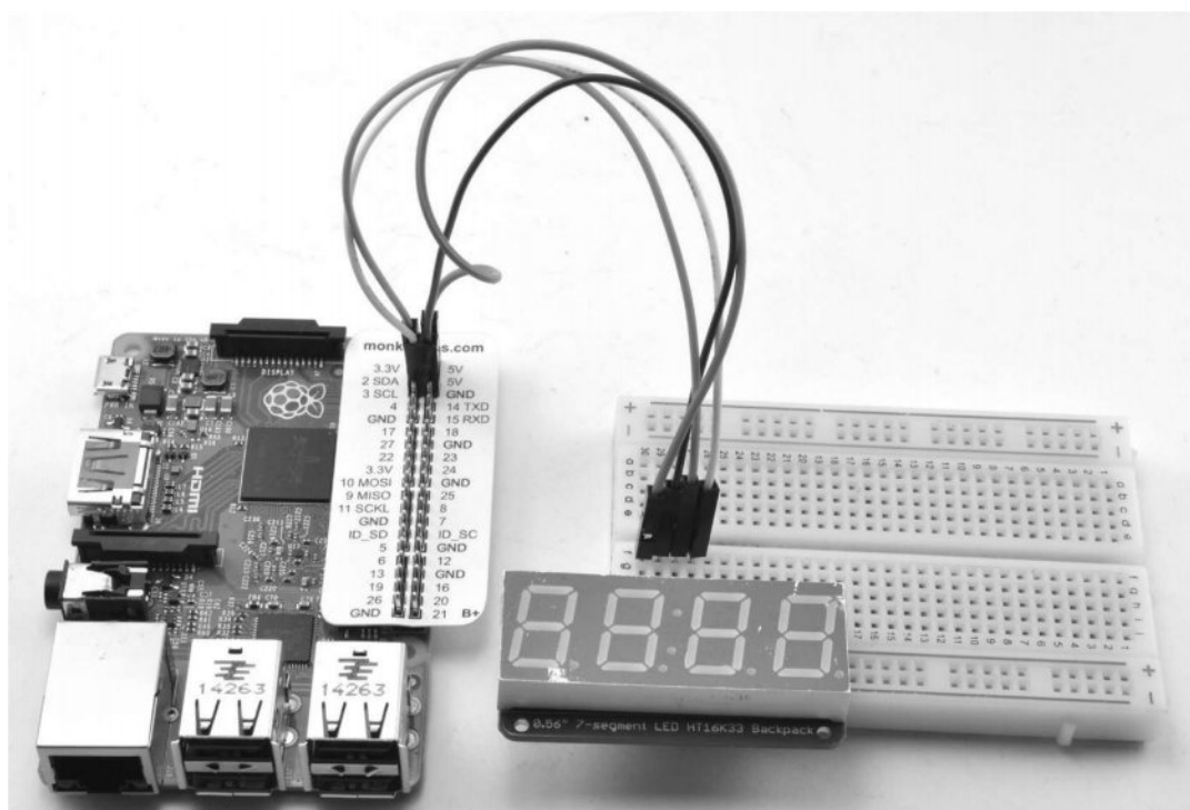
Figure 11-2 Breadboard layout.
