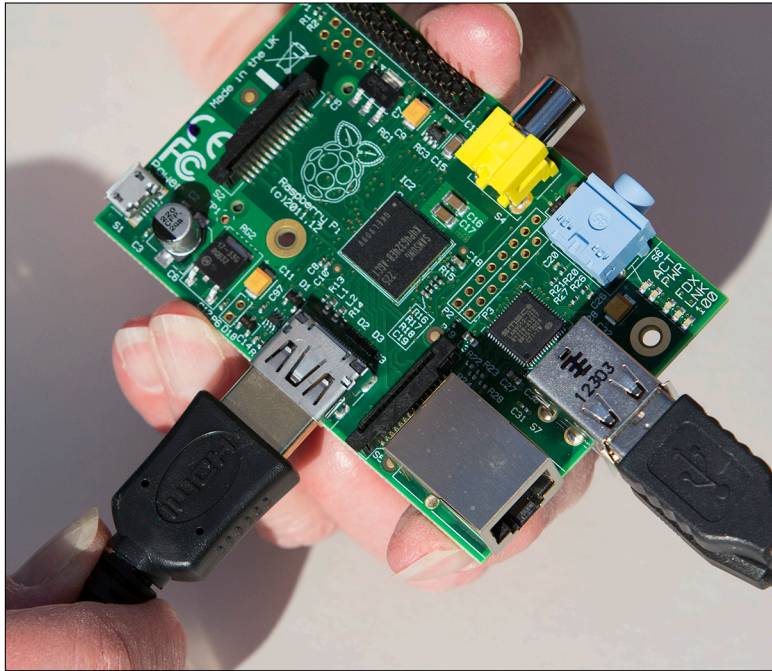
FIGURE A-5: HDMI connection on the Raspberry Pi.
