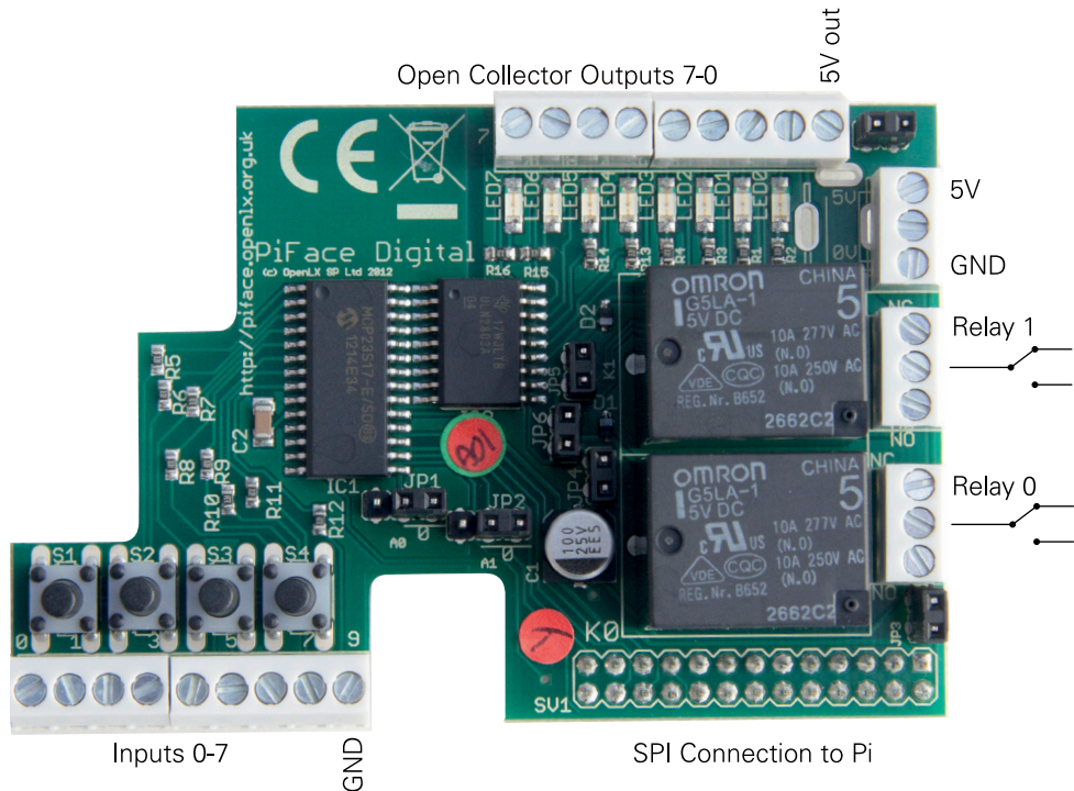
FIGURE 1-5: PiFace Digital's connectors.
