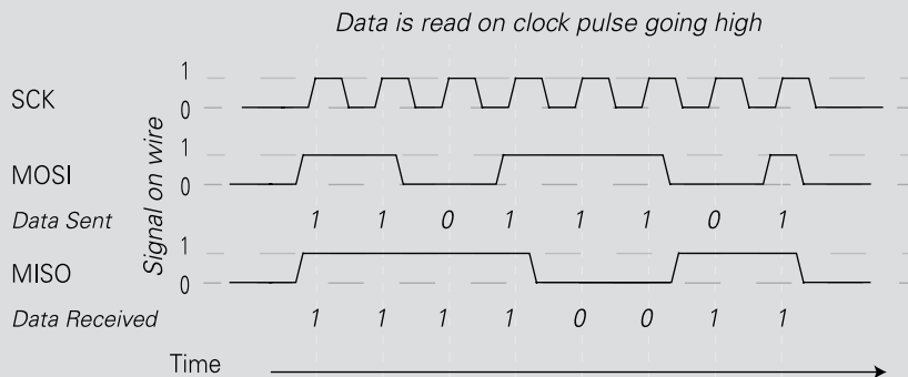
FIGURE 1-1: Example SPI transaction: The microprocessor sends data 11011101, and the device sends 11110011.
