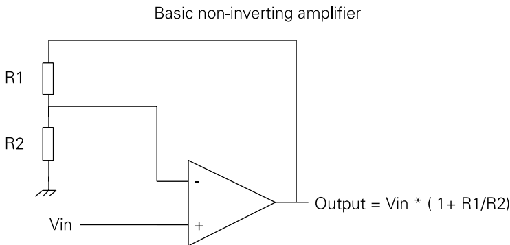
FIGURE 3-6: A non-inverting amplifier.
