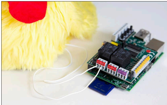
FIGURE 2-5: Wiring the toy up to the normally open relay contacts.
