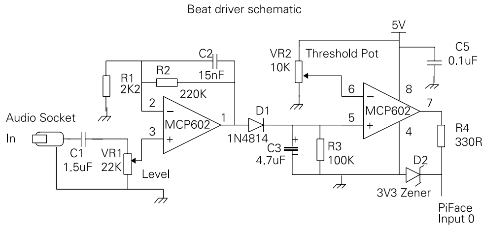
FIGURE 3-7: The schematic of the beat driver.
