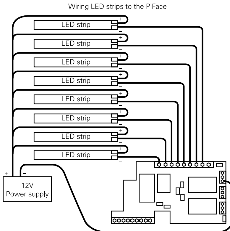
FIGURE 3-5: Wiring the LED strip to the PiFace board.
