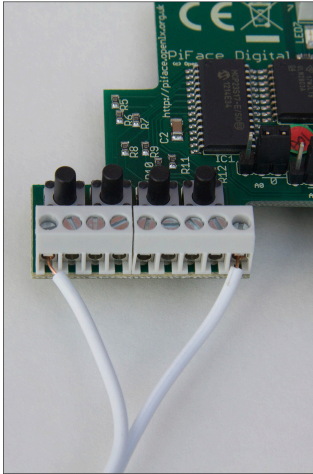
FIGURE 1-13: Wiring up a switch.
