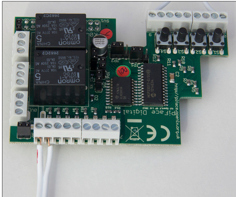
FIGURE 1-14: Wiring up an LED.
