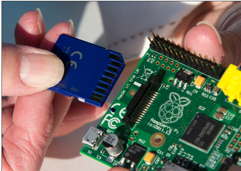
FIGURE A-10: Insert the SD card carefully.
