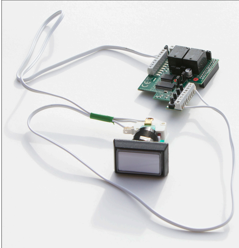
FIGURE 1-8: Wiring up the LED and switch to the Raspberry Pi.
