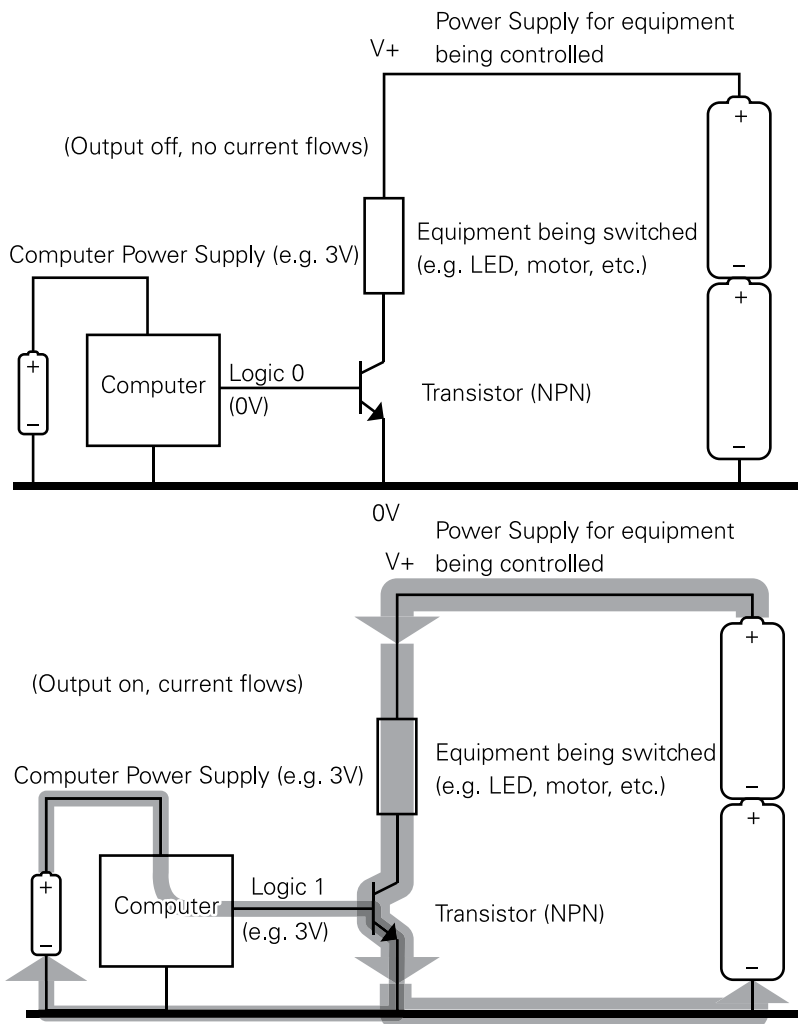
FIGURE 1-7: How to wire up an open-collector output.
