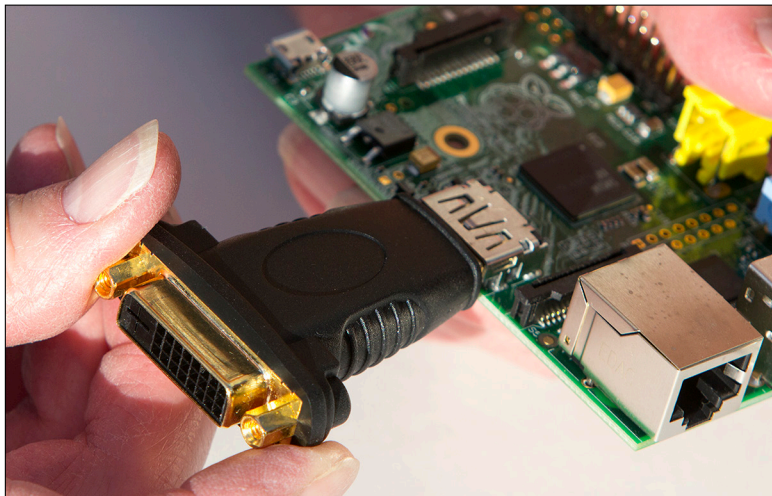
FIGURE A-6: HDMI-DVI adapter.
