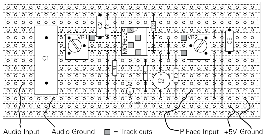
FIGURE 3-8: The physical layout of the beat driver circuit.
