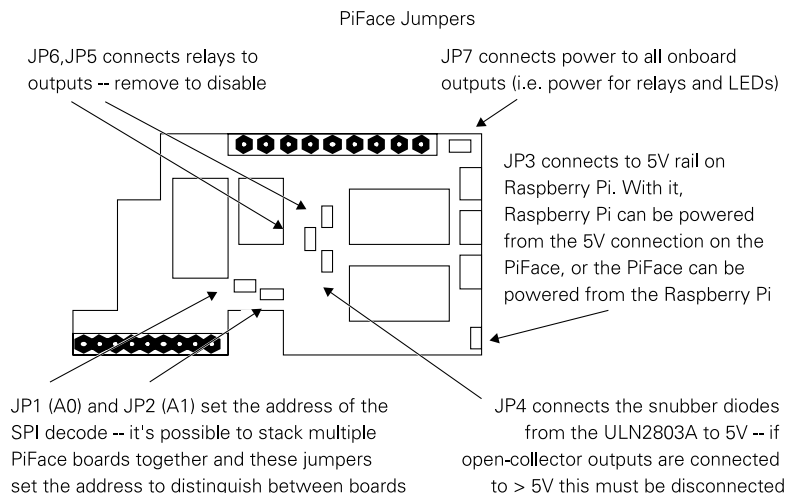
FIGURE 3-3: PiFace jumpers.
