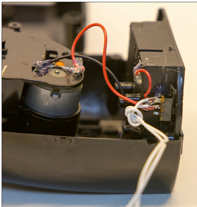
FIGURE 2-3: Add wires in parallel to the switch and add a knot to stop it from pulling through.
