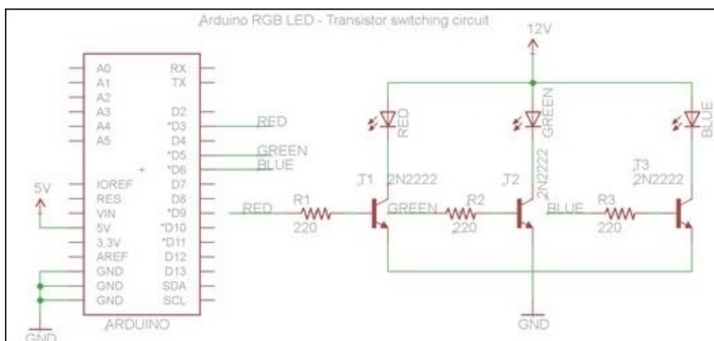
The Arduino RGB switching circuit
