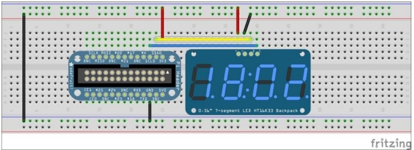
7-segment backpack connections on a breadboard
