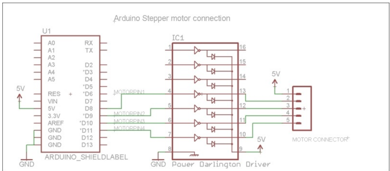
An Arduino stepper motor interface
