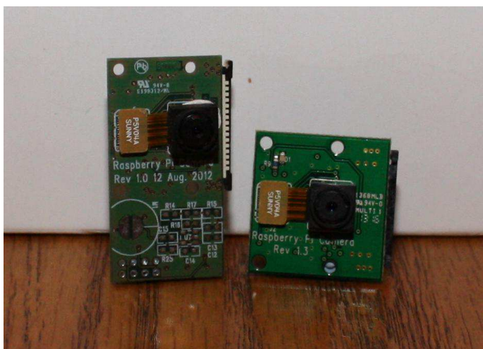
Prototype camera board (left) and final camera board (right)
