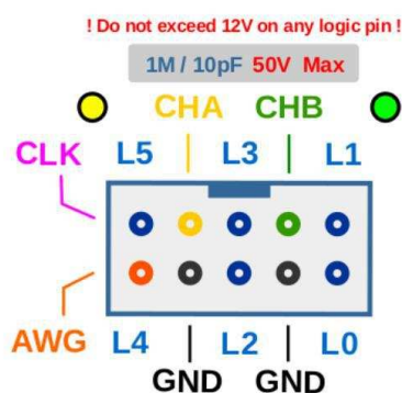
Figure 3: Pin layout of the BitScope Micro (photo courtesy by BitScope Designs)
