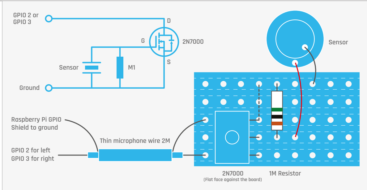
Fig 1 Schematic and physical layout of the sensors
