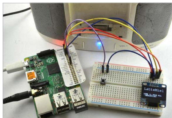
Above Your very own no-frills world radio
