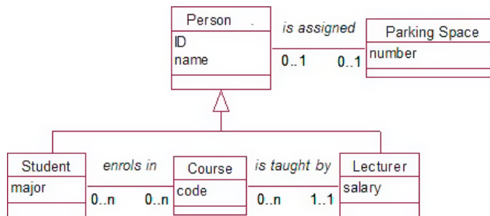
Figure 6-7. Common behavior captured in a superclass
