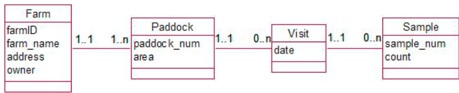
Figure 9-3. Several 1-Many ownership relationships
