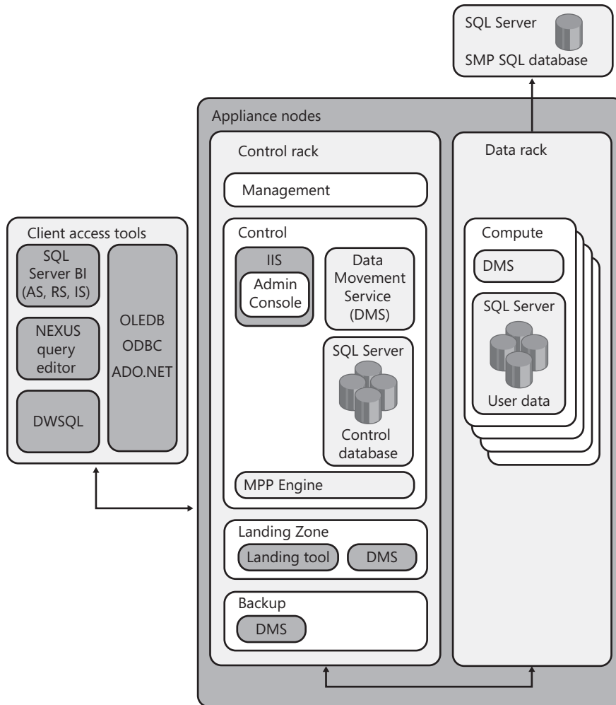
FIGURE 6-2 Appliance software
