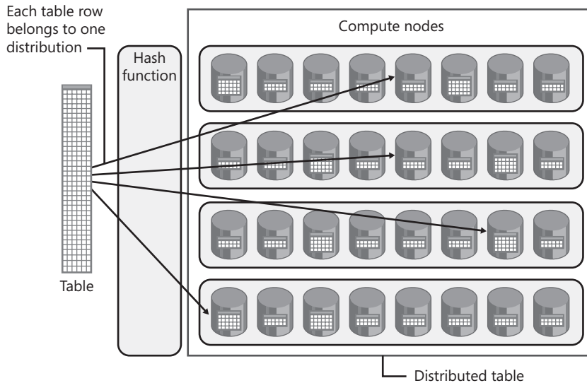
FIGURE 6-4 Distributed strategy
