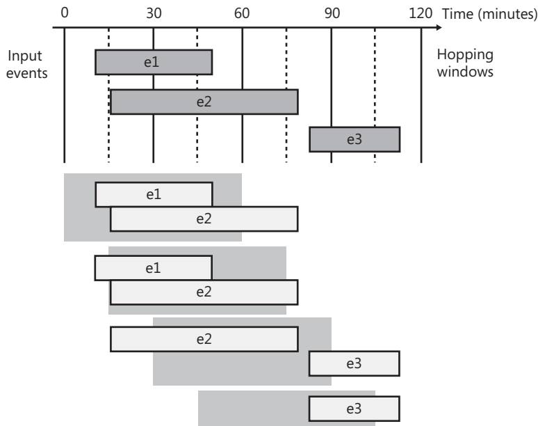
FIGURE 8-3 Hopping windows
