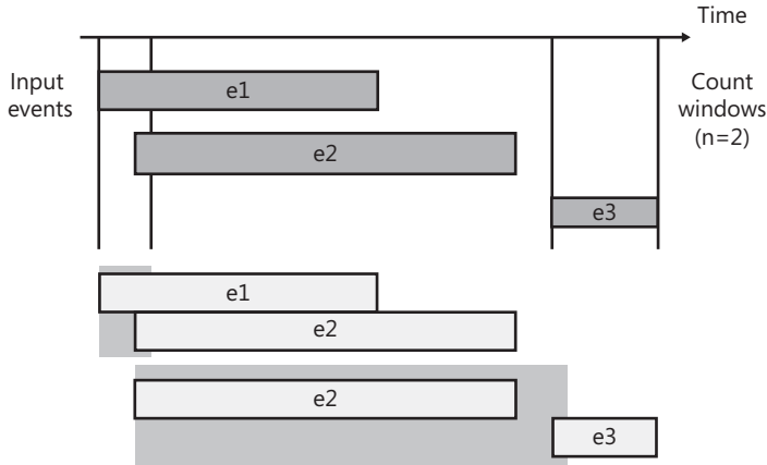
FIGURE 8-5 Count windows
