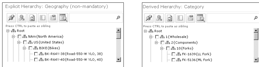
FIGURE 7-2 Product hierarchies
