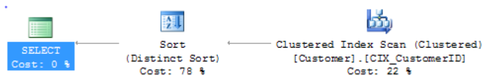
Figure 20 - Expensive sort plan during dimension processing
