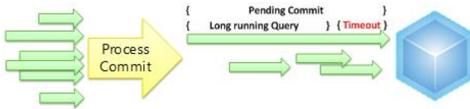
Figure 69 - Write locks blocking queries
