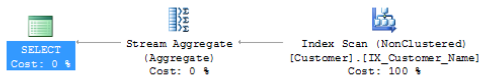
Figure 62 - A fast high cardinality attribute processing plan
