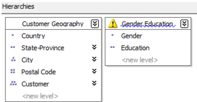
Figure 33: Natural and unnatural hierarchies
