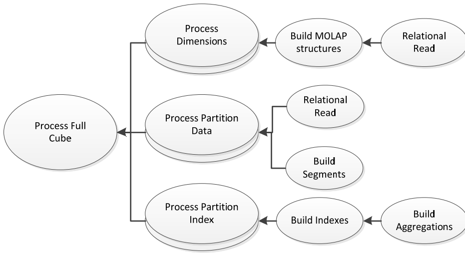
Figure 3030: Full cube processing overview
