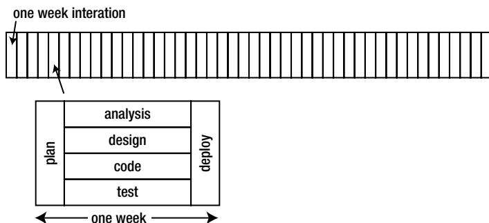
Figure 2-8. Agile project
