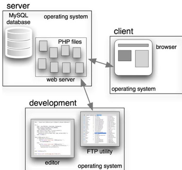
Figure 3-1. Client-server-development architecture
