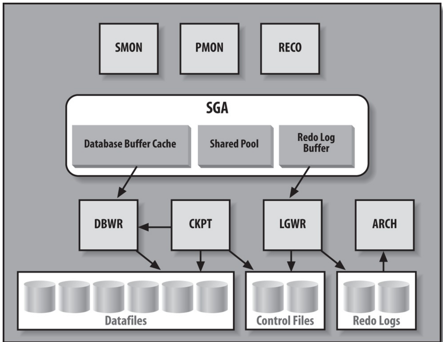
Figure 2-8. An Oracle instance
