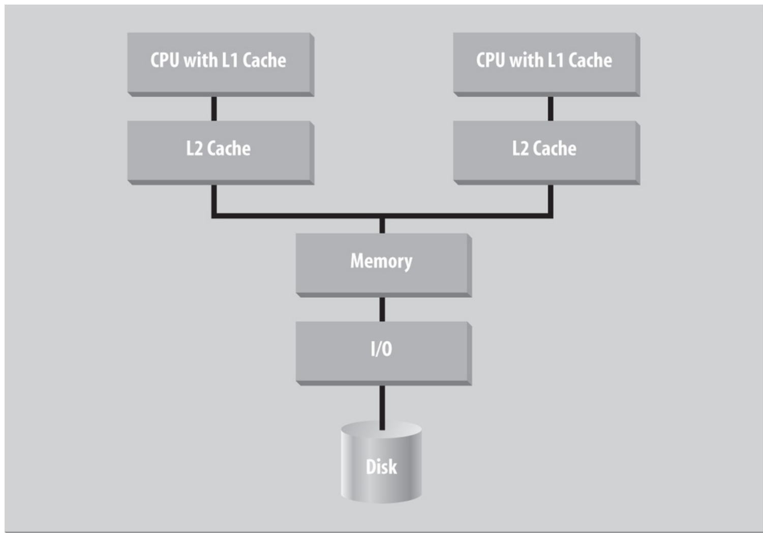
Figure 12-1. Typical Symmetric Multiprocessing (SMP) node
