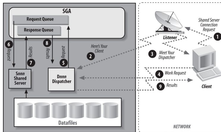
Figure 3-4. Connecting with the Oracle Net Listener (shared servers)
