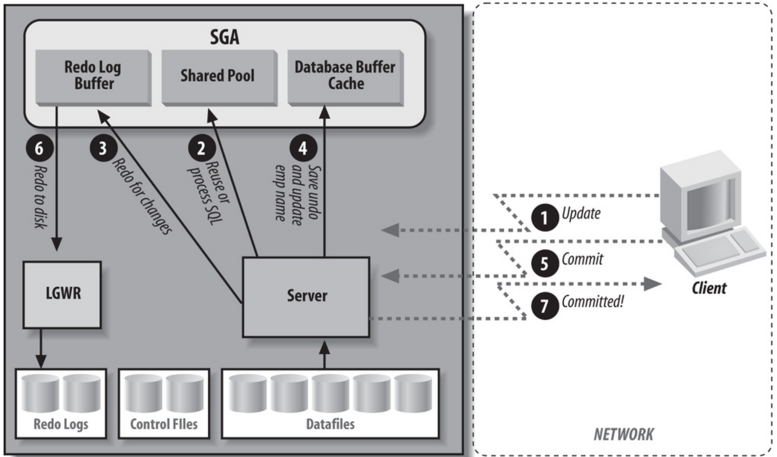
Figure 3-5. Steps for a transaction
