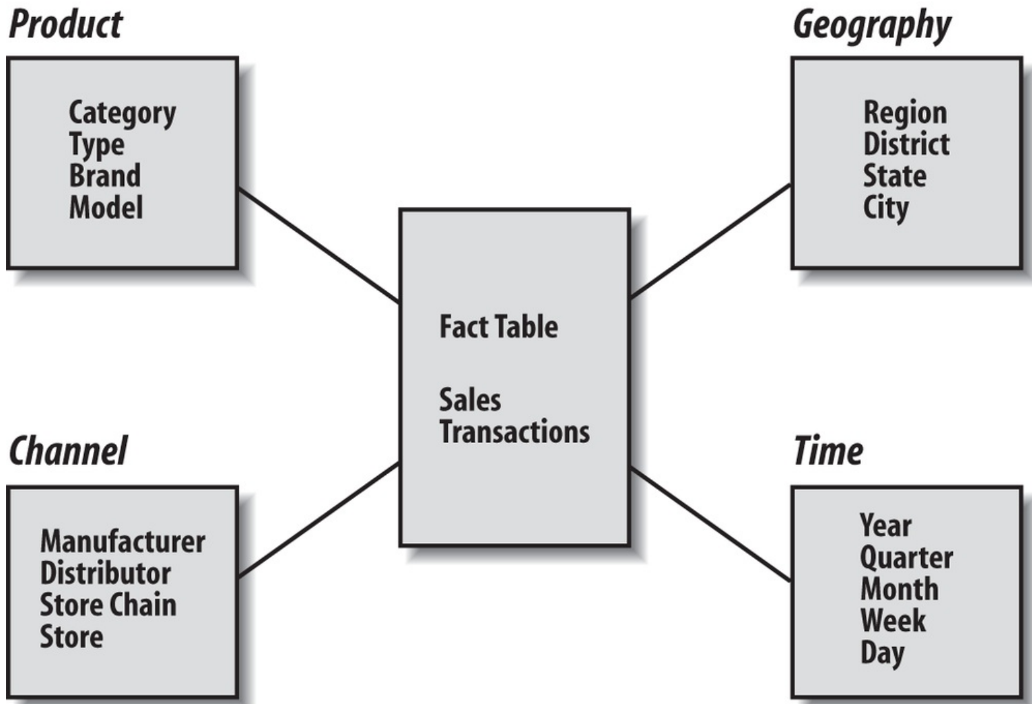
Figure 10-2. Typical star schema
