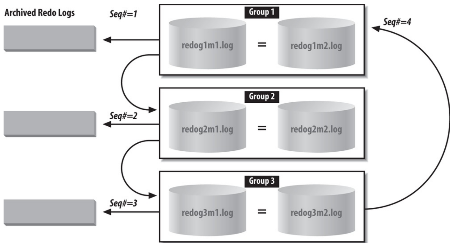
Figure 2-7. Cycling redo logs with archiving
