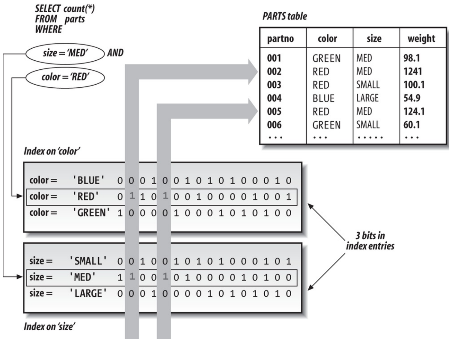
Figure 10-3. Bitmap index operation in a compound WHERE clause
