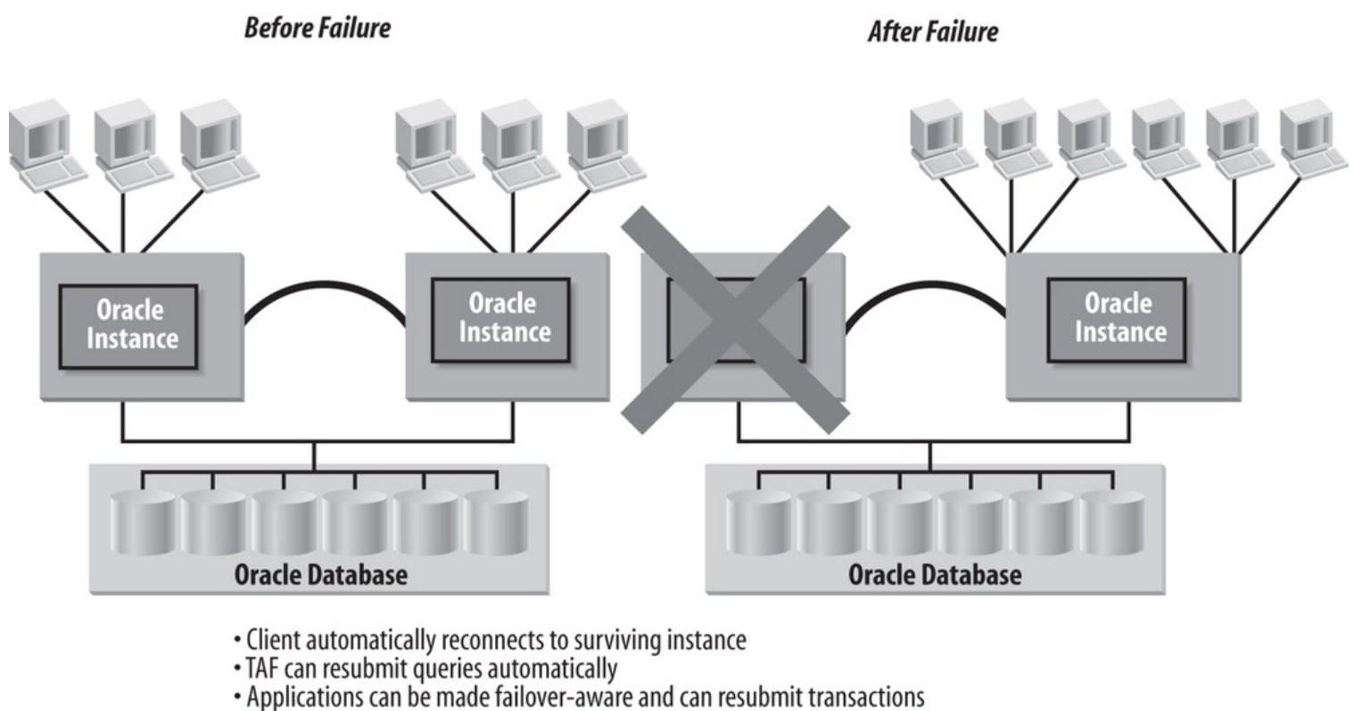
Figure 11-7. Failover with TAF and Real Application Clusters
