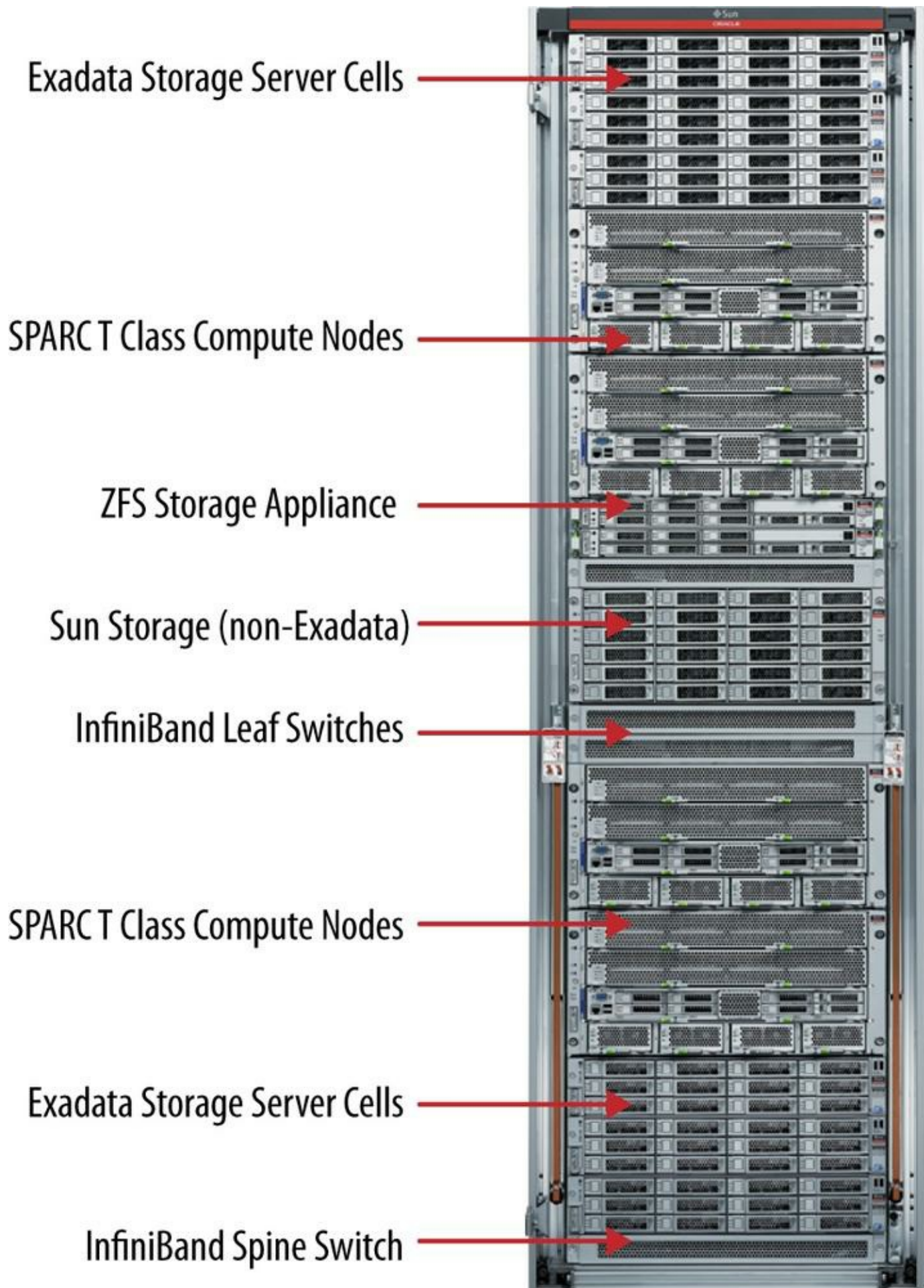
Figure 12-5. Oracle SuperCluster
