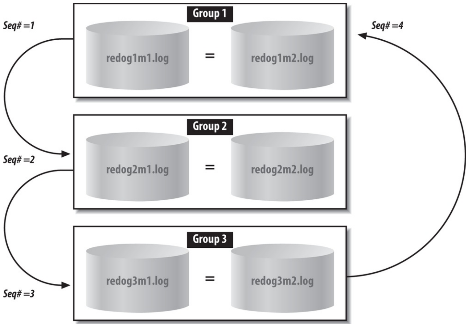
Figure 2-6. Cycling redo logs
