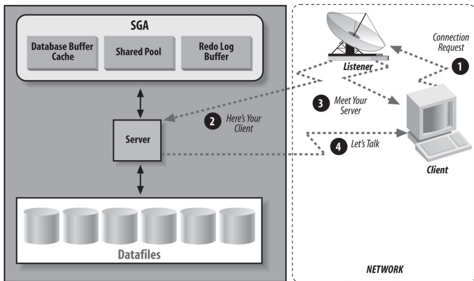
Figure 3-3. Connecting with the Oracle Net Listener
