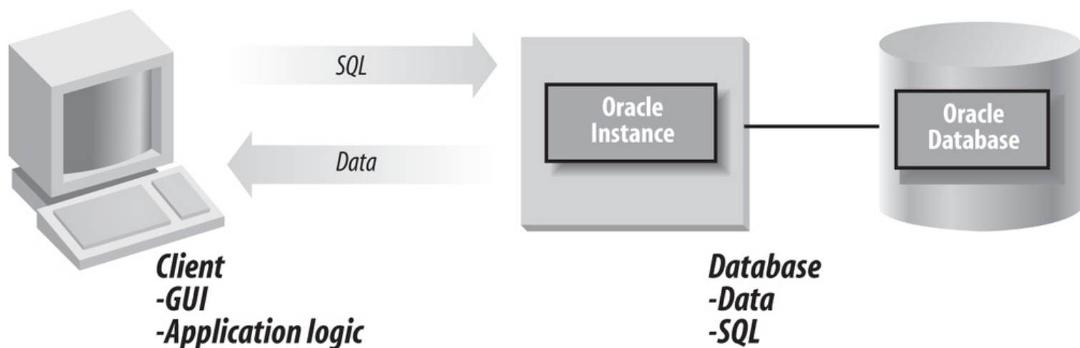
Figure 9-1. Two-tier client/server architecture
