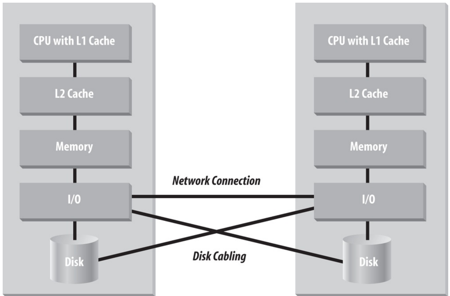
Figure 12-2. Typical cluster (two nodes shown)
