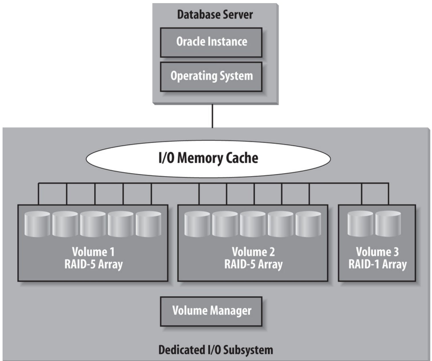
Figure 7-2. Dedicated I/O subsystems
