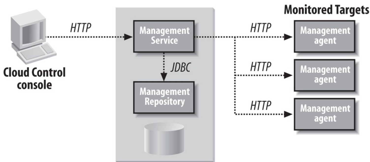
Figure 5-2. Oracle Enterprise Manager architecture
