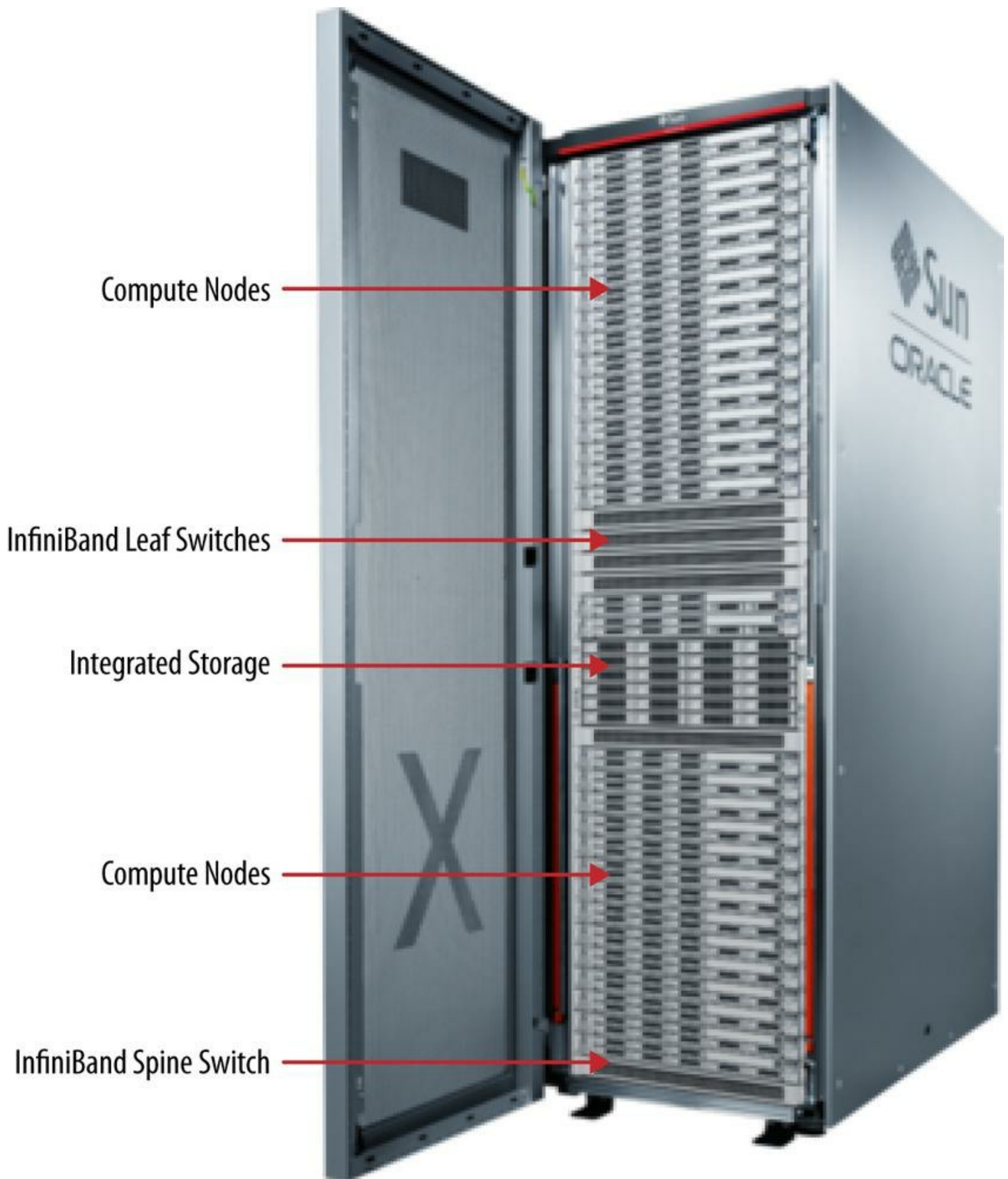
Figure 12-4. Oracle Exalogic
