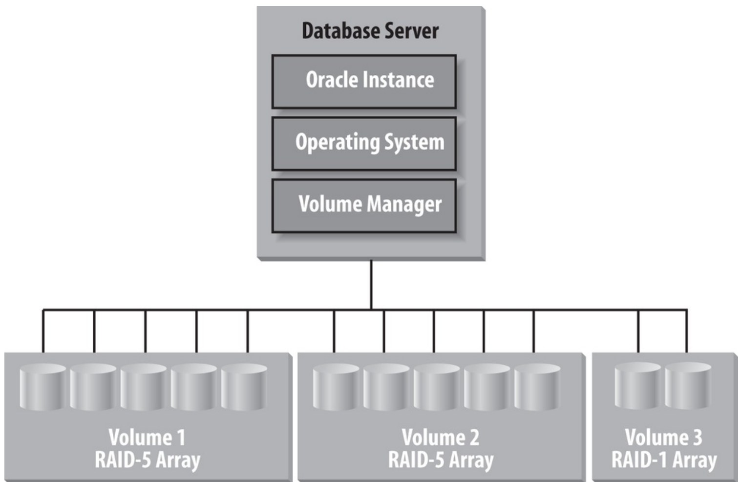
Figure 7-1. Host-based volume management
