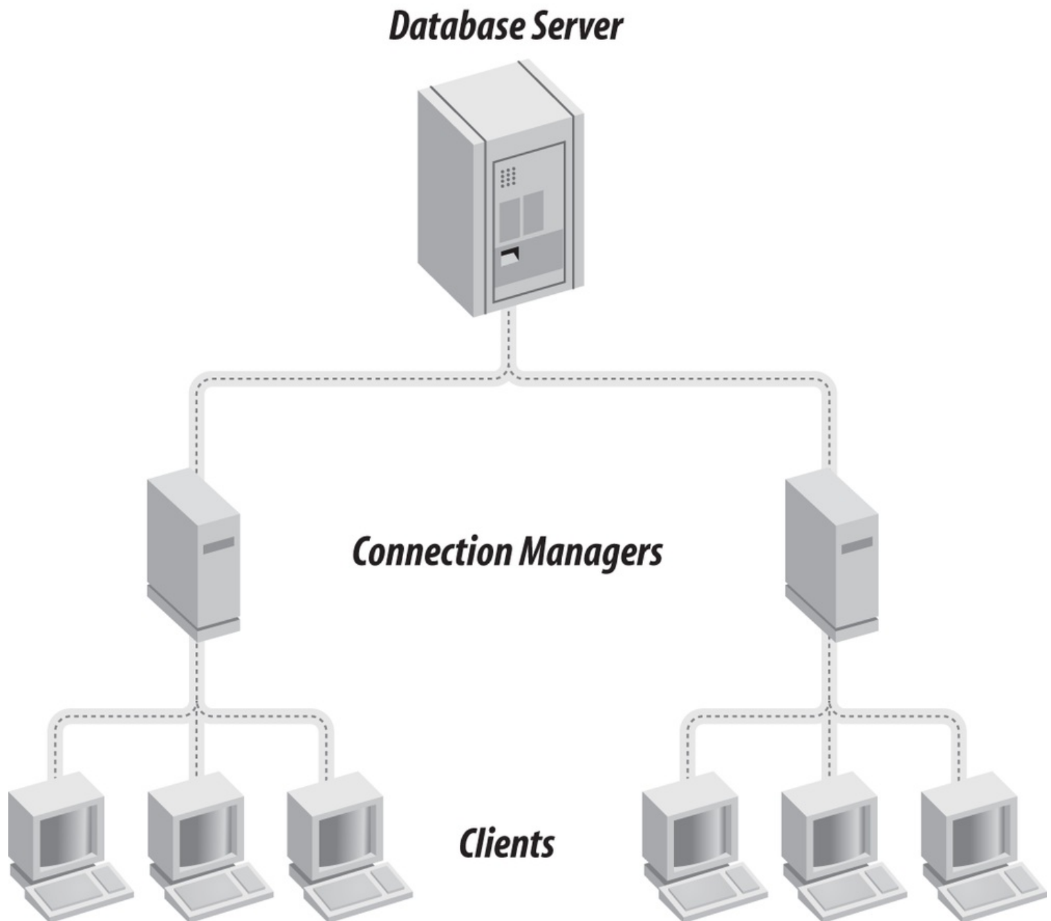
Figure 1-3. Concentrators with Connection Managers for a large number of users
