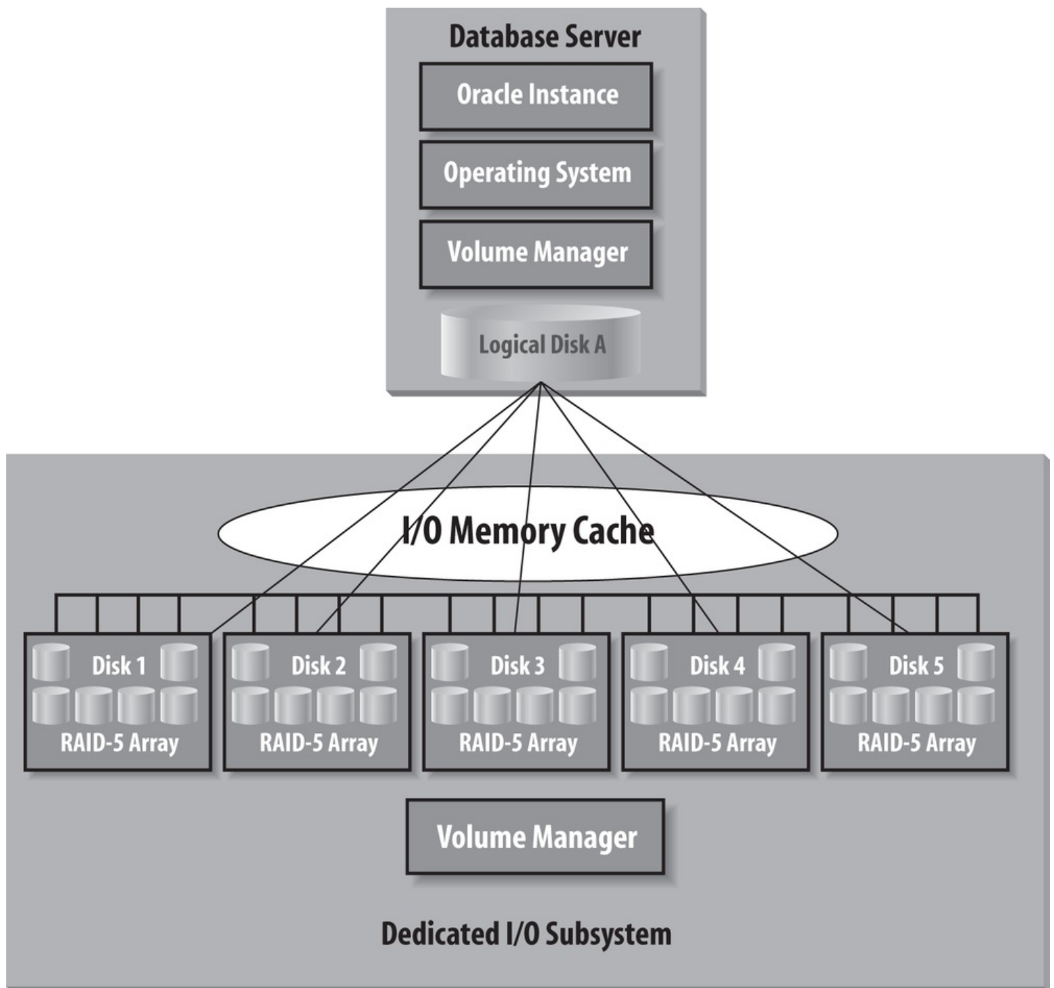
Figure 7-3. Dynamic block-range parallelism
