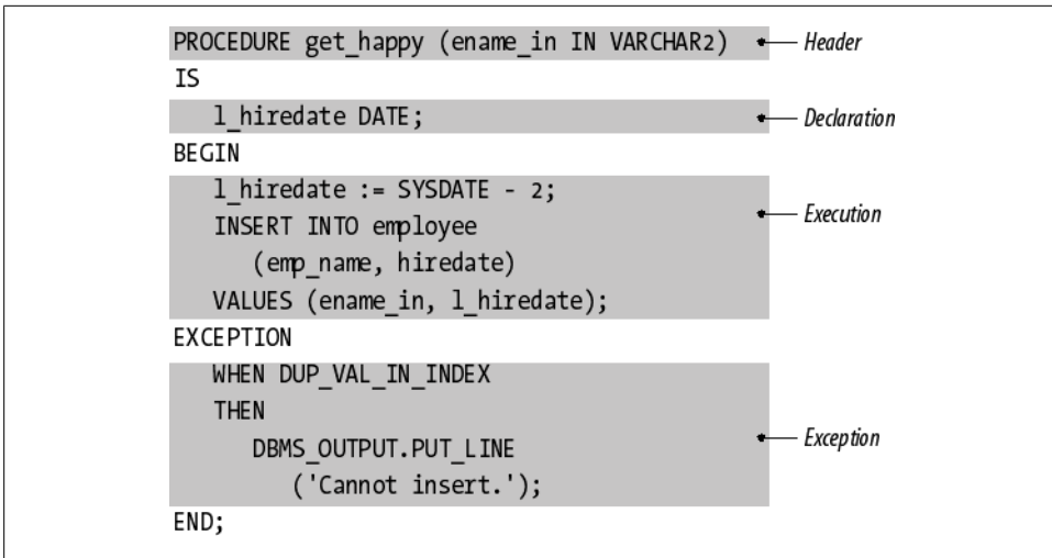
Figure 3-2. A procedure containing all four sections
