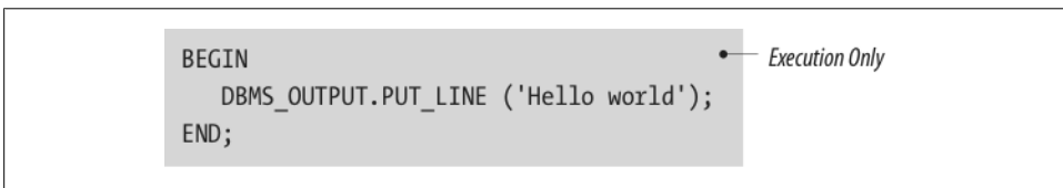
Figure 3-3. An anonymous block without declaration and exception sections
