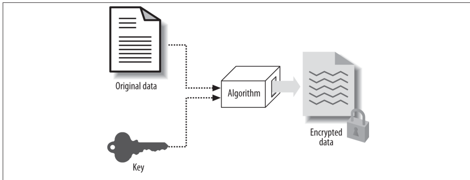
Figure 23-1. Encryption basics
