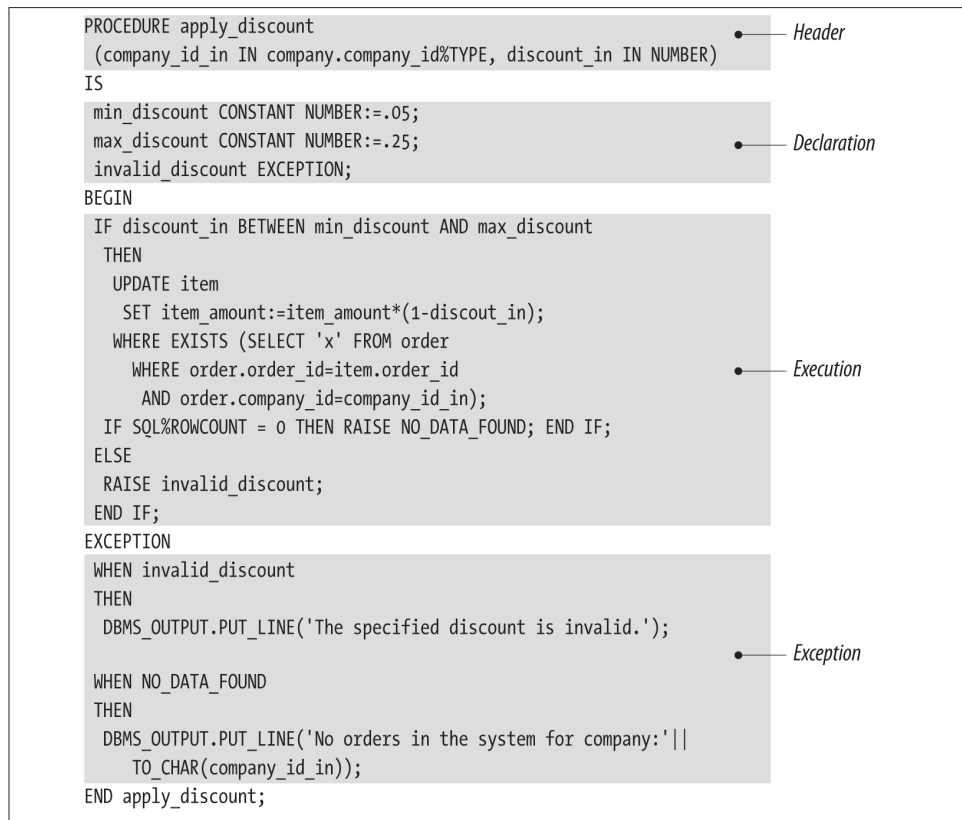
Figure 17-1. The apply_discount procedure
