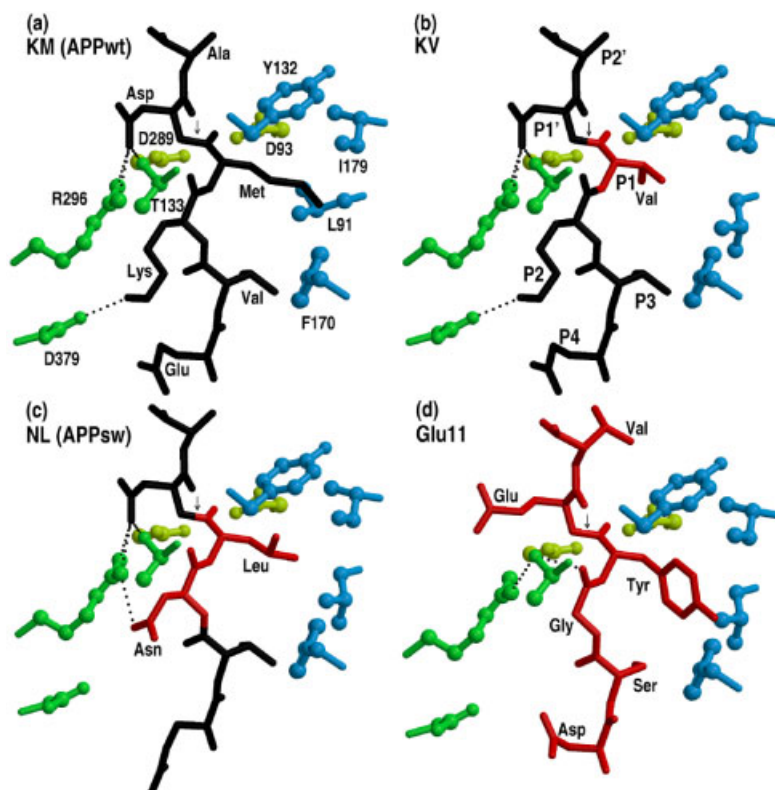
Fig. 5.4 Models of \beta -secretase with APP-derived substrates. (A) Wild-type substrate residues 592–597 of APP (GenBank accession CAA312830.1) with sequence EVKM*DA (P4-P3-P2-P1-P1'-P2') with cleavage site marked with *. (B) Mutant substrate with Val (red) substitute for P1
