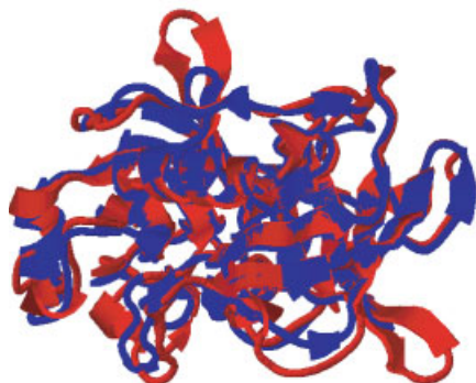
c) Superposition of the backbones of elastase (red) and trypsin (blue)
