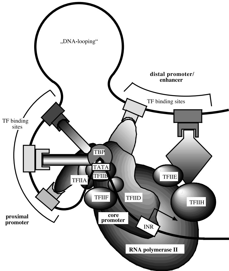
Fig. 4.3 Transcription initiation complex bound to a schematic promoter
