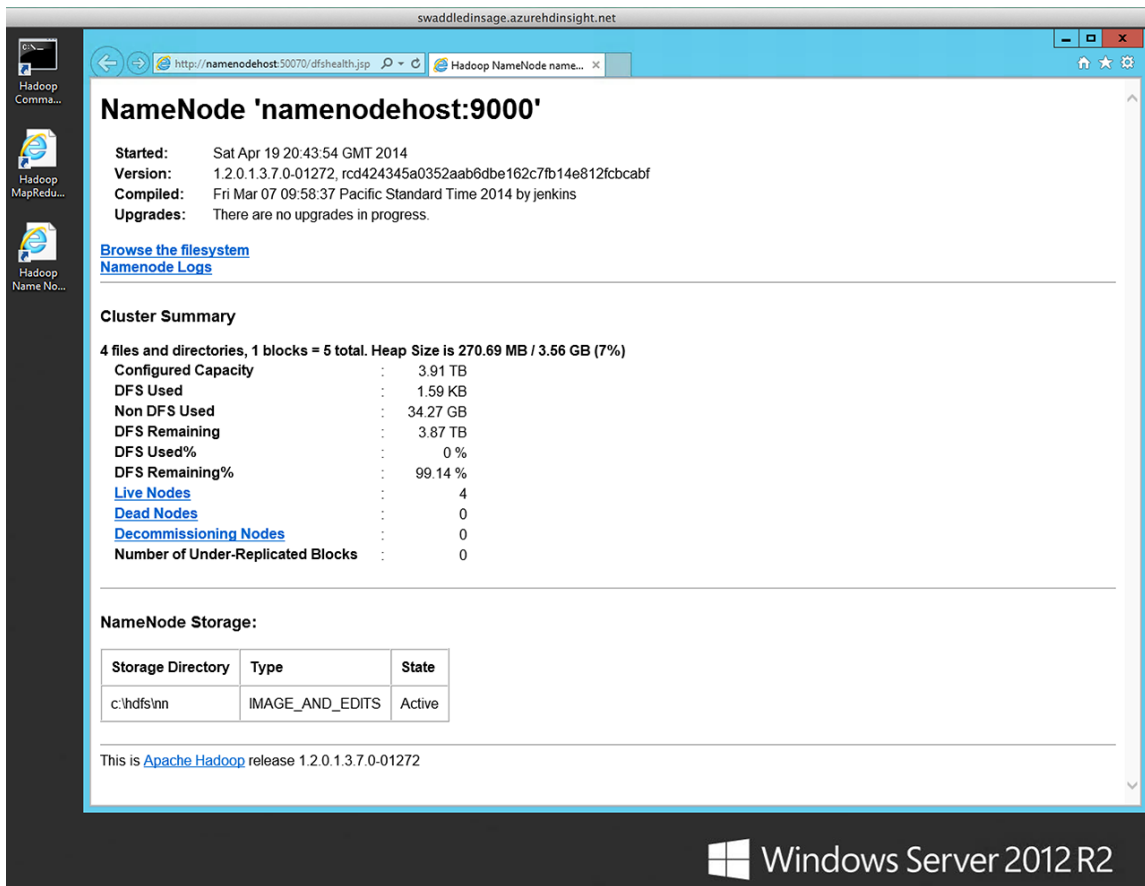
FIGURE 2-7 Hadoop name node status web service.
