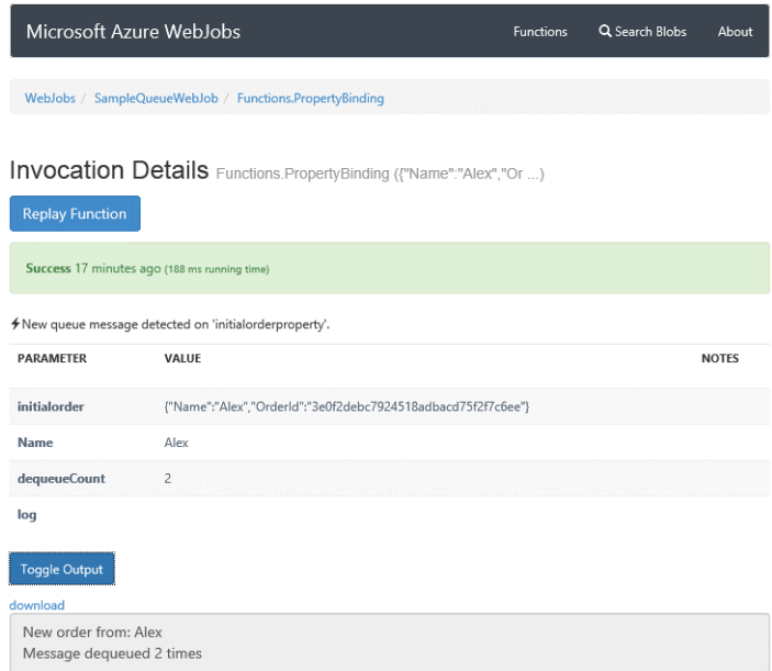
FIGURE 2-17 Invocation details for a web job function.
