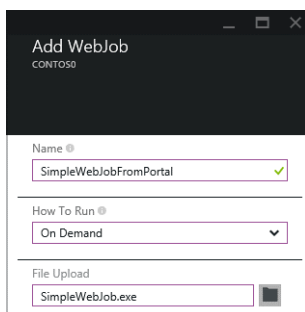
FIGURE 2-8 Add WebJob blade in the Azure portal.
