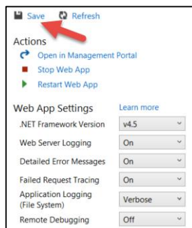
FIGURE 4-2 Application and site diagnostic log configuration in Visual Studio.
