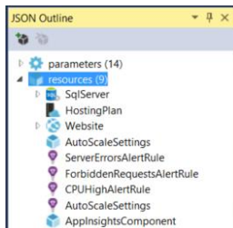
FIGURE 1-19 JSON Outline window showing resources from the resource group deployment template.
