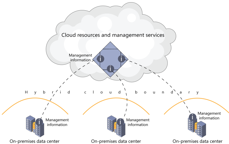
FIGURE 1-1 Three on-premises data centers exchange management information with cloud resources and management services across the hybrid cloud boundary.
