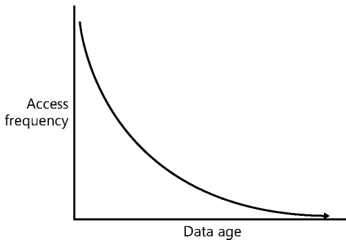
FIGURE 4-5 The typical data life cycle with access frequency as a function of data age.
