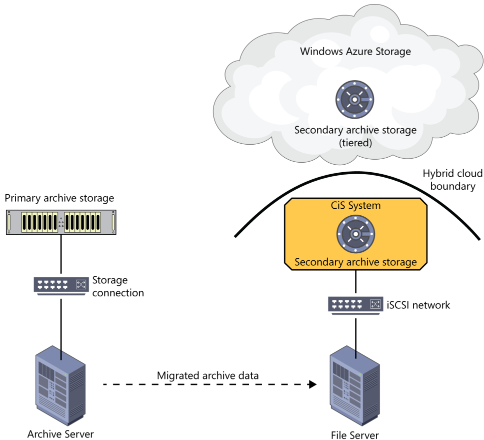
FIGURE 5-1 Archive data is migrated from primary archive storage connected to an archive server to a file server connected to Microsoft HCS.
