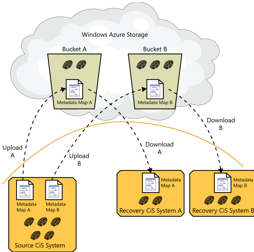
FIGURE 3-4 The process of parallel recovery from data stored in two Windows Azure Storage buckets to two different recovery CiS systems.
