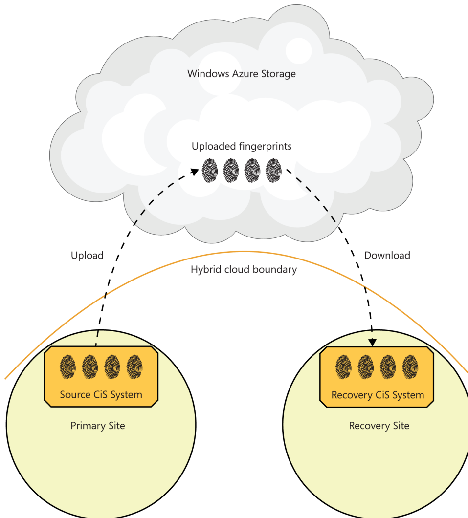
FIGURE 3-2 The data flow for recovering data with the Microsoft HCS solution.
