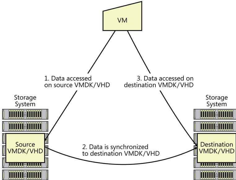
FIGURE 4-1 In storage migration, a VM moves its VHD from one storage system to another.
