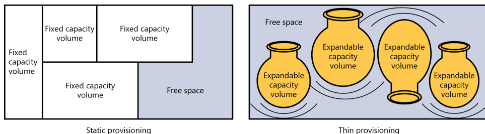
FIGURE 4-2 A comparison of static provisioning with thin provisioning.
