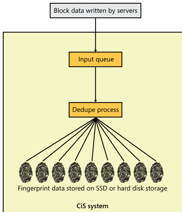
FIGURE 2-2 Block data is converted to fingerprints in the CiS system.
