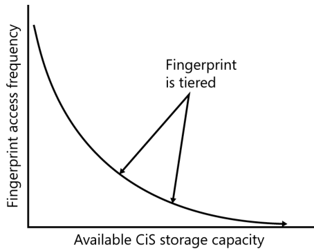
FIGURE 6-2 Fingerprints are tiered to cloud storage based on their access frequency and the available capacity in the CiS system.
