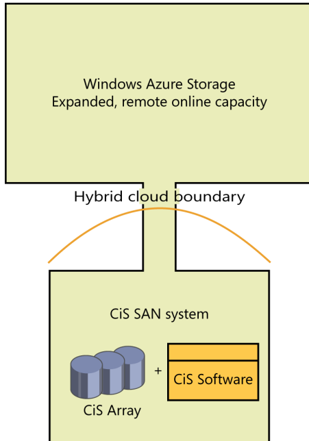
FIGURE 1-2 In the hybrid cloud storage architecture, the CiS SAN system accesses the expanded capacity available to it in Windows Azure Storage over an extended distance.
