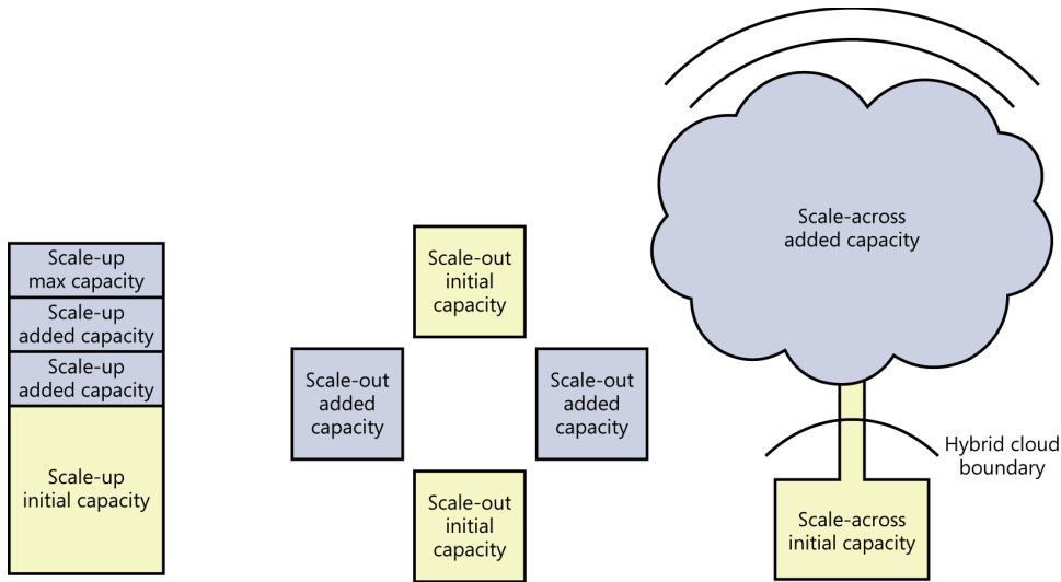
FIGURE 4-4 A comparison of storage scaling architectures.
