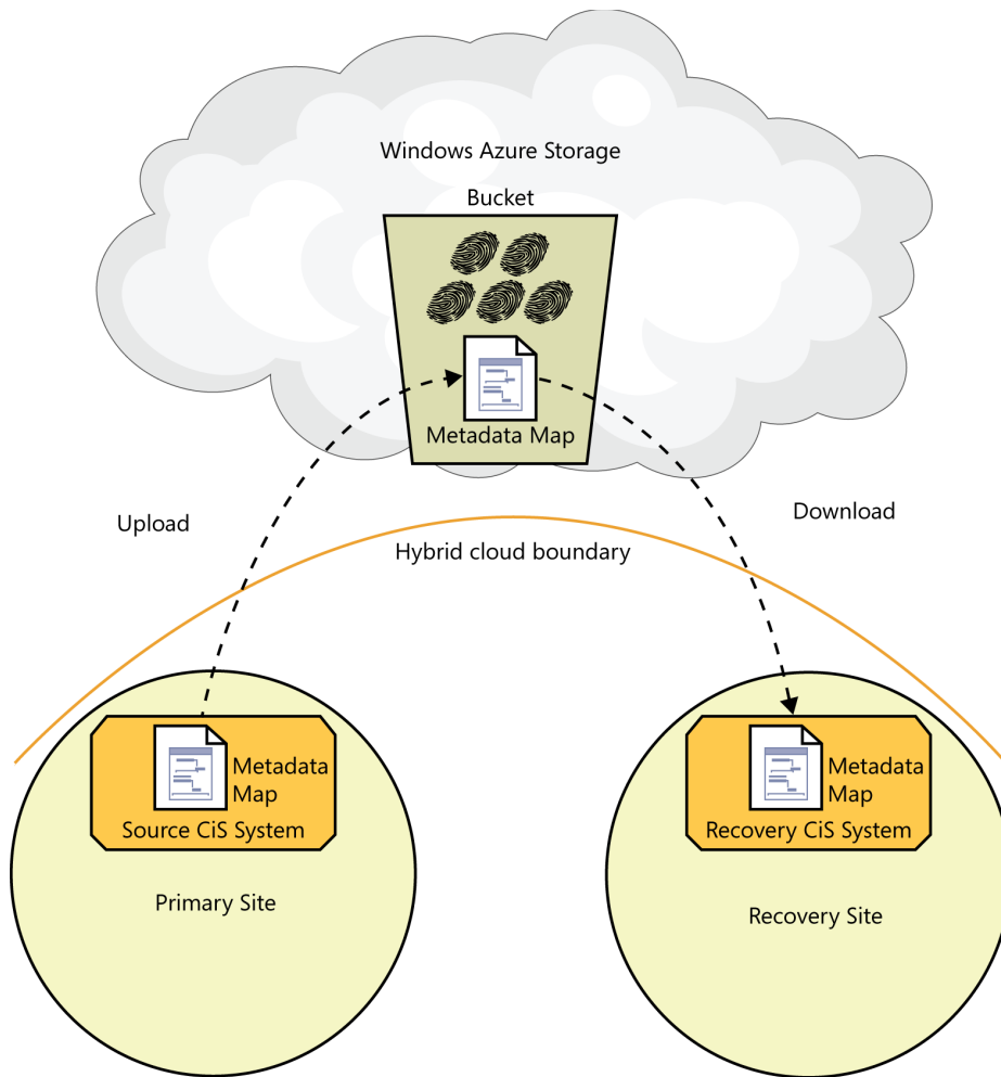
FIGURE 3-3 The metadata map that was uploaded by the source CiS system and stored in the Windows Azure Storage bucket is downloaded by the recovery CiS system.
