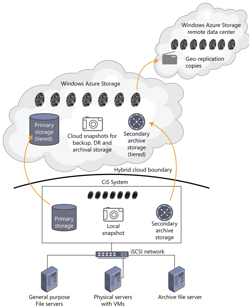
FIGURE 6-1 Servers access the Microsoft HCS solution through an iSCSI network. Primary storage, secondary archives storage and local snapshots are located on the CiS system. Cloud snapshots DR and tiered primary and secondary archive storage are located in Windows Azure Storage. The data on Windows Azure Storage is also stored in a remote Windows Azure data center through the use of geo-replication services in Windows Azure.
