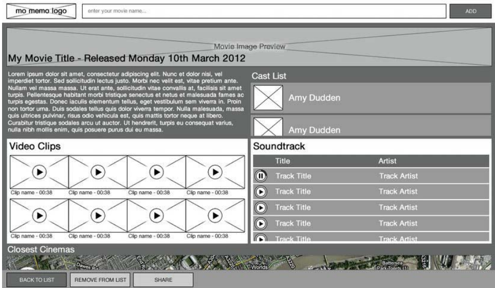
Figure 4-12. Movie info on a landscape tablet device
