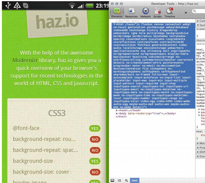
Figure 2-1. Using Modernizr to detect features on haz.io
