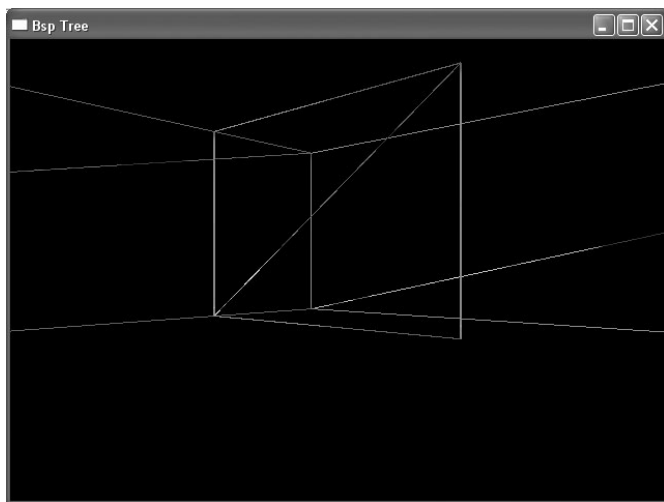
FIGURE 13.9 A screenshot from the BSP Tree demo.
