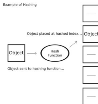
FIGURE 7.1 A hash table.
