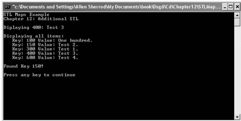
FIGURE 12.2 A Screenshot of the STL Map Demo.
