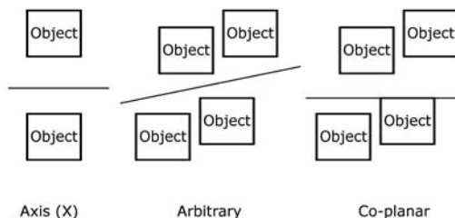
FIGURE 13.8 Splitting plane types.
