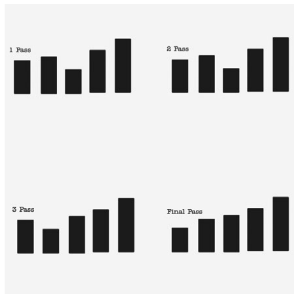
FIGURE 4.3 The array from Figure 4.2 after all bubble sort passes.
