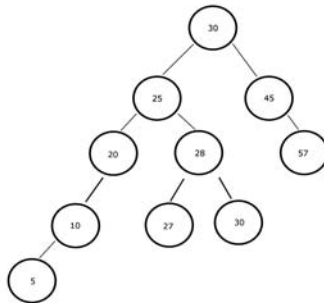
FIGURE 9.12 Replacing the node with its in-order successor leaves the tree valid.
