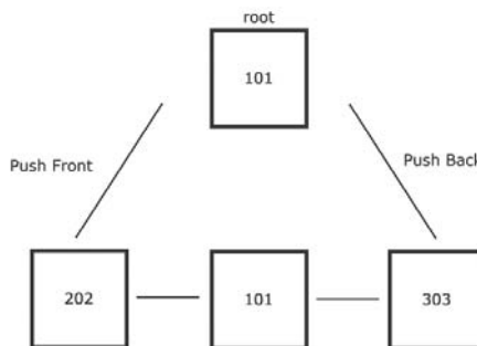
FIGURE 5.4 A double-ended link list.
