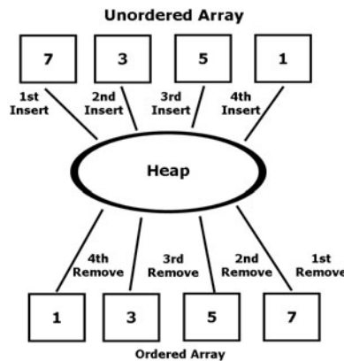
FIGURE 10.5 The heap sort.
