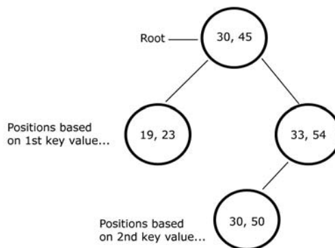
FIGURE 9.14 Nodes of a kd -tree.
