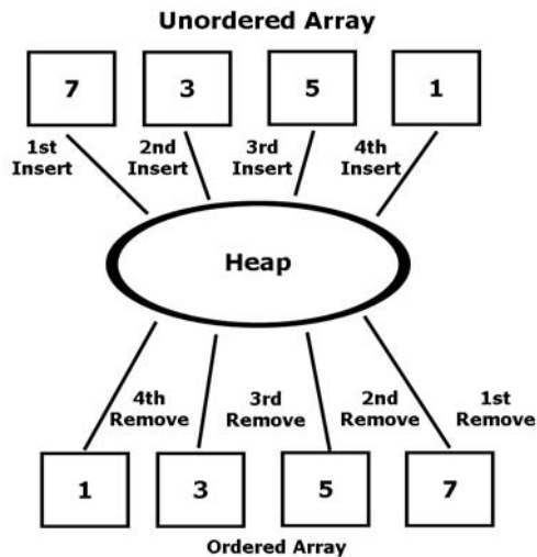
FIGURE 8.13 The heap sort.
