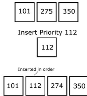
FIGURE 6.8 A priority queue.
