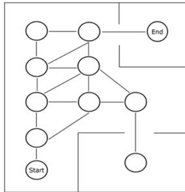
FIGURE 11.15 An overhead view of a game world where vertices define how to get from one area to another.
