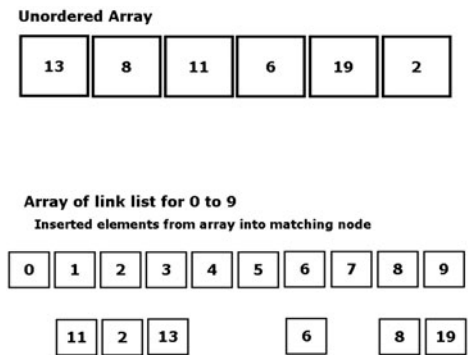
FIGURE 8.10 Sorting the ones position.
