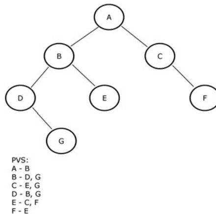
FIGURE 13.17 A BSP tree where each node knows which other nodes it can see.
