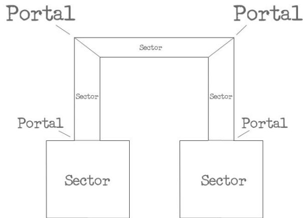
FIGURE 13.19 A scene divided by portals and sectors.
