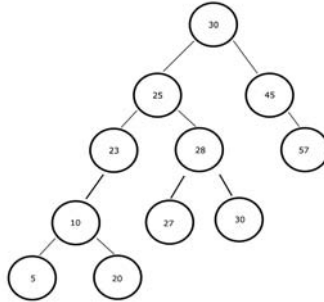
FIGURE 9.11 Simply deleting a node will lead to an invalid tree.
