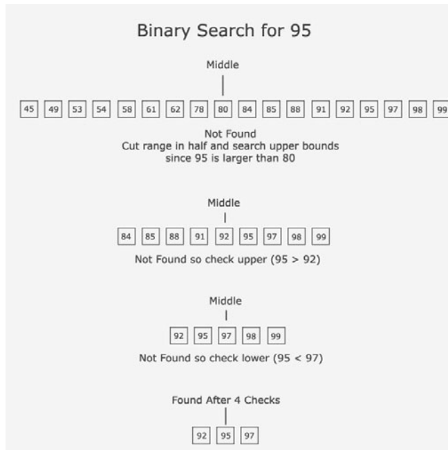
FIGURE 2.4 A binary search.
