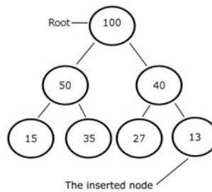
FIGURE 10.2 Inserting into a heap.
