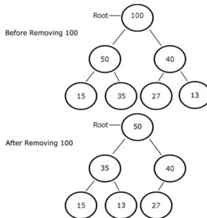
FIGURE 10.3 Removing from a heap.
