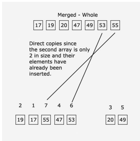
FIGURE 4.12 Merging arrays of different sizes.
