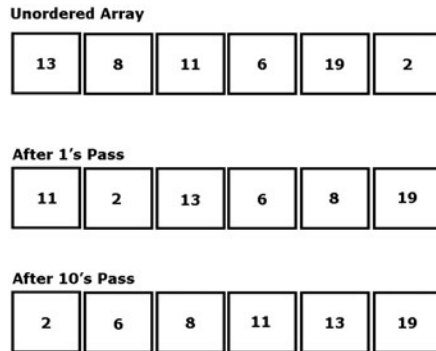
FIGURE 8.11 Sorting using the radix sort for six elements.
