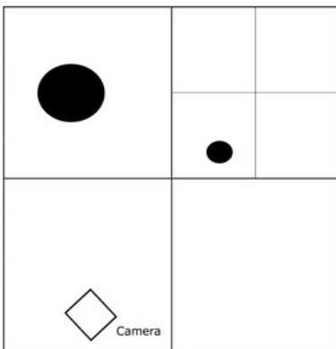
FIGURE 13.11 Building a quad tree out of a few objects.
