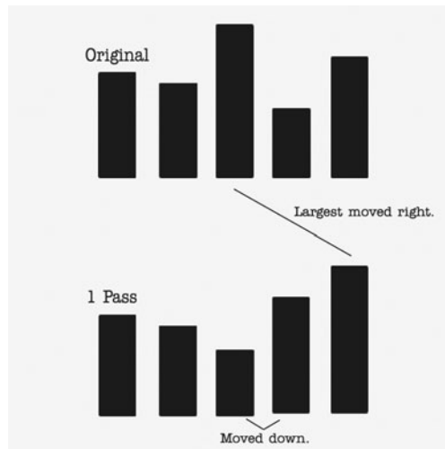
FIGURE 4.2 One pass over an array using the bubble sort.
