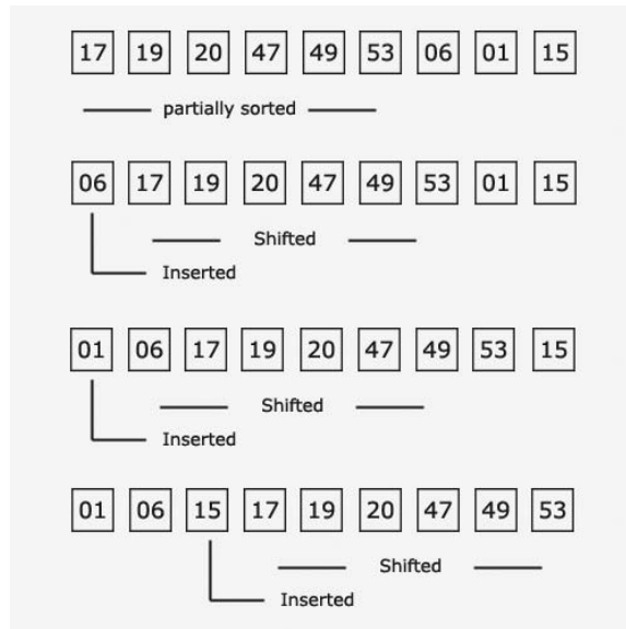
FIGURE 4.7 The insertion sort.
