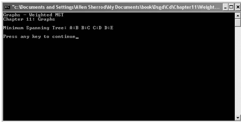
FIGURE 11.14 A screenshot of the Weighted MST demo.
