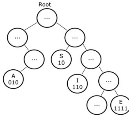
FIGURE 14.5 A binary tree for “Susie sells sea shells at the sea shore.”
