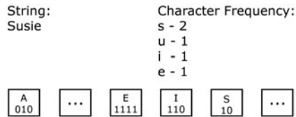
FIGURE 14.4 Removing two nodes, combining them, and placing them back on the queue.
