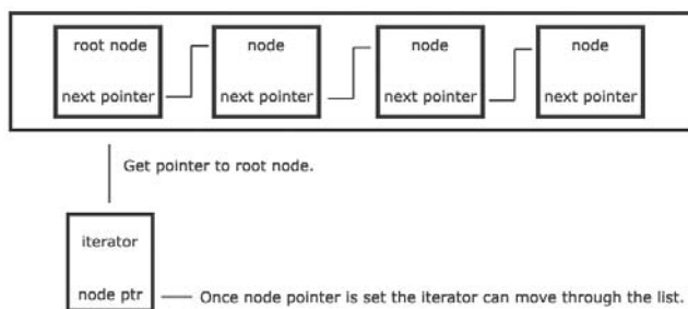
FIGURE 5.2 A visual representation of iterators.
