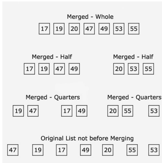
FIGURE 4.11 Merging until we have a sorted list.
