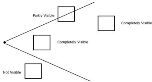
FIGURE 13.4 A frustum where some objects are outside, some inside, and others spanning.
