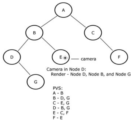
FIGURE 13.18 Using potential visibility sets.
