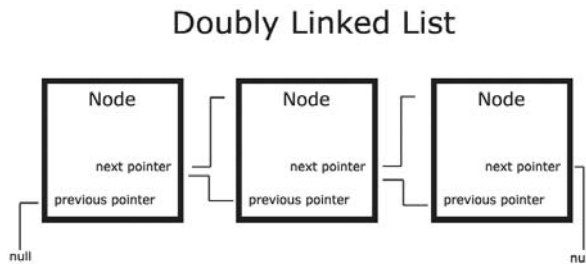
FIGURE 5.6 Visual representation of a doubly linked list.
