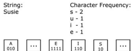
FIGURE 14.6 A Huffman table.
