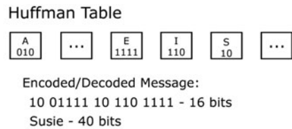
FIGURE 14.7 Compressing and decompressing using the Huffman code.
