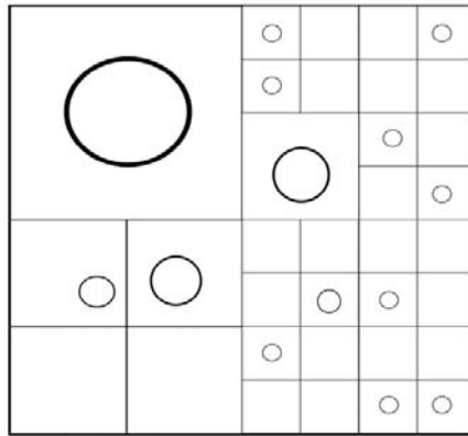
FIGURE 13.10 A quad tree.
