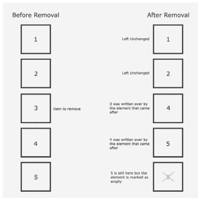
FIGURE 2.1 Removing an item from an array by copying over it.
