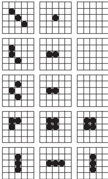
Some triplet histories in the Game of Life
