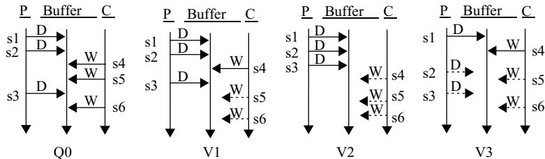
Figure 7.15 Sequence Q0 and its variants.
