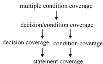
Figure 7.3 Hierarchy of sequential, structural coverage criteria based on the subsumes relation.
