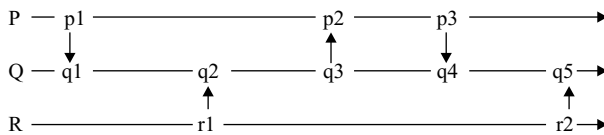
Figure 6.28 A distributed computation.
