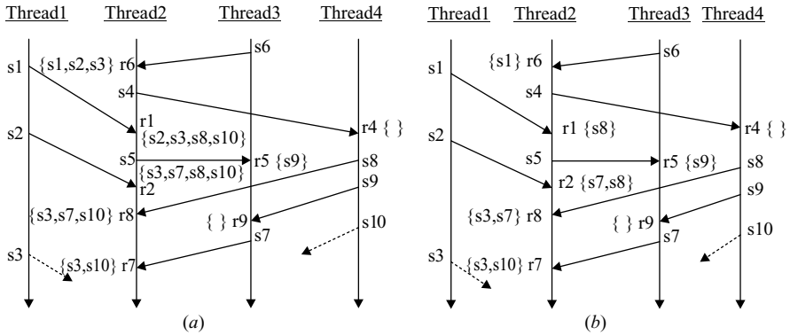
Figure 7.24 Race sets for SR-sequences.
