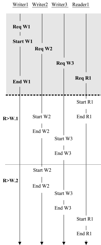
Figure 3.10 Comparing strategies R > W.1 and R > W.2 .
