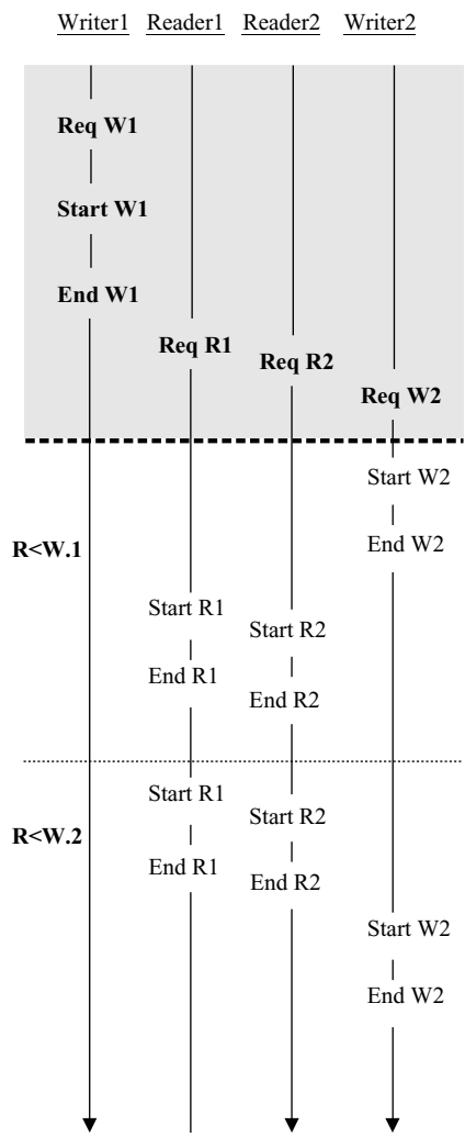
Figure 3.9 Comparing strategies R < W.1 and R < W.2 .
