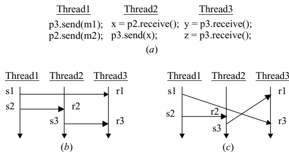
Figure 5.19 Execution trace and a variant for asynchronous ports with FIFO synchronization.
