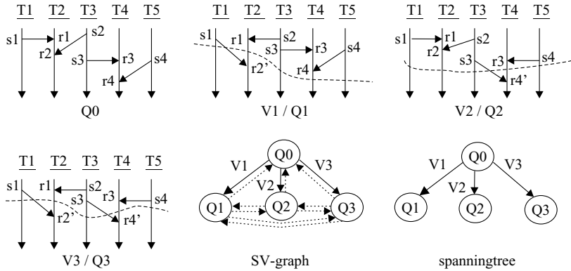
Figure 7.31 Illustrating constraint C2.
