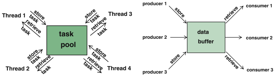
Fig. 3.6 Illustration of a task pool ( left ) and a producer–consumer model ( right )
