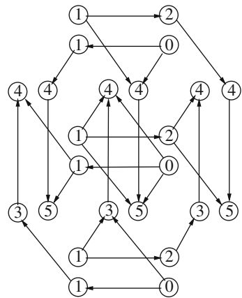
Fig. 2.21 3 × 3 mesh and corresponding channel dependence graph for XY routing
