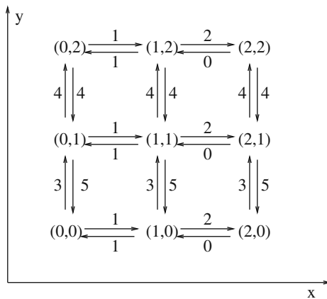
Fig. 2.21 3 × 3 mesh and corresponding channel dependence graph for XY routing
