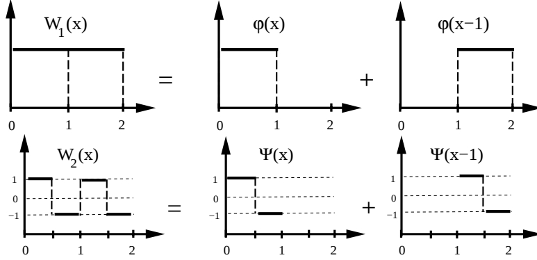
Figure 3.24: The first Walsh basis function (upper) is expressed in terms of the Haar scaling function. The second Walsh basis function (lower) is expressed in terms of the Haar wavelet.
