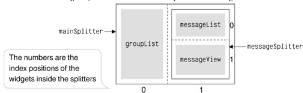
Figure 9.6. The News Reader's Splitters and Widgets
