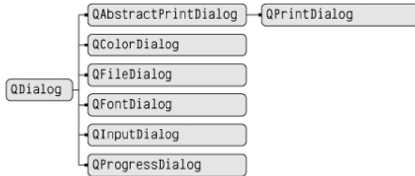
Figure C.5. Selected Classes from the QDialog Hierarchy
