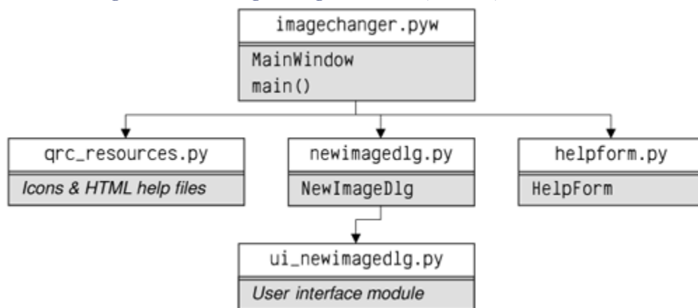
Figure 6.2. The Image Changer's Modules, Classes, and Functions
