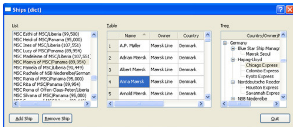
Figure 14.2. QListWidget, QTableWidget, and QTreeWidget in Action
