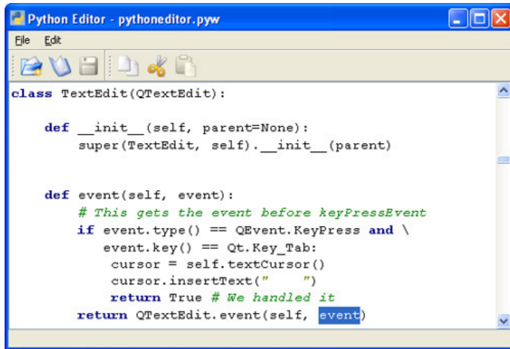
Figure 13.1. The Python Editor Editing Itself
