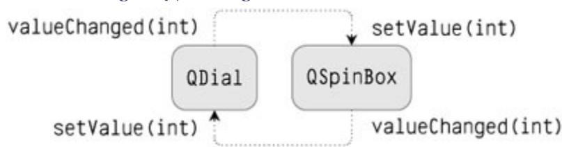
Figure 4.7. The Signals and Slots Connections
