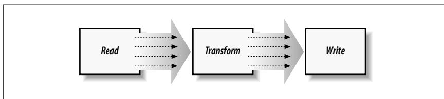
Figure 2-3. Simple SAX2 event pipeline
