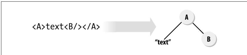
Figure 1-2. An object tree parser API
