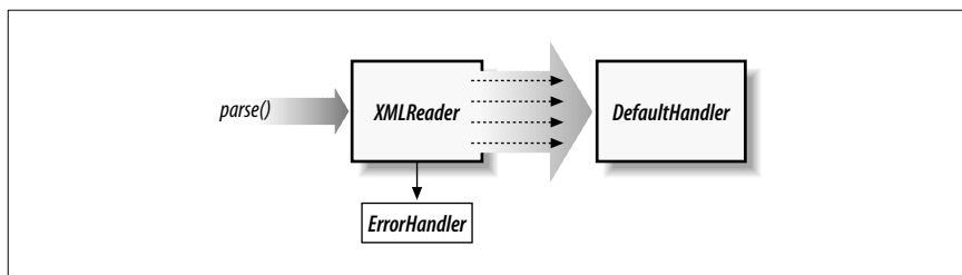
Figure 2-2. Basic SAX roles and components
