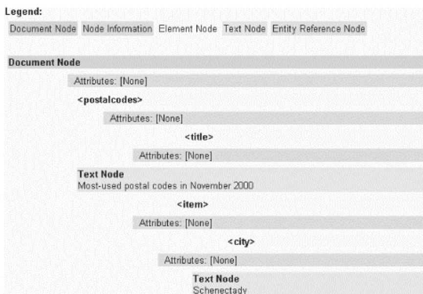
Figure 1-2. DOM tree representation of an XML document
