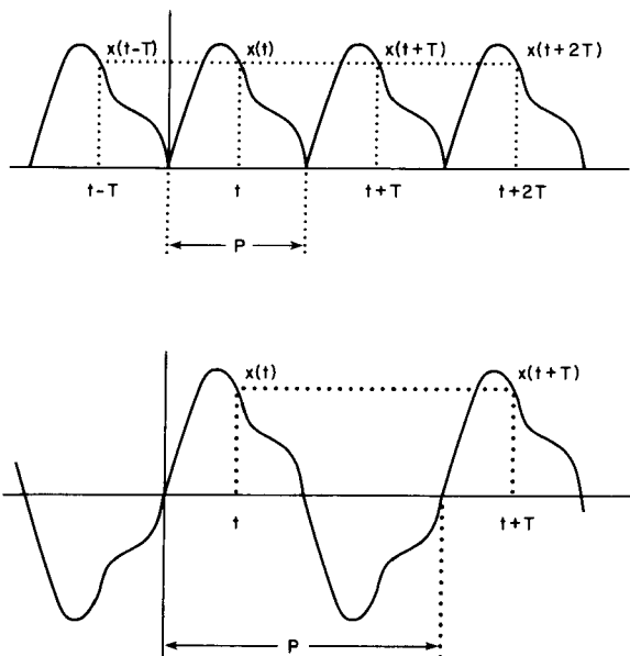
Figure 1.7 Periodic functions.
