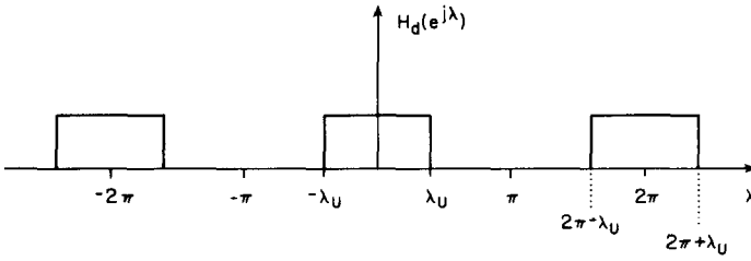
Figure 11.4 Frequency response of ideal lowpass digital filter.
