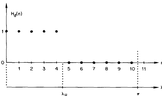
Figure 12.1 Desired discrete-frequency magnitude response for a lowpass filter with \lambda_U = 3\pi/7 .
