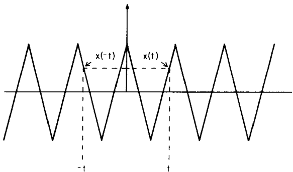
Figure 1.8 Even-symmetric function.
