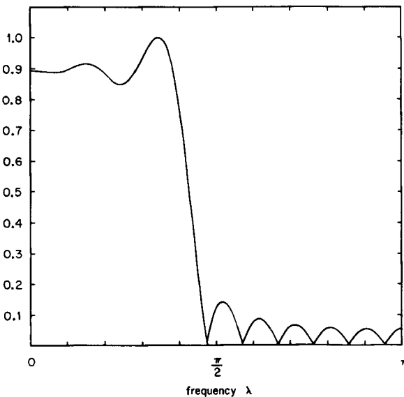
Figure 12.2 Magnitude response for filter of Example 12.1.
