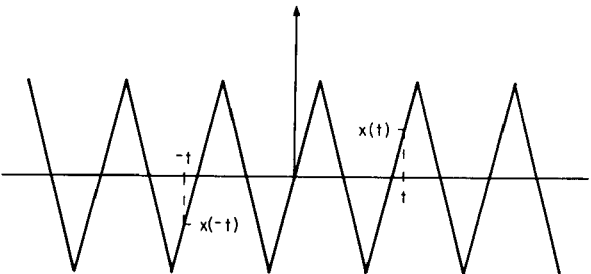
Figure 1.9 Odd-symmetric function.
