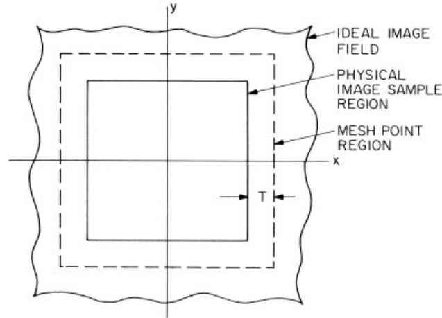
FIGURE 7.2-2. Relationship between regions of physical samples and mesh points for numerical representation of a superposition integral.
