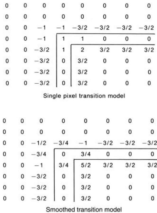
FIGURE 15.3-1. Separable eight-neighbor Laplacian responses for ramp corner models; all values should be scaled by h/8 .
