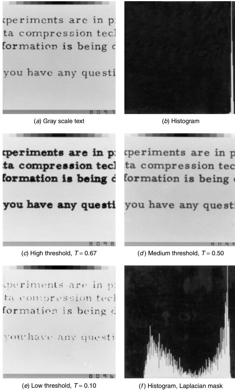
FIGURE 17.1-1. Luminance thresholding segmentation of typewritten text.
