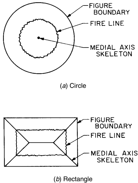
FIGURE 14.3-6. Medial axis transforms.
